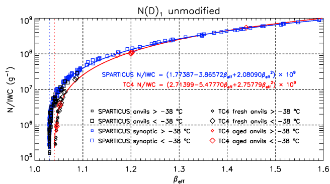
Figure 2. Dependence of N/IWC ( g^{-1} ) on the effective absorption optical depth ratio \beta_{\text{eff}} as predicted from the method of Parol et al. (1991), based on PSDs from SPARTICUS synoptic cirrus (blue squares) and anvils (black squares), and TC4 aged (red diamonds) and fresh (black diamonds) anvils, where the first size bin is included. The larger (smaller) symbols denote PSDs measured at a temperature colder (warmer) than -38 °C. The curve-fit equations are for SPARTICUS synoptic cirrus (blue) and for TC4 aged and fresh anvils (red).
