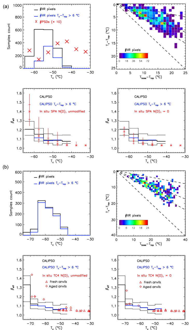
Figure 6. (a) Statistical comparison of CALIPSO IIR \beta_{eff} and in situ \beta_{eff} (synoptic cirrus) during SPARTICUS (sampled January–April 2010). Top left: the red X symbols indicate the number of PSDs used in the SPARTICUS analysis (multiplied by 10 for clarity of presentation) within 5^\circ\text{C} in situ temperature intervals, while the black histogram indicates the number of CALIPSO IIR pixels in each T_c temperature interval, and the blue histogram indicates the number of IIR pixels where T_c - T_{top} is larger than 6^\circ\text{C} . Top right: 2D-histograms of T_c - T_{top} and T_{base} - T_{top} for the IIR pixels. The dashed lines from top to bottom are 20%, 43% (average value) and 60% from cloud top, with T_c = T_{base} for the lowest curve. Bottom: temperature dependence of in situ \beta_{eff} derived assuming N(D)_1 unmodified (left) and N(D)_1 = 0 (right). The vertical lines give the measurement range, the horizontal bars give the 25th and 75th percentile values, and the asterisks give the median value. CALIPSO IIR median \beta_{eff} is given by the thick black histogram, with thin black histograms giving the 25th and 75th percentile values. The thick blue histogram is CALIPSO IIR median \beta_{eff} where T_c - T_{top} > 6^\circ\text{C} . (b) Statistical comparison of CALIPSO IIR \beta_{eff} and in situ \beta_{eff} during TC4. Top left: the black histogram indicates the number of CALIPSO IIR pixels in each T_c temperature interval, and the blue histogram indicates the number of IIR pixels where T_c - T_{top} is larger than 6^\circ\text{C} . Top right: 2D-histograms of T_c - T_{top} and T_{base} - T_{top} for the IIR pixels. The dashed lines from top to bottom are 20%, 43% and 60% from cloud top, for comparison with SPARTICUS data, with T_c = T_{base} for the lowest curve. Bottom: temperature dependence of in situ \beta_{eff} derived assuming N(D)_1 unmodified (left) and N(D)_1 = 0 (right) for fresh (red triangles) and aged (red diamonds) anvils. CALIPSO IIR median \beta_{eff} is given by the thick black histogram, with thin black histograms giving the 25th and 75th percentile values. The thick blue histogram is CALIPSO IIR median \beta_{eff} where T_c - T_{top} > 6^\circ\text{C} .
