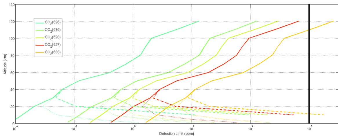
Fig. 23 Detection limits \text{CO}_2 and its main isotopologues for several dust loadings, here expressed as aerosol optical depth: solid: \text{AOD} = 0.0 , dotted: \text{AOD} = 0.1 , and dash-dotted: \text{AOD} = 1.0
