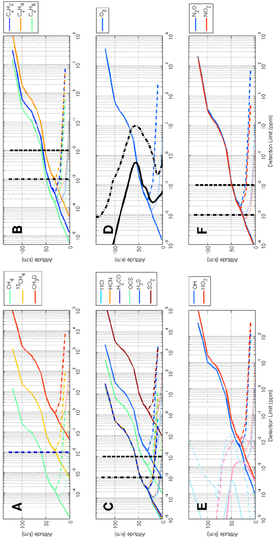
Fig. 20 Detection limits of \text{CH}_4 and other trace gases for several dust loadings, here expressed as aerosol optical depth (AOD): solid: AOD = 0.0, dotted: AOD = 0.1, and dash-dotted: AOD = 1.0. Panel A: detection limits for \text{CH}_4 and two of its isotopologues; the blue line indicates a vmr of 10 ppb which correspond to the maximum value observed by MSL (Webster et al. 2015). Panel B: detection limits of \text{C}_2\text{H}_2 , \text{C}_2\text{H}_4 , and \text{C}_2\text{H}_6 ; the black lines represent vmr values of 1 and 10 ppb respectively; Panel C: detection limits of \text{HCl} , \text{HCN} , \text{H}_2\text{CO} , \text{OCS} , \text{H}_2\text{S} , and \text{SO}_2 ; the black lines represent vmr values of 1 and 10 ppb respectively; Panel D: detection limits of \text{O}_3 ; the black lines represent results from the GEM-Mars model: solid line: yearly average profile; dash-dotted: profile made up of the maximum value calculated by the model at each altitude; Panel E: detection limits of \text{OH} and \text{HO}_2 ; the cyan ( \text{OH} ) and pink ( \text{HO}_2 ) lines represent results from the GEM-Mars model: solid line: yearly average profile; dash-dot: profile made up of the maximum value calculated by the model at each altitude; Panel F: detection limits of \text{N}_2\text{O} and \text{NO}_2 ; the black lines represent vmr values of 1 and 10 ppb respectively
