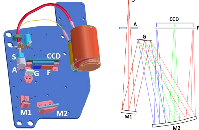
Fig. 7 Layout of the UVIS spectrometer: the entrance slit (S), the aperture (A), the collimating mirror (M1), the diffraction grating (G), the focusing mirror (M2), the 2nd order filter (F) and the detector (CCD)
