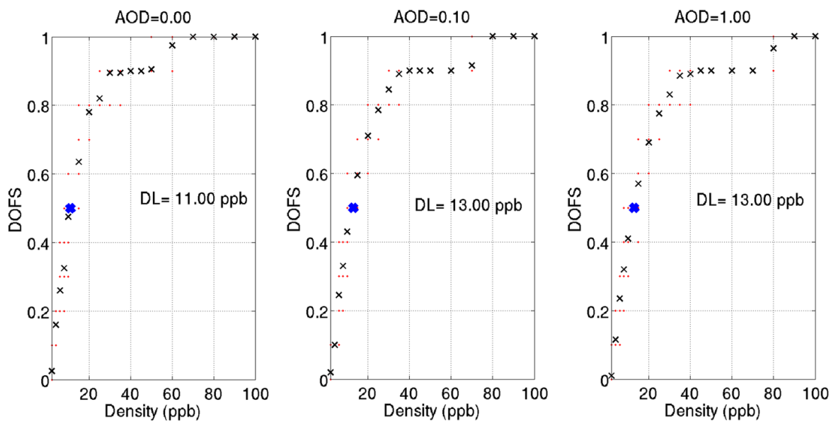
Fig. 28 Detection Limits for \text{CH}_4 in three scenarios of dust: AOD = 0 (left), AOD = 0.1 (center) and AOD = 1.0 (right). These results were obtained by retrieving methane in the diffraction order 134 i.e. spectral interval from 3011 to 3036 \text{ cm}^{-1} . The red dots show the 20 individual results. The 18 black markers indicate the mean Degree of Freedom of the Signal (DOFS) per factor tested. The DOFS equals to 0.5 is represented by the blue marker
