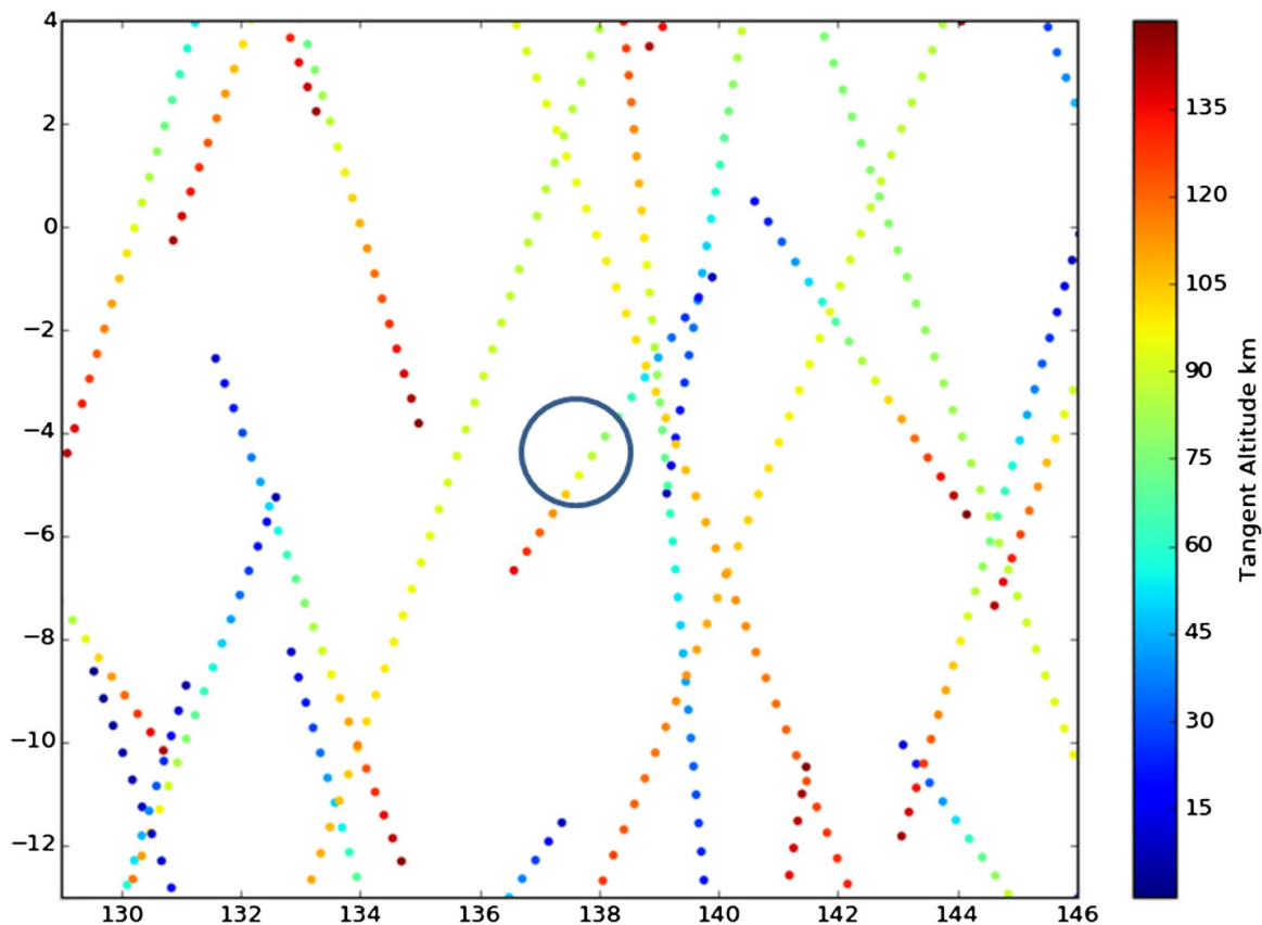
Fig. 15 Typical groundtrack coverage for solar occultation measurements near the location of the NASA Curiosity Rover landing site ( 4.5^{\circ}\text{S} , 137.5^{\circ}\text{E} ), for a 12-month simulation period from May 2018. Even close to the equator, the number of solar occultations is significant
