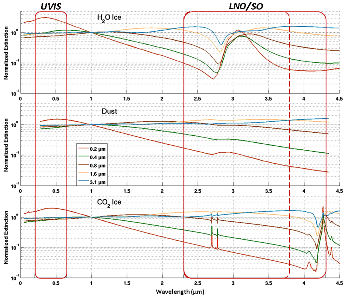
Fig. 27 Wavelength dependence of the computed normalized extinction for \text{H}_2\text{O} ice (top panel), dust (middle panel) and \text{CO}_2 ice (bottom panel) particles as a function of the wavelength and for different effective radii given by the color code in the middle panel. The spectral regions probed by NOMAD/UVIS, SO (red frames) and LNO (dashed line) are also indicated. The refractive indexes that are adopted for the Mie computation are from Warren and Brandt (2008) for \text{H}_2\text{O} ice, from Wolff et al. (2009, 2010) for Martian dust and from Hansen (1997, 2005) for \text{CO}_2 ice. The particle size distribution used is a log-normal distribution with r_{\text{eff}} = 0.2 \mu\text{m}
