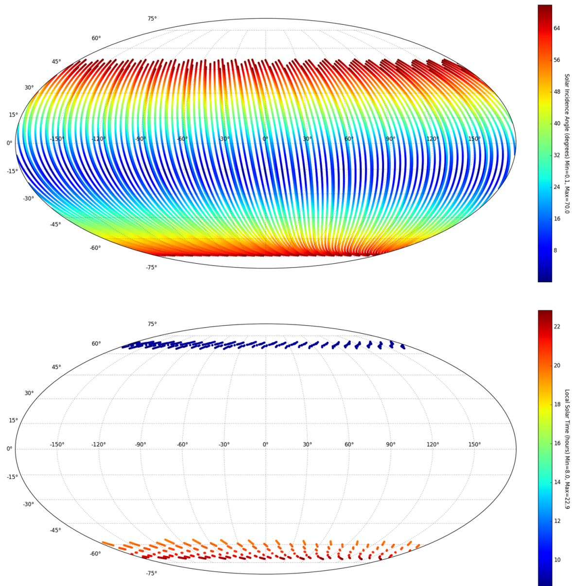
Fig. 12 Results of a 10-day orbit simulation where the beta angle is low. Top: dayside nadir coverage, showing how the solar zenith angle varies across the nadir groundtrack. Here a cut-off at 70^\circ was applied, hence no polar coverage or nightside nadir observations are plotted. In reality, the cut-off will be varied to avoid large gaps in coverage. Bottom: solar occultation coverage for the same 10 days, where the color denotes the local solar time, which here is around 10am or 10pm for this period
