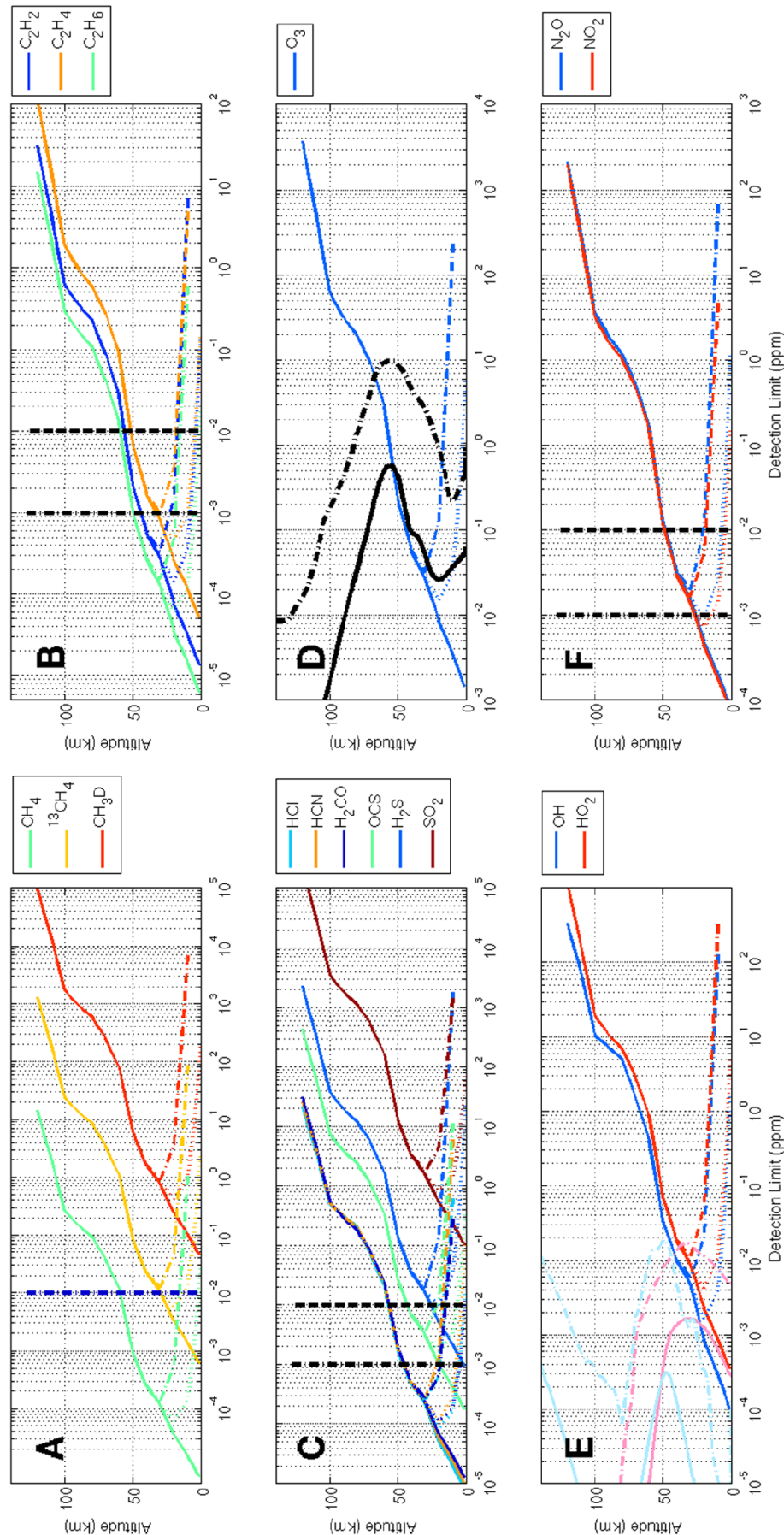
Fig. 20 Detection limits of CH 4 and other trace gases for several dust loadings, here expressed as aerosol optical depth (AOD): solid: AOD = 0.0, dotted: AOD = 0.1, and dash-dotted: AOD = 1.0. Panel A: detection limits for CH 4 and two of its isotopologues; the blue line indicates a vmr of 10 ppb which correspond to the maximum value observed by MSL (Webster et al. 2015). Panel B: detection limits of C 2 H 2 , C 2 H 4 , and C 2 H 6 ; the black lines represent vmr values of 1 and 10 ppb respectively; Panel C: detection limits of HCl, HCN, H 2 CO, OCS, H 2 S, and SO 2 ; the black lines represent vmr values of 1 and 10 ppb respectively; Panel D: detection limits of O 3 ; the black lines represent results from the GEM-Mars model; solid line: profile made up of the maximum value calculated by the model at each altitude; dash-dotted: yearly average profile; Panel E: detection limits of OH and HO 2 ; the cyan (OH) and pink (HO 2 ) lines represent results from the GEM-Mars model; solid line: yearly average profile; dash-dot: profile made up of the maximum value calculated by the model at each altitude; Panel F: detection limits of N 2 O and NO 2 ; the black lines represent vmr values of 1 and 10 ppb respectively
