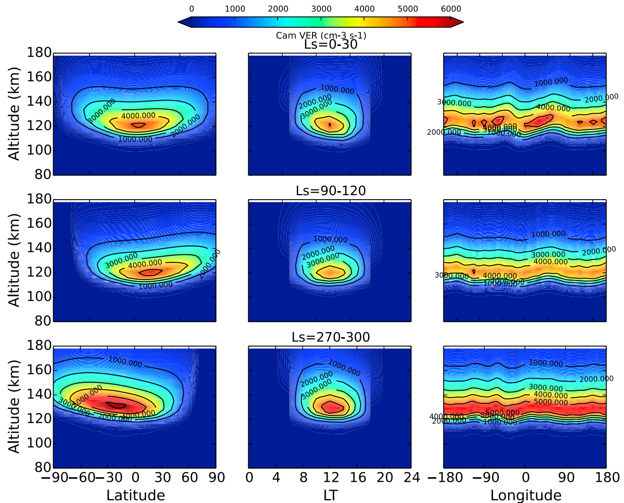
Figure 12. LMD-MGCM predicted variability of VER profiles for the Cameron bands as a function of latitude (left column), local time (center column), and longitude (right column), for the Ls = 0–30° (top), Ls = 90–120° (middle), and Ls = 270–300° (bottom) seasons. VER = volume emission rate.
