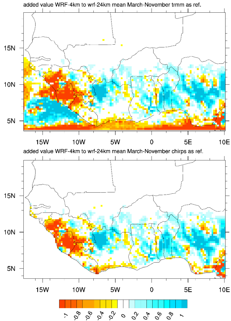
Fig. 3 Added value of high resolution (wrf-4km) simulation to coarse resolution (wrf-24km): on top computed using TRMM as reference dataset and the bottom computed using CHIRPS dataset as the reference.
