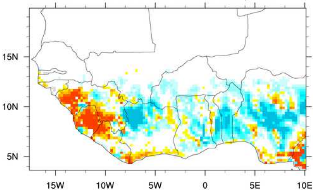
added value WRF-4km to wrf-24km mean March-November chirps as ref.
