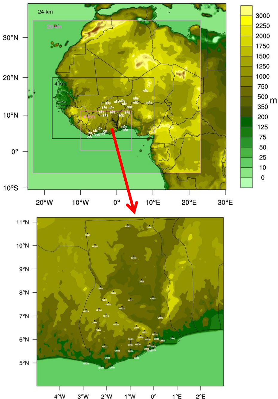
Fig. 1 Top: WRF model domain and elevation (m); parent domain at 24 km horizontal resolution (25°W–30°E,10°S–40°N). The nested domain is depicted by the back box (17°W–10°E,4°N–20°N) black boxes (first set of runs). The pink boxes correspond to the domains for the second set of runs (sensitivity to MP and PBL schemes) where parent domain is at 20 km horizontal resolution (25°W–30°E,10°S–40°N). The nested domain covers the southern coastal area (10°W–5°E,0°N–12°N). The white dots indicate the ground-based stations used. Bottom: Zoom over Ghana (Table 1 provides the name and coordinates of the stations cited in the manuscript)
