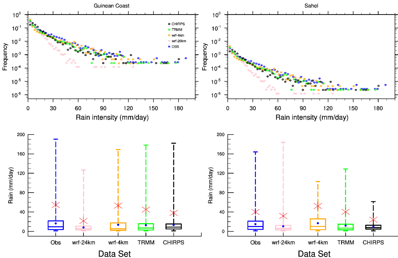
Fig. 5 Empirical probability distribution functions of daily precipitation (top) daily. Boxplots of the daily precipitation (Bottom) respectively from the ground-based observations, wrf-24km, wrf-4km, TRMM and CHIRPS data sets over the Guinean coast (left) and the Sahelian (right) regions. The boxes indicate respectively from the bottom to the top the first, second and third interquartile ranges and the whiskers stretch to minimum and maximum values of each data set. Blue dots and the red stars represent respectively the mean value and the 95 th percentile of the precipitation for each data set.
