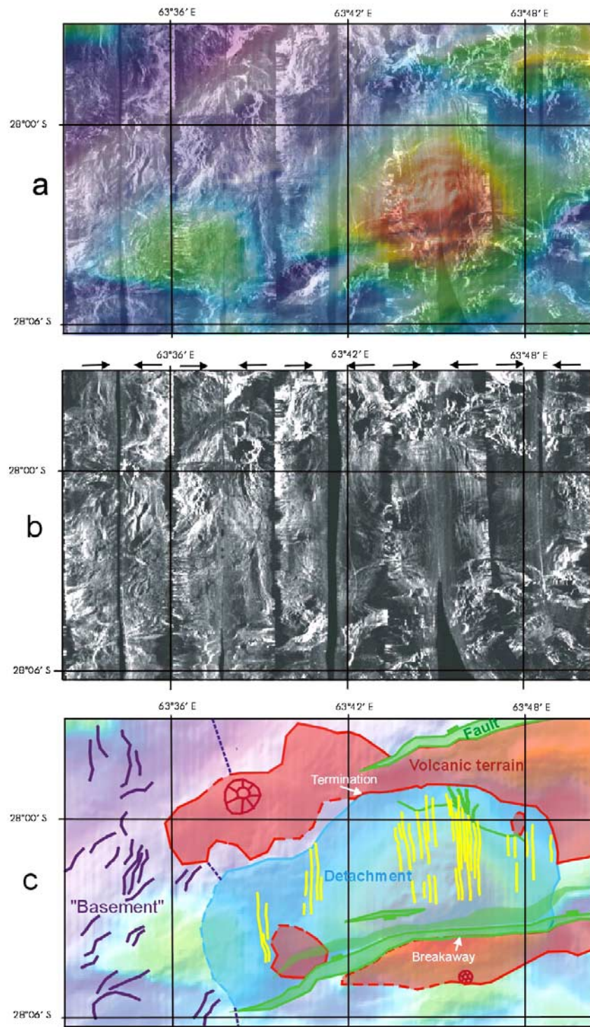
Figure 2. (a) TOBI side scan mosaic overlain by coloured bathymetry in the area of the FUJI Dome detachment. (b) Side-scan sonar mosaic, corrected for slant-range distortion and variations in vehicle height. Light tones represent strong acoustic backscatter. Arrows at top of image show insonification direction for each swathe. (c) Geological interpretation based on side scan and bathymetry superimposed on bathymetry image. Red, volcanic terrains and volcanoes; blue: detachment surface; yellow, spreading-parallel lineaments on detachment; green, normal faults; purple, curved lineaments of "basement" terrain (see text). Outlines are dashed where uncertain. See Figure 1 for location.
