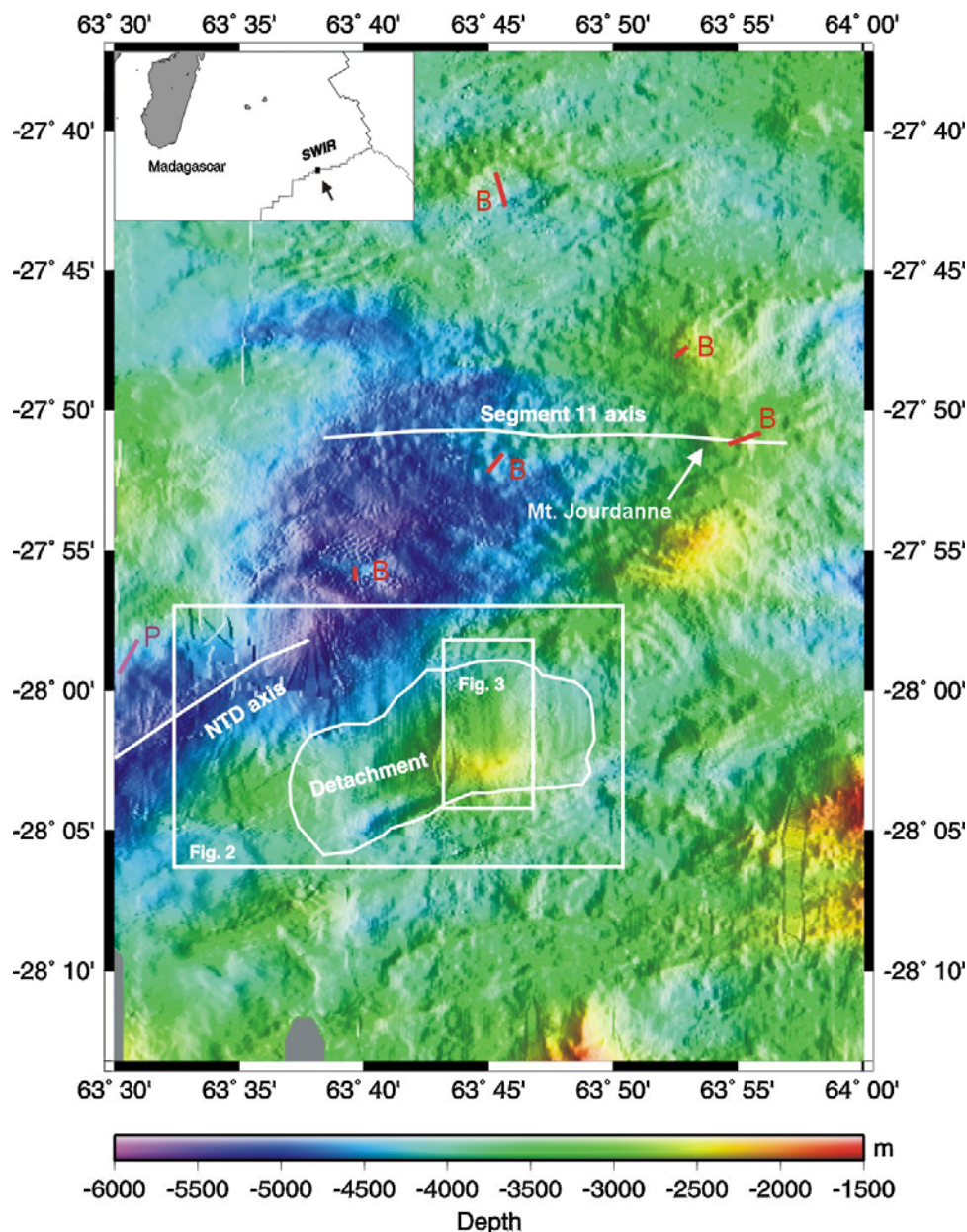
Figure 1. Seafloor topography (shaded relief, illuminated from east, depth in meters), showing the FUJI Dome on the southern flank of the southwest Indian Ridge. Red bars marked “B” show positions of basalt dredges; purple bar marked “P” a peridotite dredge [Mével et al. , 1997a]. Inset shows regional location, with study area arrowed.
