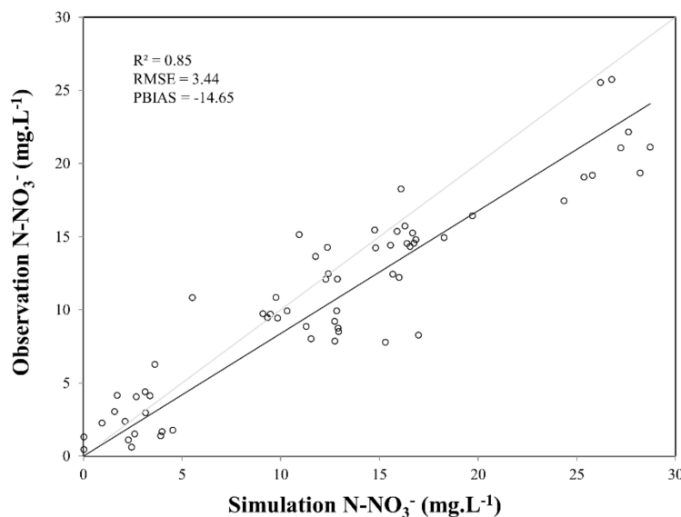
Figure 6. Observed and simulated (dilution plus denitrification) groundwater nitrate concentration in the two periods (2004–2005 and 2013).
