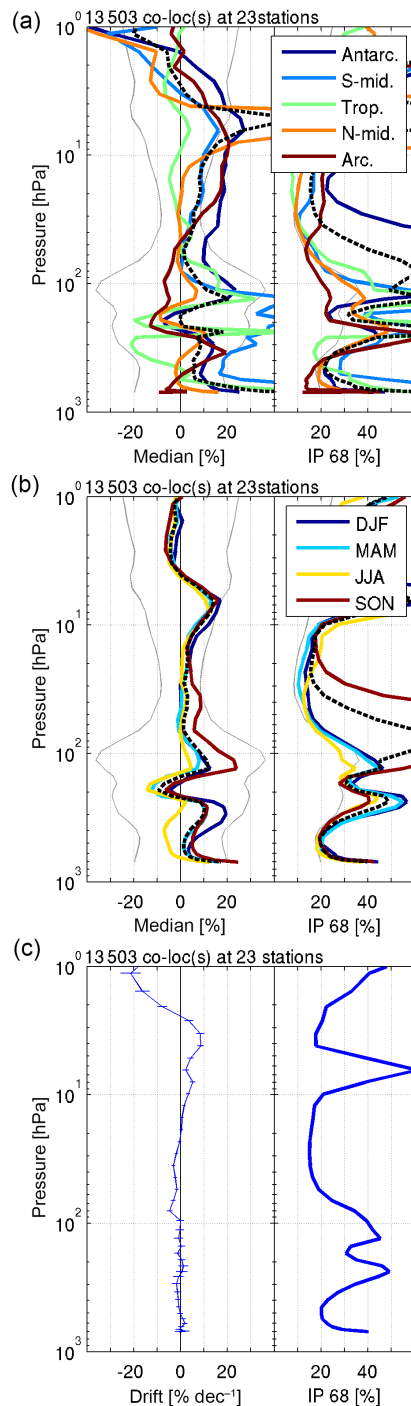
Figure 13. Median relative differences and 68 % interpercentile spreads for comparison of L4 assimilated nadir ozone profile data with ground-based reference measurements (a, b). The same difference statistics are redistributed over two influence quantity ranges, with the influence quantities being the latitude (a) and quarter (b). The black dashed line shows the average of the coloured curves, while light grey lines indicate the satellite uncertainty provided in the product. Panel (c) shows the corresponding relative decadal drift and 68 % interpercentile spread. Two sigma error bars, resulting from a bootstrapping with 1000 samples, are added to the drift profile.
