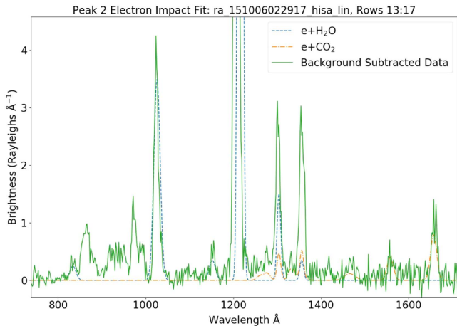
Figure 5. Quiescent and background-subtracted spectrum from the second spike with dissociative electron impact of \text{H}_2\text{O} and \text{CO}_2 ( e+\text{H}_2\text{O} and e+\text{CO}_2 ) model spectra. The expected emission from O I 1304 Å and O I 1356 Å from these two sources is then subtracted from the total, as shown in Equations (1) and (2).
