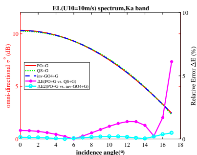
Fig. A2. \sigma^0(\theta) (in dB) as a function of \theta with the PO model (red line) for a 10 m/s wind speed, using EL spectrum, for Ka-band. Color codes and symbols are the same as in Fig.1
