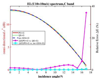
Fig. A1. \sigma^0(\theta) (in dB) as a function of \theta with the PO model (red line) for a 10 m/s wind speed, using EL spectrum, for C-band. Color codes and symbols are the same as in Fig.1
