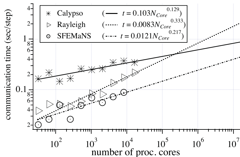
Figure 4. The data communication time per step in the weak-scaling test for the three codes shown in Figure 2. Lines are power law fits of elapsed time t in seconds/step extrapolated to a million processor cores.
