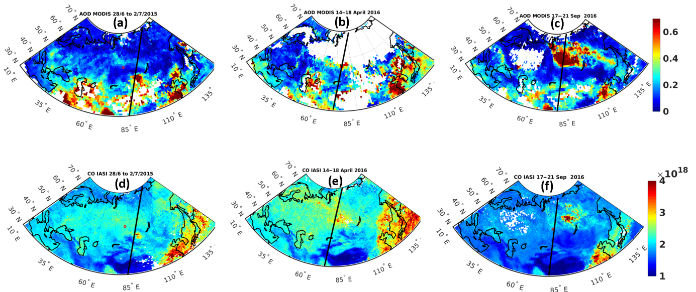
Figure 13. Five-day average of AOD at 532 nm from 1^\circ \times 1^\circ MODIS observations (a, b, c) and of CO in molecules \text{cm}^{-2} from IASI observations (d, e, f) for July 2015 (a, d), April 2016 (b, e) and September 2016 (c, f). The red circle is Tomsk and the thick black lines are the CALIOP overpasses shown in Figs. 14 to 16.
