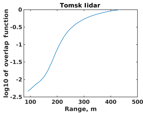
Figure 2. Geometrical overlap function used for the correction of the lidar data in log10 scale between 100 and 500 m.
