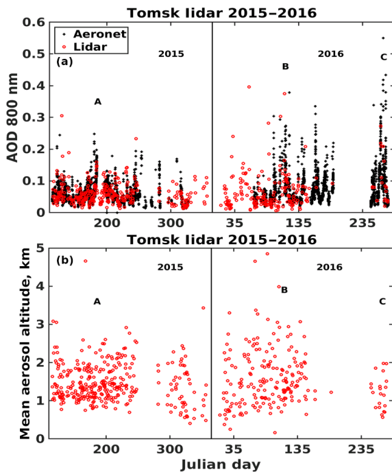
Figure 8. Time evolution from April 2015 to September 2016 of the 800 nm AOD for lidar (red) and sun-photometer (black) observations (a) and corresponding aerosol altitudes z_{\text{aer}} given by Eq. (2) (b). A, B, and C are the cases analysed in Sect. 5.
