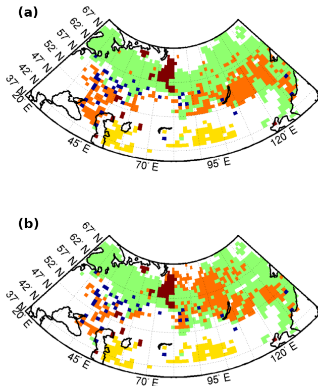
Figure 5. Map of the 2015 (a) and 2016 (b) aerosol sources coupled with a FLEXPART PES gridded map: grid cells with large cities (blue square), central Asia desert (yellow), biomass burning (light brown), gas flaring (dark brown) and taiga (green).
