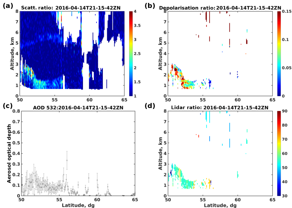
Figure 14. Latitudinal cross section of CALIOP 532 nm scattering ratio R_{532} (a), aerosol depolarization ratio \delta_{532} (b), aerosol optical depth AOD_{532} (c) and lidar ratio S_{532} (d) for 14 April 2016.
