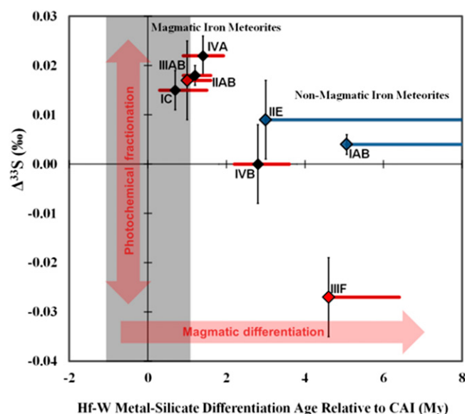
Fig. 2. \Delta^{33}\text{S} vs. exposure-corrected Hf-W metal-silicate segregation ages. Average \Delta^{33}\text{S} for each group of magmatic (red) ( n = 6 ) and nonmagmatic (blue) ( n = 2 ) iron meteorites plotted against Hf-W ages. Solid black diamonds represent preexposure \epsilon^{182}\text{W} values (6), hollow diamonds represent maximum calculated cosmogenic exposure corrections on groups IC and IIIF (8), and Sm-based corrections on IAB and IIE (7). Colored lines span the range of maximum corrected values from available data. Error bars represent 2SE for IAB, IVA, IIAB, & IIIAB, and 2s.d. ( \pm 0.008\% ) for other groups. Gray band represents uncertainty in calcium-aluminum inclusion (CAI) initial.
