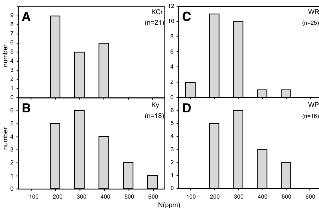
Figure 5. Comparison of nitrogen content for diamonds recovered from the Luobusa chromitites and mantle peridotites, and from the Ray-Iz chromitites. (A) Nitrogen content for diamonds recovered from the Luobusa chromitite. (B) Nitrogen content for diamonds recovered from the Luobusa mantle peridotite. (C, D) Nitrogen content for diamonds recovered from the Ray-Iz chromitite.
