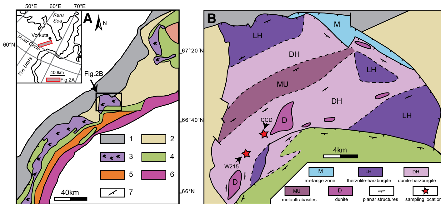
Figure 2. Simplified geological maps of the Vorkuta ophiolite belt in the Polar Urals and the Ray-iz ophiolite (revised after Yang et al., 2015). (A) Index map of the northern Ural Mountains. 1—Allocthonous Paleozoic sedimentary assemblages of the continental shelf and slope, volcanic units (Lemva Zone), and pre-Ordovician bimodal volcanic series (Uraltau Zone). 2—Precambrian and pre-Paleozoic volcanic and sedimentary complexes of the crystalline basement of the East European platform. 3—Ultramafic rocks, mainly harzburgite and dunite with minor lherzolite. 4—Metamorphosed gabbro, olivine gabbro, and minor troctolite and pyroxenite. 5—Early Devonian tonalite and granodiorite and Middle Devonian diorite and monzodiorite. 6—Island-arc complex. 7—Major thrust faults and fault systems. (B) Geologic map of the Ray-iz ophiolite.
