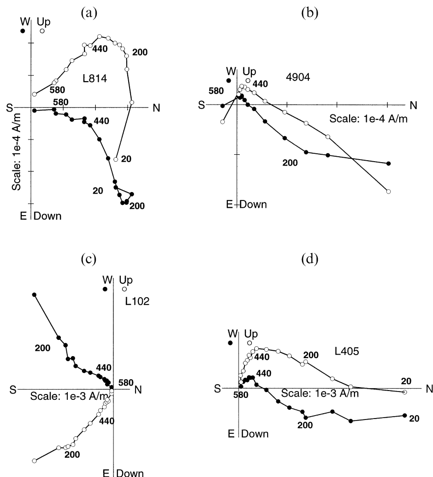
Figure 6. Orthogonal vector diagrams in stratigraphic coordinates of progressive thermal demagnetization for samples from the Norian limestones of the Abadeh region. The filled and open symbols refer to the horizontal and vertical plane, respectively. Three components are observed in each of these four examples.
