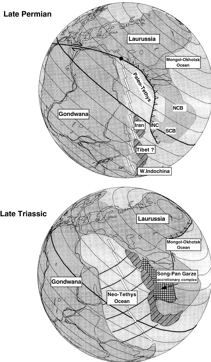
Figure 11. Palaeogeographic reconstruction of the Tethyan ocean and its bordering continents during the Late Permian and the Late Triassic. Cross-hatched areas, Cimmerian blocks; solid line, palaeoequator; the heavy lines perpendicular to the ridge indicate the motion of the Iranian blocks between Gondwana and Laurussia (indicated as transform faults). Open triangles, subduction zones; filled circle, the fault-ridge-trench triple junction. NCB, North China block; SCB, South China block; INC, Indochina.
