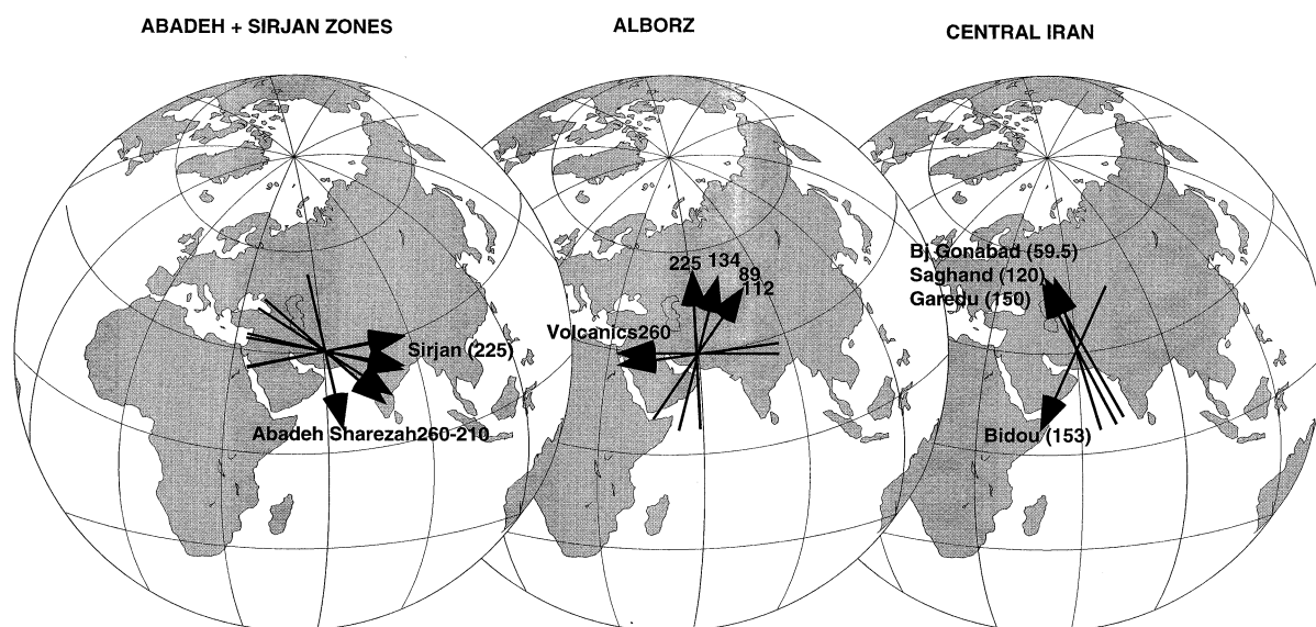
Figure 10. Difference between observed Iranian and expected Eurasian declinations for three Iranian regions. Note the very large rotations showing the complex tectonic history of these regions.
