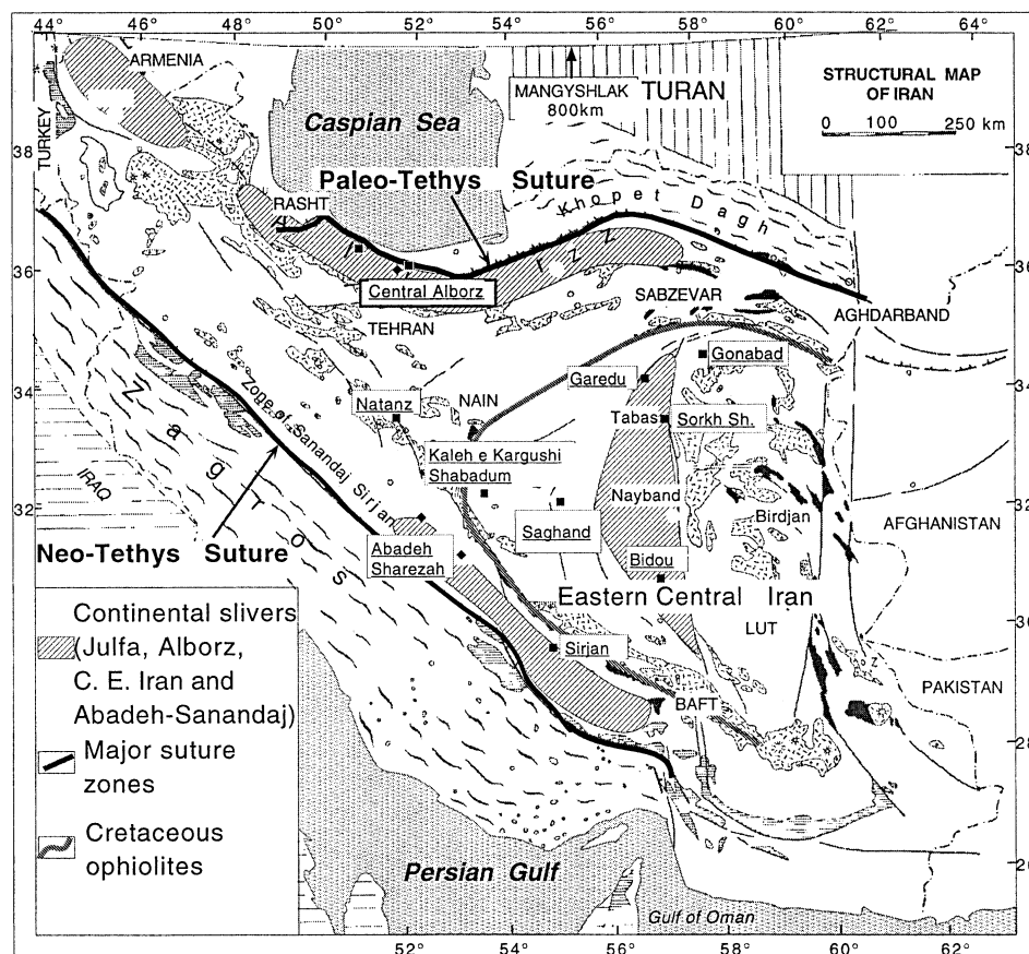
Figure 1. Simplified geological map of Iran showing the locations of the palaeomagnetic sampling sites (diamonds, this study; squares, other studies), the main Palaeo- and Neotethyan sutures, and the Nain–Sabzevar and Nain–Baft alignments corresponding to Cretaceous ophiolites.
