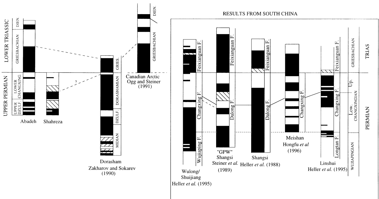
Figure 5. Correlation of Permian-Triassic magnetostratigraphic sections from Iran (Abadeh and Shahreza, this study), south China, Canadian Arctic and the former USSR.
