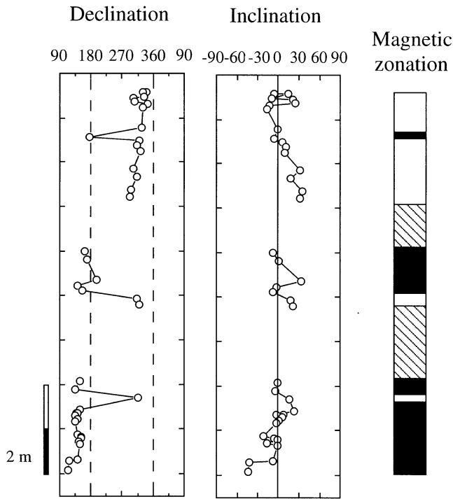
Figure 4. Magnetostratigraphy of the Hambast Formation (Dorashamian) in the Shahreza area. Left to right: declinations, inclinations and magnetic zonation versus stratigraphic depth. The polarity zonation is shown assuming a southern hemisphere of deposition.
