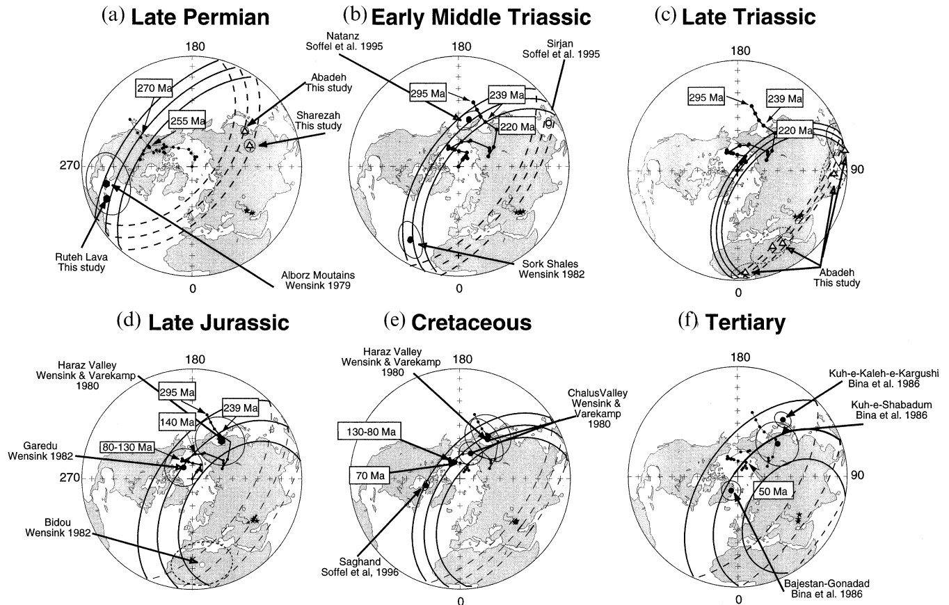
Figure 8. Equal-area projection showing our Iranian selected directions for six time windows: (a) Late Permian, (b) Early–Middle Triassic (c) Late Triassic, (d) late Jurassic, (e) Cretaceous and (f) Cenozoic. The poles are listed in Table 2 and described in Appendix A. Poles from Alborz are indicated by hexagons, poles from central Iran by circles, and poles from the Sanandaj–Sirjan zone by triangles. Poles in the upper and lower hemisphere are represented by filled and open symbols, respectively. The Gondwanian apparent polar wander path (APWP) is shown in (a) and the Eurasian APWP in (b)–(f). The small circles representing the possible loci of poles are centred on the sampling sites (represented by stars).
