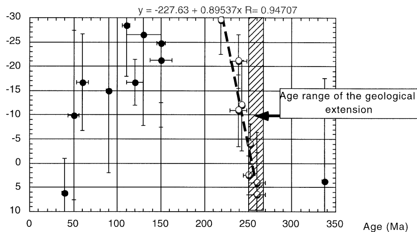
Figure 9. (a) Differences between the observed Iranian and predicted Eurasian palaeolatitudes. The horizontal error bars are the age errors in the Iranian data, and the vertical error bars are the errors of latitude difference computed as (\lambda_{\text{predicted}}^2 + \lambda_{\text{observed}}^2)^{1/2} , where \lambda is the palaeolatitude. The grey areas represent the corresponding errors for the poles, with age uncertainties of \pm 10 Myr. The dashed line is an estimation of the palaeomagnetic age of collision made using a linear regression on data between 260 and 219 Ma. Note the high value of the correlation coefficient R . (b) Difference between predicted Iranian and expected Gondwanian palaeolatitudes. The symbols are the same as in (a). The northward component of the motion of Iran with respect to Africa is around 10 \text{ cm yr}^{-1} .
