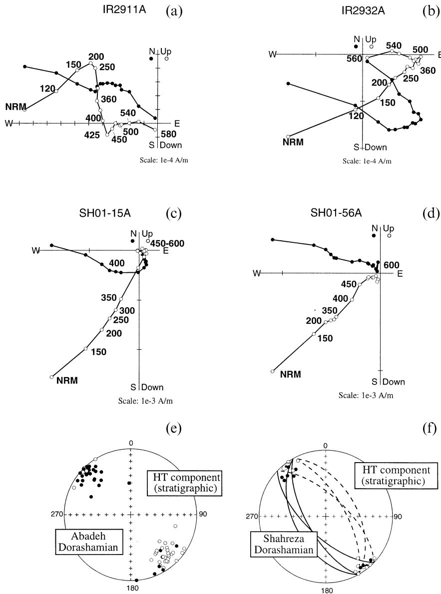
Figure 3. (a)–(d) Orthogonal vector diagrams in stratigraphic coordinates of progressive thermal demagnetization of samples from the Dorashamian of (a), (b) Abadeh and (c), (d) Shahreza. The filled and open symbols refer to the horizontal and vertical plane, respectively. (e), (f). Equal-area projections of the characteristic high-temperature directions for (e) Abadeh and (f) Shahreza.
