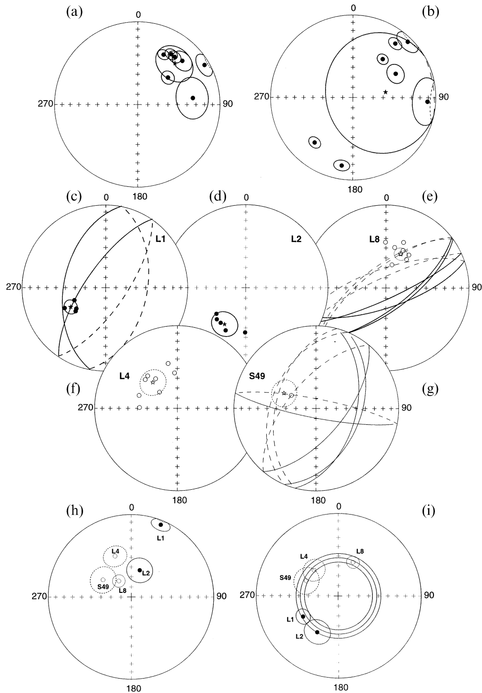
Figure 7. (a), (b) Equal-area projections of the middle-temperature component directions of Abadeh samples (a) before and (b) after bedding corrections. (c)–(g) Equal-area projections in stratigraphic coordinates of the directions carried by the characteristic high-temperature component of samples from Abadeh (sites S49, L1, L2, L4, L8). (h), (i) Equal-area projections of the mean directions carried by the characteristic high-temperature component of samples from Abadeh (Norian) before and after bedding correction. The difference in declinations indicates relative rotations between these sites.
