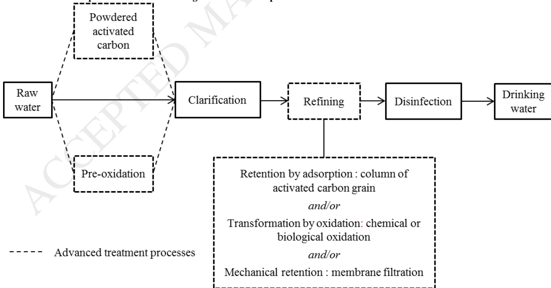
FIGURE 3: Representation of a drinking water treatment plant
