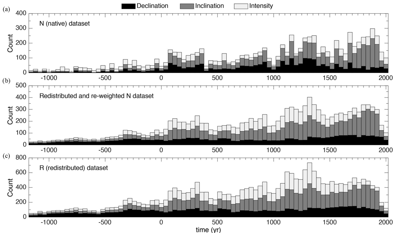
Figure 5. Histograms of the archaeomagnetic data sets used in this study. (a) The native (N) data set constructed from Geomag50.V2 (Donadini et al. 2009); (b) redistribution of the N data set given the re-weighting based on the probability density function of the age of each datum, counted by their weights; (c) the redistributed (R) data set, which assumes that the redistributed data are independent, with a recalibrated measurement uncertainty. See the text for details.
