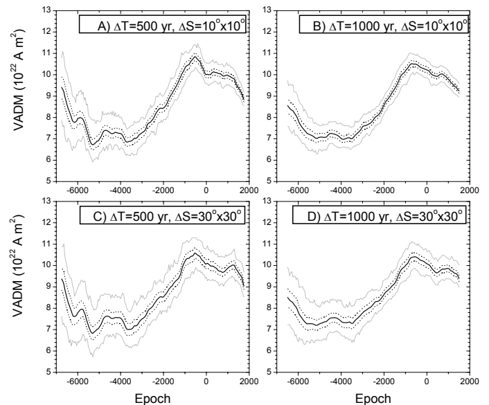
Fig. A.2. Comparison between VADM curves computed between 7000 BC and 2000 AD using sliding windows of \Delta T = 500 years (panels A, C)) and 1000 years (B, D)) shifted by 50 years, and using a weighting over regions of \Delta S = 10^\circ \times 10^\circ (A, B)) and \Delta S = 30^\circ \times 30^\circ (C, D) width. The thick black line exhibits the averaged VADM computed using a bootstrap scheme (see main text and legend of Tables C.1 and C.2 available at CDS), with its 1\sigma uncertainties (dotted lines) and the envelope of possible VADM values (gray lines).
