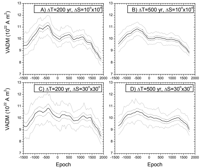
Fig. A.1. Comparison between VADM curves computed between 1500 BC and 2000 AD using sliding windows of \Delta T = 200 years (panels A, C)) and 500 years (B, D)) shifted by 50 years, and using a weighting over regions of \Delta S = 10^\circ \times 10^\circ (A, B)) and \Delta S = 30^\circ \times 30^\circ (C, D) width. The thick black line exhibits the averaged VADM computed using a bootstrap scheme (see main text and legend of Tables C.1 and C.2 available at CDS), with its 1\sigma uncertainties (dotted lines) and the envelope of possible VADM values (gray lines).
