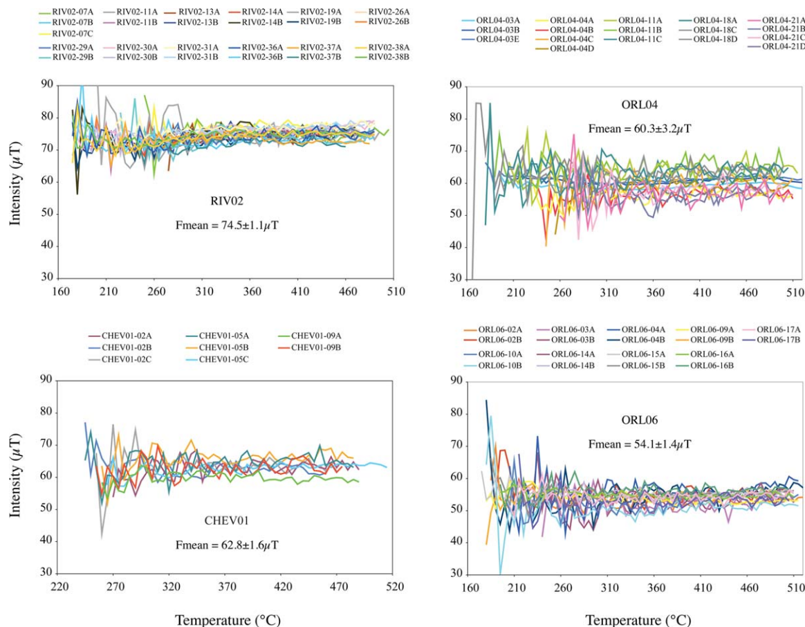
Figure 3. Intensity determinations that fulfill our selection criteria for four groups of archeological fragments. Individual curves represent the intensity values computed using the R^*(Ti) ratios for one specimen over the temperature interval of analysis [Le Goff and Gallet, 2004] (see Figure S1, supporting information for intensity determinations from eight other groups of fragments).
