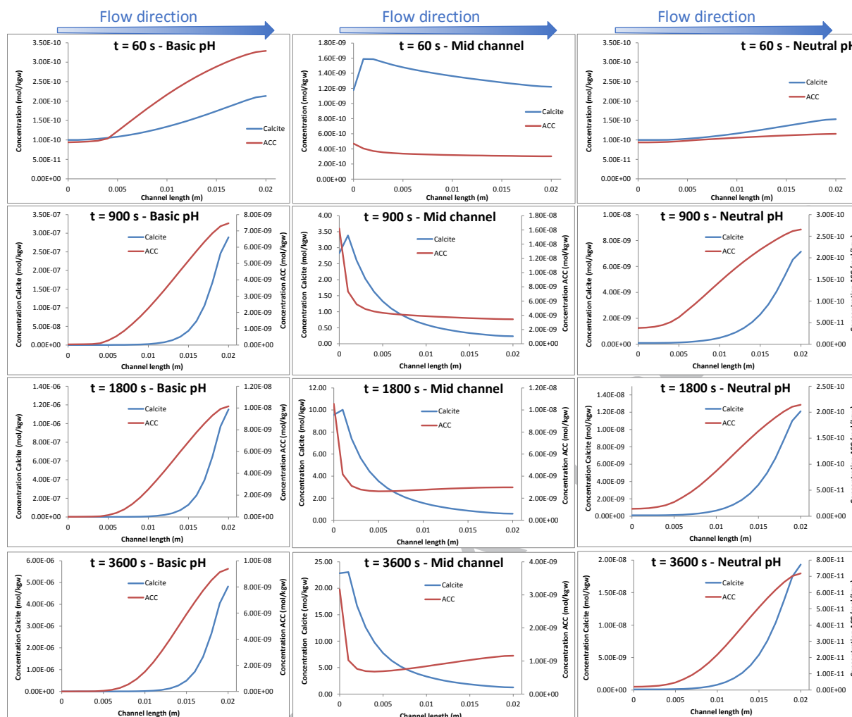
Figure 8 – Variation of carbonate complex (solid red lines) and calcite (solid blue lines) along the channel at time = 60 seconds (first line), 900 seconds (second line), 1800 seconds (third line) and 3600 seconds (fourth line). Left column: basic part of the channel ( y = 0.000375 m), second picture: in the center of the channel ( y = 0.00025 m), right picture: neutral part of the channel ( y = 0.000125 m)
