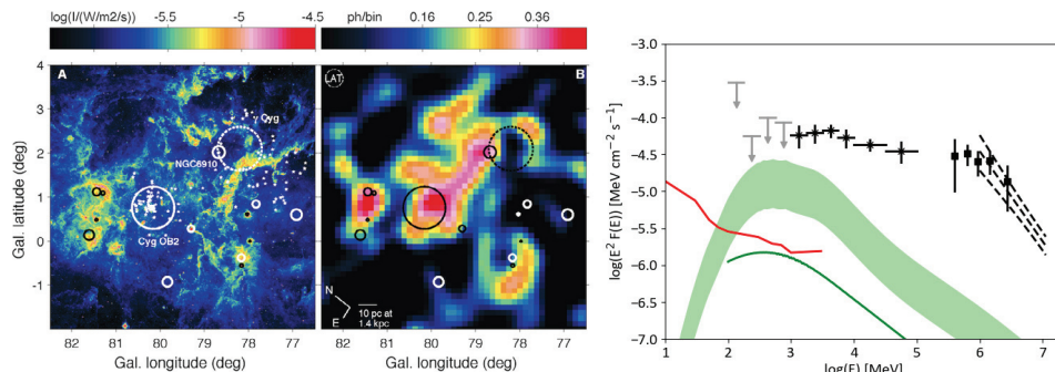
Figure 3.3.1: Left: 8\ \mu\text{m} intensity map of the Cygnus X region from MSX showing the heated contours of the superbubble. OB stars (white stars), OB associations (white circles), and the supernova remnant \gamma Cygni (dashed circle) are overlaid [307]. Center: Fermi -LAT photon count map of the same region in the 10-100 GeV band. The 50-pc-wide excess coincident with the bubble signals a cocoon of freshly accelerated CRs [307]. Right: Energy spectrum of the Cygnus cocoon emission as detected by Fermi -LAT (crosses), ARGO-YBG (squares), and MILAGRO (dashed lines). The curves show model expectations from normal Galactic CRs spreading the ionized gas (green band) or up-scattering the stellar and interstellar light fields (green curve). The sensitivity of e-ASTROGAM (red curve) is given for one year of effective exposure in the Galactic disc. Adapted from [306, 307].
