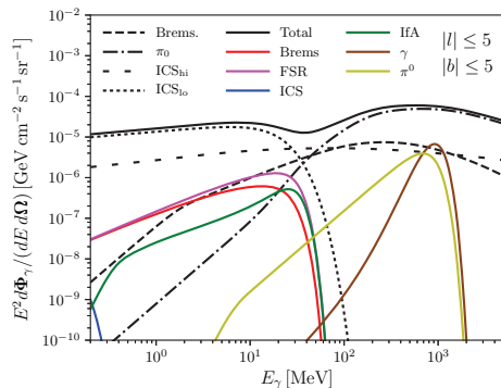
Figure 4.5.1: Total background emission in the inner 10^\circ \times 10^\circ (black, solid) and broken down into subcomponents (interrupted). Colored lines show spectral features from primary and secondary emission due to DM annihilation, convolved with an energy resolution of \Delta E/E = 0.3 . The yellow (box) and brown lines (monochromatic photon) are for \chi\chi \rightarrow \pi^0\gamma with m_\chi = 800 MeV. The red, magenta, blue and green line correspond to the emission for an m_\chi = 30 MeV DM particle annihilating to e^+e^- . In both cases \langle\sigma v\rangle = 10^{-28} cm 3 s -1 . See Ref. [393] for details.
