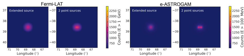
Figure 4.8.2: Comparison between the Fermi -LAT and e-ASTROGAM abilities to resolve between an extended source and two nearby point sources (extracted from [460]). See text for details.
