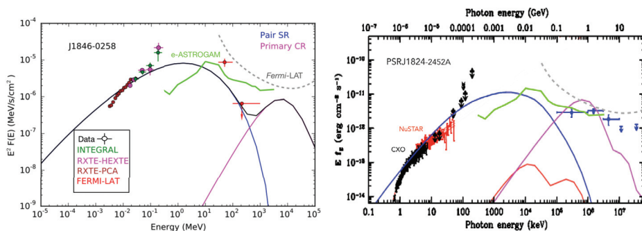
Figure 6.4.2: SEDs of the young pulsar J1846-0258 (left) and of the millisecond pulsar J1824-2452A (right). The model curves show the expected curvature radiation (magenta) and synchrotron radiation (red) from the primary particles accelerated in the current sheet, and the synchrotron radiation (blue) from the secondary pairs produced in cascades and radiating in the open magnetosphere. Adapted from [664], [667] and [668], with J1846-0258 data from [615] and [666]. The sensitivities of e-ASTROGAM (solid green) and of Fermi -LAT (dashed gray) are given for one year of effective exposure in the Galactic disk.
