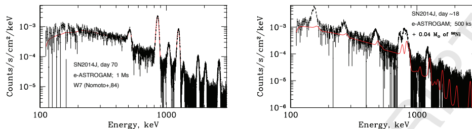
Figure 5.1.1: Left: Simulated background-subtracted spectrum of a SN event like SN 2014J (distance of 3.5 Mpc; 70 days after explosion; 1 Ms exposure). The spectrum is dominated by ^{56}\text{Co} lines, scattered continuum and annihilation emission. The W7 model [546]. Such event would be detected at \sim 300\sigma by e-ASTROGAM. Right: Simulated spectrum for a model with 0.04 M_{\odot} of radioactive ^{56}\text{Ni} located outside the main ejecta (3.5 Mpc; 500 ks exposure centered at day 17.5 after explosion; 3Dball model from [550]). Extremely bright lines of ^{56}\text{Ni} at 158 and 810 keV are clearly detected. Such lines would not be seen if all ^{56}\text{Ni} is confined within the ejecta (see red curve that shows a canonical model).
