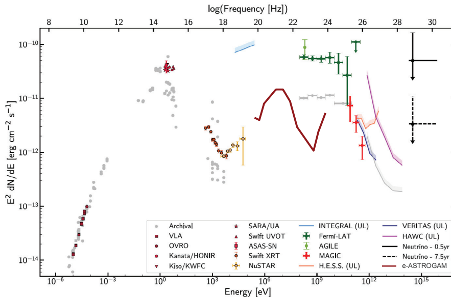
Figure 2.2.1: SED of the blazar TXS 0506+056, from [4]. Dark points represent data taken during the flare; grey points correspond to non-flaring states. The e-ASTROGAM expected sensitivity (solid brown) is calculated for an effective exposure of 7 days, corresponding to the observations by Fermi -LAT and MAGIC during the flare.
