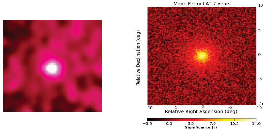
Figure 7.2.1: Images of the Moon seen by EGRET [762] (left) and by the Fermi -LAT [764] (right). The EGRET plot covers a field of view of roughly 40^\circ .
