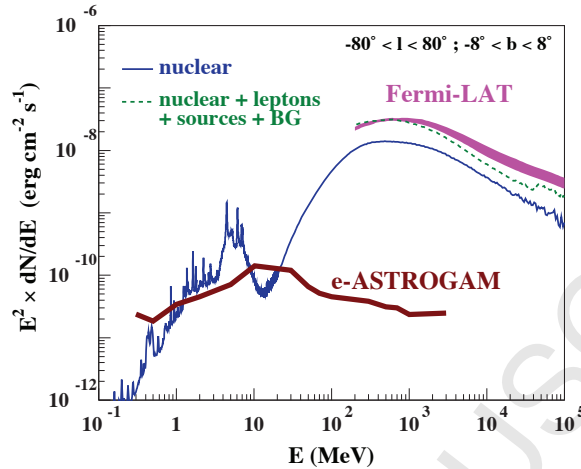
Figure 3.5.1: Predicted gamma-ray emission due to nuclear interactions of CRs in the inner Galaxy (longitude -80^\circ \leq l \leq 80^\circ and latitude -8^\circ \leq b \leq 8^\circ ). The gamma-ray line emission below 10 MeV is due to LECRs, whose properties in the ISM have been adjusted such that the mean CR ionization rate deduced from H_3^+ observations and the Fermi -LAT data (magenta band) at 1 GeV are simultaneously reproduced (adapted from [347]). The dashed green line shows the total calculated emission when adding leptonic contributions, point sources and extragalactic gamma-ray background that were taken from [344]. The 1-year sensitivity of e-ASTROGAM (for Galactic background) is superimposed.
