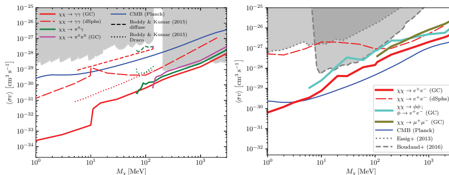
Figure 4.5.2: Projected 95% CL upper-limits on DM annihilating to various final states. Adapted from Ref. [393]. Projections are compared to current limits from the CMB (blue, [372]). Left: Projections from [393] DM annihilation into \gamma\gamma (red, solid=GC, long-dashed=dSphs), \pi^0\gamma (green) and \pi^0\pi^0 (magenta). The CMB constraints are for \chi\chi \rightarrow \gamma\gamma [372, 408]. For the same channel we show gamma-ray limits derived [394] and [429] in grey. Right: Projected 95% CL upper-limit on gamma-ray emission from DM annihilating to e^+e^- . Results are for the total DM spectrum from the three reference leptonic cases: direct annihilation (red, solid=GC, long-dashed=dSphs), cascade channel (turquoise) and the muon channel (olive). The blue solid line shows the CMB limits on DM s -wave annihilation into e^+e^- from Planck [372, 408]. In addition we show in light-grey the limits for \chi\chi \rightarrow e^+e^- from Voyager [433] and current limits from diffuse emission gamma-rays [417].
