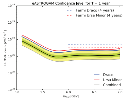
Figure 4.7.1: Sensitivity for \langle \sigma v \rangle from observation of the classical dwarf galaxy Draco and Ursa Minor for self-annihilation channel b\bar{b} .
