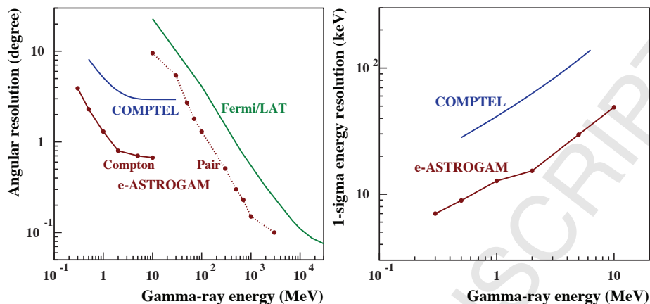
Figure 1.3.1: Left: e-ASTROGAM on-axis angular resolution compared to that of COMPTEL and Fermi -LAT. In the Compton domain, the presented performance of e-ASTROGAM and COMPTEL is the FWHM of the angular resolution measure (ARM). In the pair domain, the PSF is the 68% containment radius for a 30^\circ point source. The Fermi -LAT PSF is from the Pass 8 analysis (release 2 version 6) and corresponds to the FRONT and PSF event type. Right: 1\sigma energy resolution of COMPTEL and e-ASTROGAM in the Compton domain after event reconstruction and selection on the ARM.
