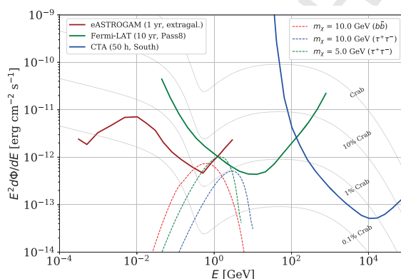
Figure 4.8.1: e-ASTROGAM differential sensitivity (solid brown line) to point-like WIMP DM subhalos, compared to those of the Fermi -LAT (green) and the future CTA (blue). Dashed lines represent examples of DM subhalo energy fluxes for three DM particle models. A J -factor value of 1.5 \times 10^{19} \text{ GeV}^2 \text{ cm}^{-5} and a \langle \sigma_{ann} v \rangle value of 2.2 \times 10^{-26} \text{ cm}^3 \text{ s}^{-1} have been assumed. See text for further details.
