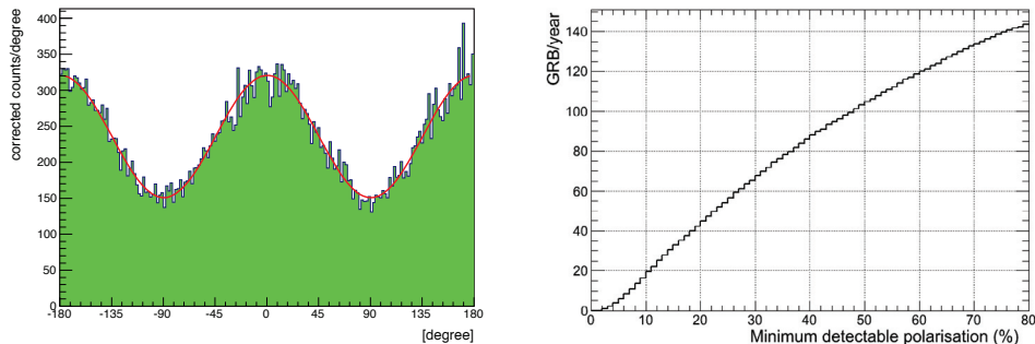
Figure 1.3.2: Left: e-ASTROGAM polarization response (polarigramme) in the 0.2 – 2 MeV range for a 100% polarized, 10 mCrab-like source observed on axis for 10^6 s. The corresponding modulation is \mu_{100} = 0.36 . Right: Cumulative number of GRBs to be detected by e-ASTROGAM as a function of the minimum detectable polarization at the 99% confidence level.
