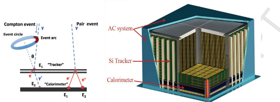
Figure 1.2.2: Left: Representative topologies for a Compton event and for a pair event. Photon tracks are shown in pale blue, dashed, and electron and/or positron tracks are in red, solid. Right: Overview of the e-ASTROGAM payload.
