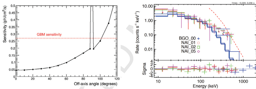
Figure 2.1.2: Left: 6\sigma sensitivity of e-ASTROGAM to an average GRB on a 1 second timescale in the 0.2–2 MeV band. The sharp loss of sensitivity at 90^\circ incidence is due to gamma-rays crossing the tracker parallel to the silicon detectors. The red line gives the equivalent trigger sensitivity of Fermi GBM, adapted from [50]. Right: the flux from the hard component of GRB170817A as recorded from Fermi GBM (solid blue line), and a conservative extrapolation (20x) to an on-axis flux (dashed red line).
