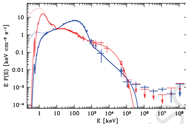
Figure 6.7.1: Broad-band X-ray/gamma-ray spectra for Cyg X-1 in the hard (blue heavy symbols) and soft (red thin symbols) states. The data at < 10 MeV (attenuated by X-ray absorption) are from BeppoSAX and CGRO, while the data at \geq 40 MeV are from Fermi/LAT. Data are compared to hybrid-Comptonization accretion-flow models [696]. The observed emission above \sim 100 MeV in the hard state is dominated by the jet. The dotted curves at soft X-rays show the unabsorbed models.
