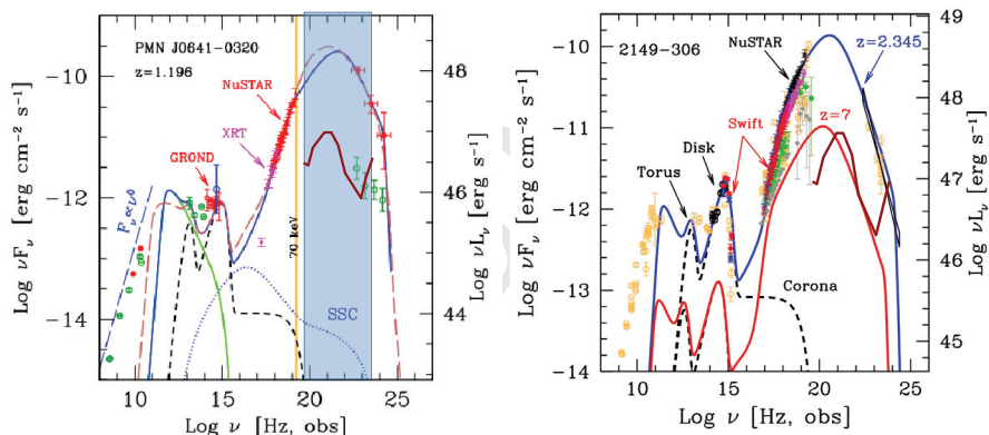
Figure 2.6.1: Left: SED and model of the MeV blazar PMN J0641-0320 taken from [141]. Observations with quasi-simultaneous observations by GROND, Swift , NuSTAR and Fermi -LAT (in red). The black dashed curve represents to contribution of the torus, accretion disc and X-ray corona. The solid green line shows the synchrotron emission. The solid blue line represents a model with external photon field in the BLR, while the dashed brown model takes into account a photon field of the region between the BLR and the torus. In blue the energy range of e-ASTROGAM is marked to illustrate the coverage of the MeV energy where we have a gap of observations due to the lack of an instrument like e-ASTROGAM. Its expected sensitivity is shown (solid brown line) for an effective exposure of 7 days, corresponding to the integration time of Fermi -LAT data. Right: SED and model of the MeV blazar PKS 2149-306 (redshift of z=2.345 ), which was observed by NuSTAR together with multi-wavelength instruments and discussed in [143]. Additionally, a model, illustrating how such source might appear at a redshift of z=7 , was added. Hence, e-ASTROGAM will have the sensitivity (solid brown line, for 1 year of effective exposure) to detect this kind of source even at a redshift of z=7 .
