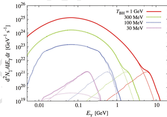
Figure 4.12.1: Gamma-ray instantaneous rate for BH at different temperatures. For each temperature, the curve with the peak to the right (left) represents the primary (secondary) component and the thick curve denotes their sum. The figure is a reproduction of Fig. 1 of Ref. [496].
