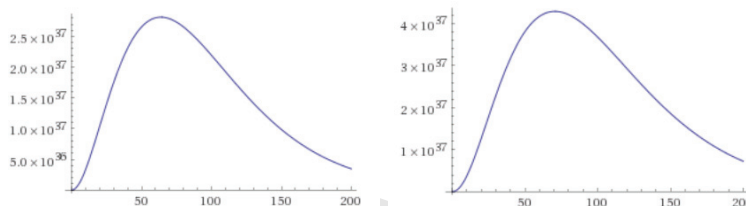
Figure 4.11.4: The differential axion rate from the supernova, dN_a/dE ( \text{GeV}^{-1} ), for a SN of 10 (left) and 18 (right) solar masses. The abscissa is in MeV.
