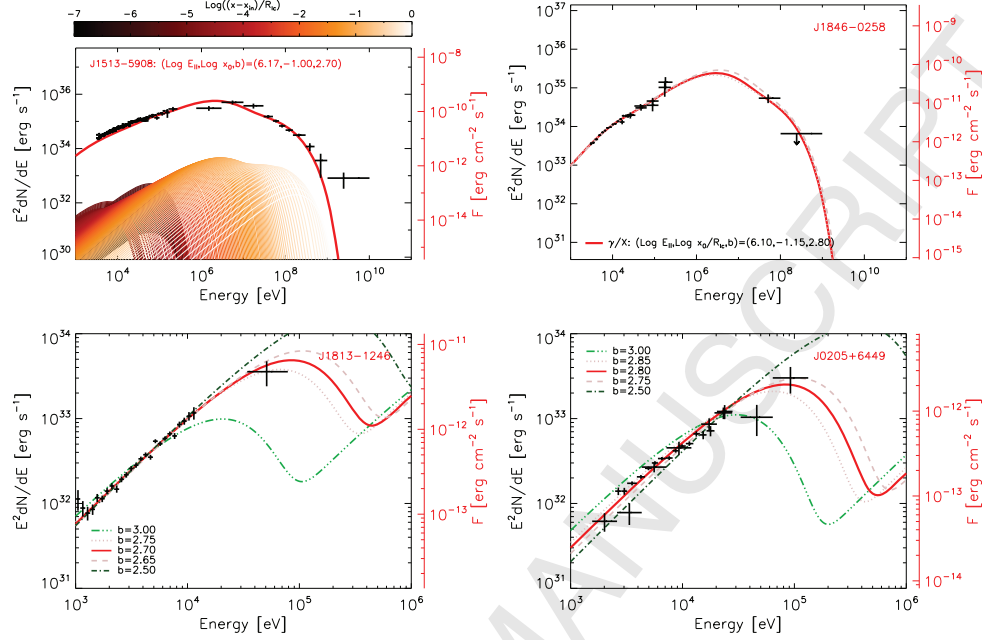
Figure 6.1.2: Top: Reproduced from corresponding panels in Fig. 1 and 2 of [629]. Model fitting for the 2 known MeV pulsars. See text for further comments. Bottom: Reproduced from corresponding panels of Fig. 2 of the Supplementary Material of [629]. These show examples of the spectral influence of the magnetic gradient ( b ) zooming out from X-ray to MeV energies. The different curves show the effect on variations on b around the corresponding best-fit one, keeping other parameters fixed at the best-fit solution.
