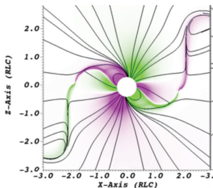
Figure 6.4.1: Current J \cdot B in a near-force-free magnetosphere. The pink/green color indicates current along/opposite the local magnetic field direction. Current flows out of the polar regions and in from the current sheet. From [663].
