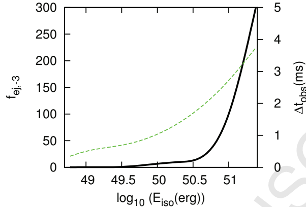
Figure 6.8.1: Expected e-ASTROGAM visibility window for vSGRBs. Lower energy bound for peak energy at E_p \sim 300 keV shows the upper region limit (black solid line) where detection with e-ASTROGAM is possible as a function of the logarithm of the isotropic equivalent energy released in the GRB. The left axis shows the fraction of the energy ejected in the outer crust, while on the right axis (dashed line) the duration of the expected signal is depicted (in ms).
