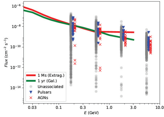
Figure 8.4.1: Flux of the unassociated sources, pulsars and AGNs detected by Fermi -LAT (3FGL) as a function of individual bands. The red and green curves are the e-ASTROGAM sensitivity for different integration times and for the energy range 0.03–3 GeV.
