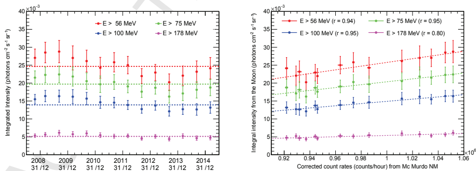
Figure 7.3.1: Left: time evolution of the lunar gamma-ray intensity above 56, 75, 100 and 178 MeV [764]. Right: study of the correlations between the lunar gamma-ray intensity [764] and the count rates of the McMurdo neutron monitor [770]. The values reported in brackets are the correlation coefficients.
