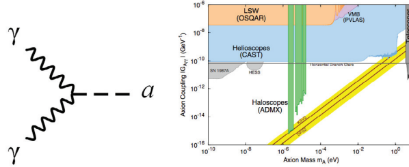
Figure 4.11.1: Left: Photon-photon-ALP vertex. Right: experimental limits on ALPs – the yellow line indicates standard axions.
