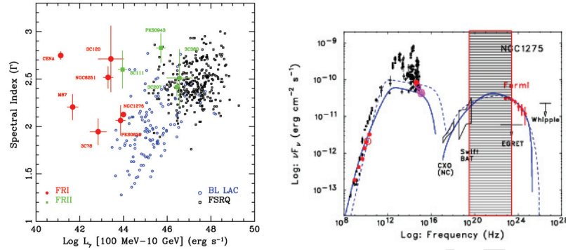
Figure 2.11.1: Left: Photon index vs. gamma-ray luminosity of MAGN and blazars detected by Fermi -LAT [207]. Right: SED of NGC 1275 from radio to TeV taken from [227]. The shaded area represents the energy range covered by e-ASTROGAM.
