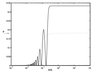
Figure 4.11.3: Oscillatory behavior around E_* for g_{a\gamma} = 0.33 \times 10^{-10} \text{ GeV}^{-1} , B = 0.5 \text{ nG} and N = 200 magnetic domains.
