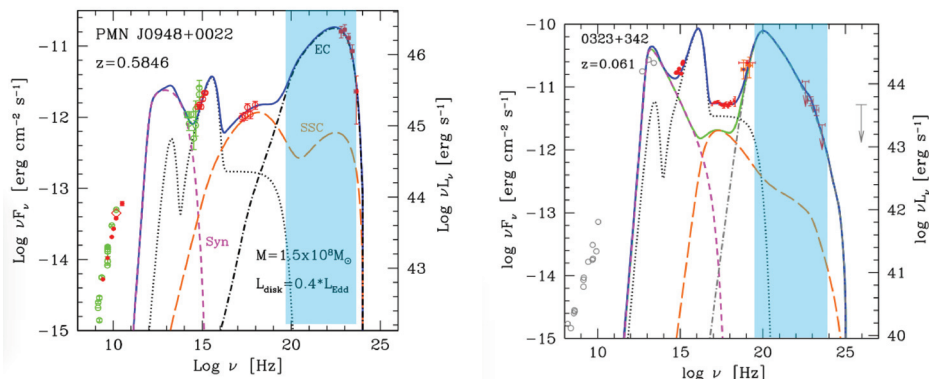
Figure 2.10.1: Left: SED of PMN J0948+0022 taken from [198]. The dotted line shows the contribution from the infrared torus and accretion disc. The SSC is shown in dashed and the IC from external photon fields (EC) is shown with a dot-dashed line. The blue area represents the energy range of e-ASTROGAM. Right: 1H 0323+342 is the closest among the gamma-ray emitting NLSy1. The SED is taken from [196]. The BH mass is assumed to be M_{BH} \sim 10^7 M_{\odot} and accretion disc luminosity of L_{disc} = 0.9L_{Edd} ([196]). Based on its characteristics in optical/X-rays, 1H 0323+342 seem to represent a transitional case in which the inner disc heats up and blows up to a torus configuration, as the accretion rate goes down ([197]).
