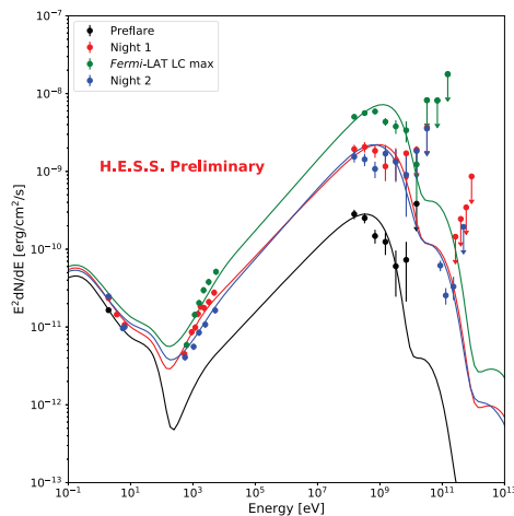
Figure 2.7.1: Multi-wavelength SED ( Swift -XRT, Fermi -LAT and H.E.S.S.) for different flux states superimposed with fits of an hadronic model. From [148].
