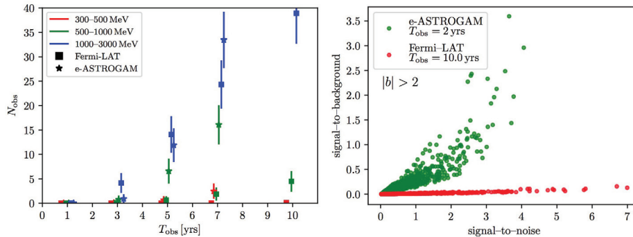
Figure 8.3.2: Projections for the detectability of the bulge MSP population. Left: Number of sources detectable with \text{SNR} > 5 as a function of total observation time in different energy ranges and for |b| > 2^\circ . We show predictions for T_{\text{obs}} \in [1, 3, 5, 7] yrs (minor shifts away from these values are for visibility). For Fermi -LAT we also include the 10 year prediction for comparison. Right: Signal-to-noise ratio (SNR) versus signal-to-background ratio (SBR) for a random realization of an MSP population that can reproduce the GCE in the energy range 0.5–1 GeV. We compare the current Fermi -LAT sensitivity (red) to that expected for e-ASTROGAM after 2 years of total exposure (green). Due to its larger exposure, the Fermi -LAT can reach a SNR comparable to e-ASTROGAM in this energy range, however, e-ASTROGAM has a superior SBR due to better angular resolution.
