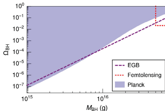
Figure 4.12.2: Compilation of PBH density bounds in the range 10^{15-17} g. The figure is a reproduction of Fig. 6 of [495].
