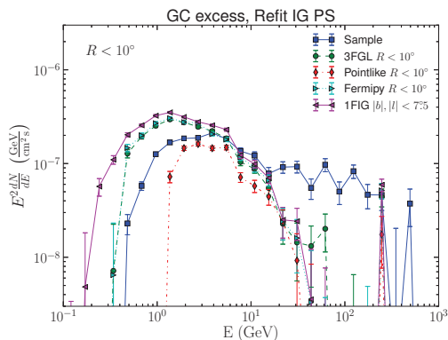
Figure 8.3.1: Effect on the spectrum of the GC excess from refitting of PS near the GC [833].
