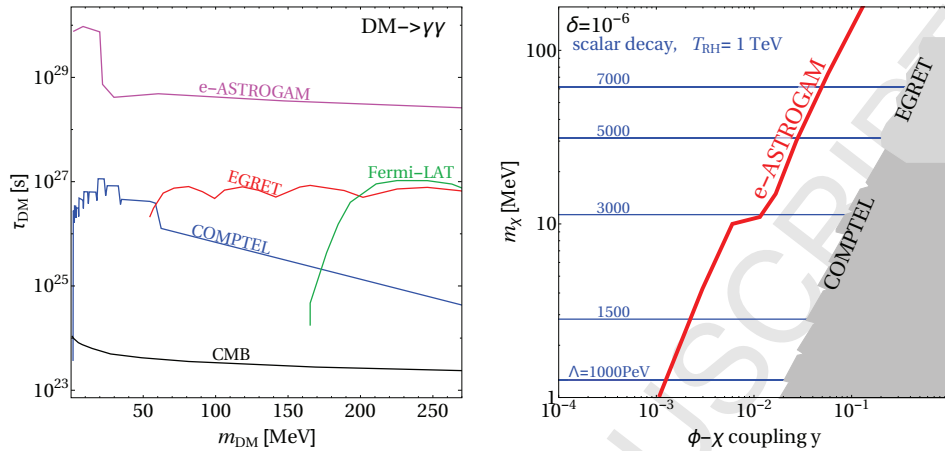
Figure 4.3.1: Left: Expected sensitivity of e-ASTROGAM to DM decay to photons (obtained by converting the limits on DM annihilation presented in [393] and Sec. 4.5), compared to existing constraints (based on [394]). Right: Expected e-ASTROGAM constraints on the parameter space of the DM model from Ref. [415].
