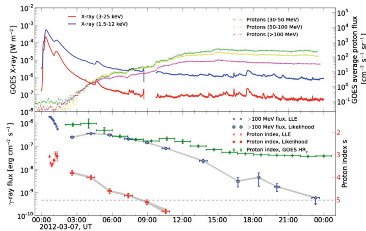
Figure 7.5.1: Temporal evolution of two bright X-class solar flares - 2012 March 7. (Top panel) X-ray emission and proton flux detected by GOES satellite. (Bottom panel) Long lasting gamma-emission detected by Fermi . Picture taken from [804].
