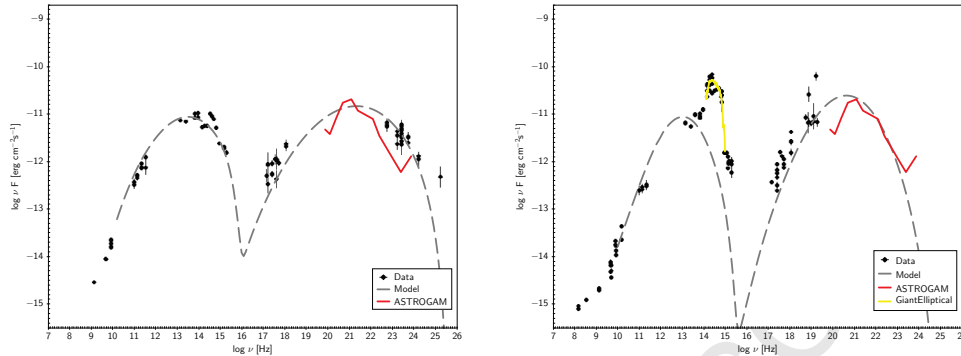
Figure 2.12.1: SEDs 1647+495 (left) and 1719+485 (right), that comprise multi-wavelength from the radio to the gamma-ray bands. The objects are representative of the class of low luminosity radio loud VLBL: (1) have the peak of synchrotron emission at low frequencies ( \nu_{\text{peak}}^{\text{sync}} < 10^{14} Hz), and for that reason their blazar nature appear disguised in the optical band, particularly when in the presence of a prominent host galaxy component; (2) they are core-jet VLBI sources, which is in general a good indication of alignment between the jet and the observer; (3) a fraction of these objects are gamma-ray sources. The dashed gray line represents the emission from SSC models, see text for details. The red line shows e-ASTROGAM sensitivity curve and in the case of 1719+485 an elliptical galaxy template is also shown in yellow. Data, templates and models (which are based on [236] and [237]) were obtained from SSDC website.
