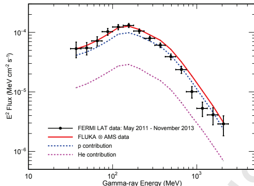
Figure 7.2.2: Comparison of the lunar gamma-ray flux measured by the Fermi -LAT in the period from May 2011 to November 2013 [764] with the predictions obtained by folding the fluxes of cosmic-ray protons and helium nuclei measured by AMS-02 [765, 766].
