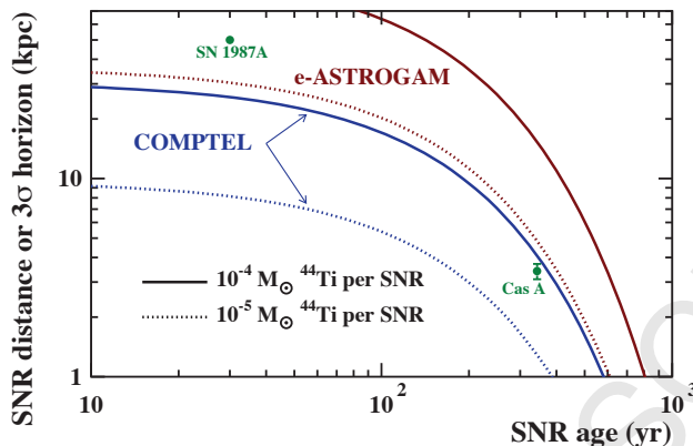
Figure 5.2.1: Horizon of detectability of the ^{44}\text{Ti} line at 1157 keV as a function of SNR age for CGRO/COMPTEL (blue lines) and e-ASTROGAM (red lines). The plotted sensitivities are for an effective source exposure of 1 year (COMPTEL: 9.0 \times 10^{-6} ph \text{cm}^{-2} \text{s}^{-1} ; e-ASTROGAM: 6.4 \times 10^{-7} ph \text{cm}^{-2} \text{s}^{-1} ), assuming two different yields of ^{44}\text{Ti} production per SNR: 10^{-5} M_{\odot} (common events; dotted lines) and 10^{-4} M_{\odot} (Cas A-like events; solid lines). Also shown are the age and distance of the two CCSNe with detected ^{44}\text{Ti} : SN 1987A and Cas A.
