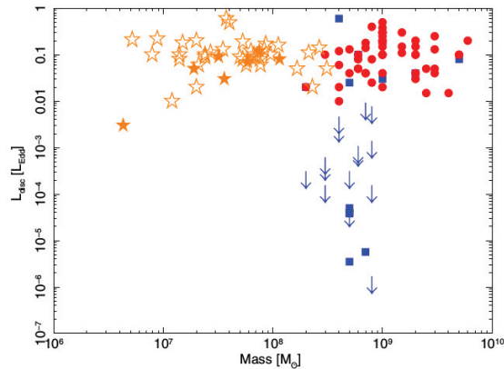
Figure 2.10.2: Accretion disc luminosity in Eddington units versus the mass of the central BH, taken from the survey study of [202]. The orange stars represent the characteristics of the radio-loud NLSy1 galaxies. The red circles show the FSRQs and the blue squares and arrows the BL Lac objects.
