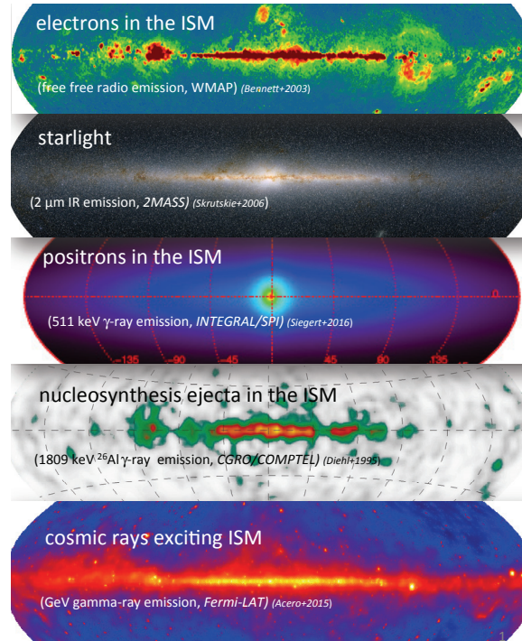
Figure 5.4.1: The diffuse emissions of our Galaxy across several astronomical bands: e-ASTROGAM will explore the link between starlight (second image from top) and CRs (top and bottom). The current-best images of positron annihilation (3rd from top) and ^{26}\text{Al} radioactivity (4th from top) gamma-rays illustrate that this link is not straightforward, and e-ASTROGAM will uncover more detail about the astrophysical links and processes. (Image composed by R. Diehl, from observations with WMAP, 2MASS, INTEGRAL , CGRO, and Fermi ; Refs. [7, 598, 599, 600, 601])
