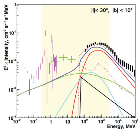
Figure 3.6.1: Spectrum of the inner Galaxy from [357, 306], including data from INTEGRAL /SPI (magenta and blue bars), COMPTEL (green crosses) and Fermi -LAT (black bars). The components are: pion decay (red line), IC (green line), Bremsstrahlung (cyan line), total (blue line), isotropic (black line), detected sources (magenta lower dashed line), detected sources plus total (magenta upper dashed line). The spectral coverage of e-ASTROGAM is highlighted in yellow. Its extended-source sensitivity for one year of observations based on simulations for the inner Galaxy is of the order of a few 10^{-5} \text{ cm}^{-2} \text{ s}^{-1} \text{ sr}^{-1} \text{ MeV} below a few MeV, increasing to 10^{-4} \text{ cm}^{-2} \text{ s}^{-1} \text{ sr}^{-1} \text{ MeV} around 10 MeV, and decreasing again to few 10^{-5} \text{ cm}^{-2} \text{ s}^{-1} \text{ sr}^{-1} \text{ MeV} above 30 MeV. This is a factor of \sim 30 - 10^3 below the interstellar intensity depending on the energy. The interstellar propagation model shown here is an example of standard models.
