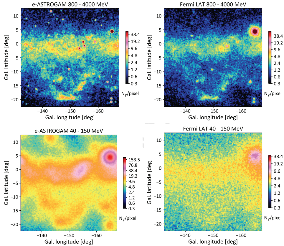
Figure 3.7.1: Photon count maps of the Galactic disc and Orion clouds in the 0.8-4 GeV (upper panels) and 40-150 MeV (lower panels) energy bands, simulated for e-ASTROGAM for one year of effective exposure (left panels) and compared to four years of Fermi -LAT data in scanning mode (right panels).
