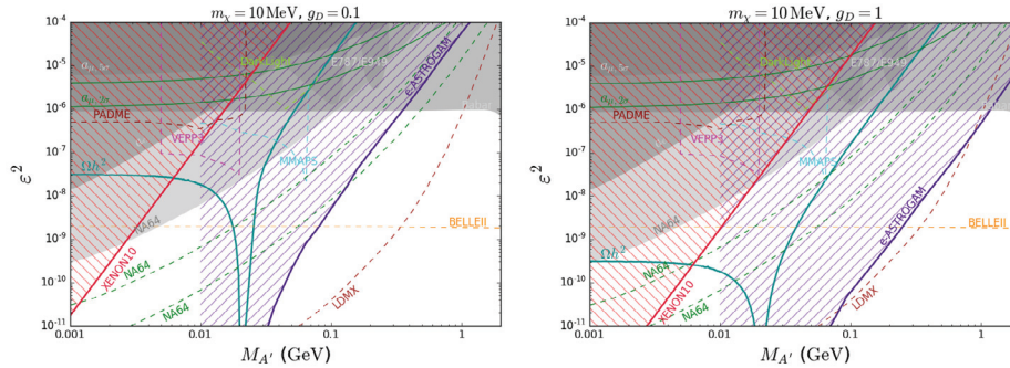
Figure 4.2.2: MeV DM complementarity : Bounds on the plane \varepsilon^2 versus dark photon mass. Direct detection and e-ASTROGAM exclusion regions are shown in red and purple hatched regions respectively. The correct relic density curve with turquoise lines for DM mass m_\chi = 10 MeV and two different values for the dark coupling g_D , g_D = 0.1 (left panel) and g_D = 1 (right panel). Existing (projected) bounds resulted from dark photon searches are displayed with gray regions (dashed lines).
