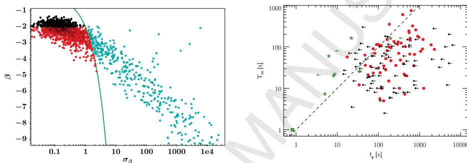
Figure 2.4.1: Left: high energy powerlaw spectral index \beta ( N(E) \propto E^\beta ) versus its relative uncertainty for the population of Fermi GRBs. The green line separates (leftward) GRBs with well constrained \beta (75% of the Fermi population) from (rightward) the GRBs with unconstrained \beta (25%). Right: GRB duration versus time of the fireball deceleration ( t_p ) both measured in the observer frame (Figure from Ghirlanda et al. 2017). Green symbols show the GRBs detected by LAT.
