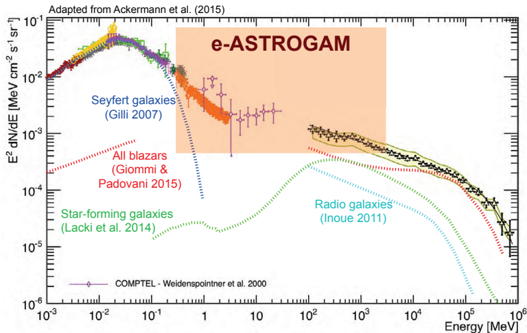
Figure 1.0.3: Compilation of the measurements of the total extragalactic gamma-ray intensity between 1 keV and 820 GeV [6], with different components from current models; the contribution from MeV blazars is largely unknown. The semi-transparent band indicates the energy region in which e-ASTROGAM will dramatically improve on present knowledge.
