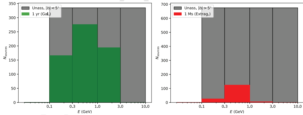
Figure 8.4.2: Left: Number of unidentified low galactic latitude sources from the 3FGL Catalog that would be detected by e-ASTROGAM for different energy intervals. Right: The same but for high galactic latitude sources.
