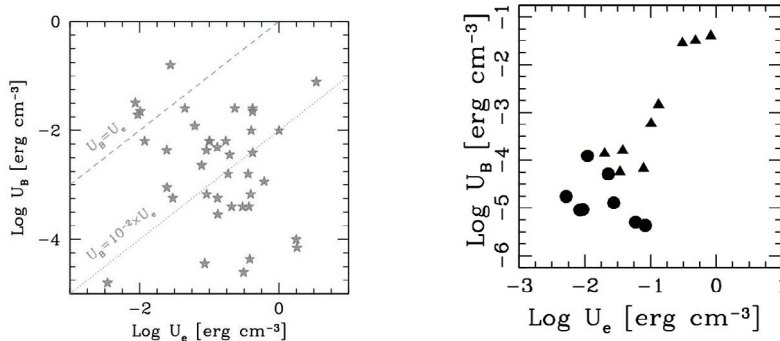
Figure 2.13.1: Left: Magnetic energy density and relativistic electron density estimated from SEDs of 45 BL Lac objects [240]. Right: Same, for Mrk 421 (triangles) and Mrk 501 (circles) in different activity states [241].
