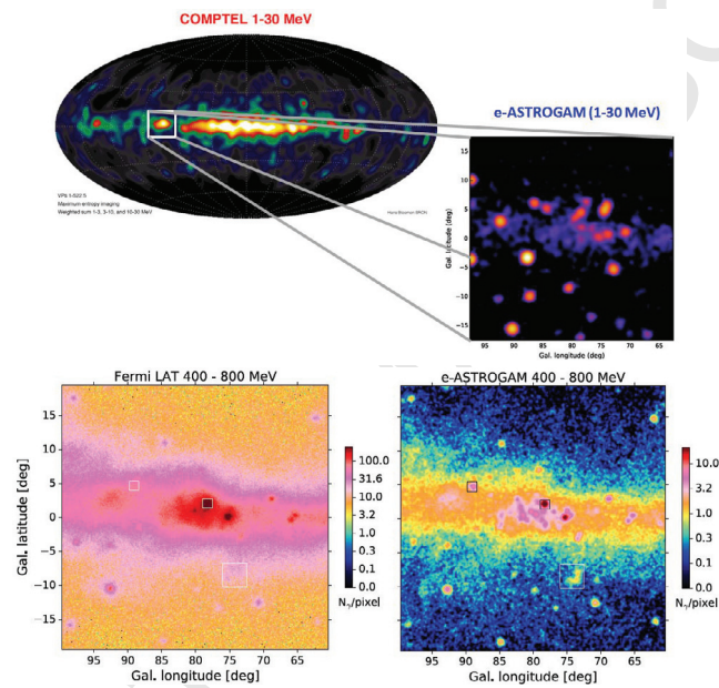
Figure 1.0.2: An example of the capability of e-ASTROGAM to transform our knowledge of the MeV-GeV sky. Upper panel: The upper left figure shows the 1-30 MeV sky as observed by COMPTEL in the 1990s; the lower right figure shows the simulated Cygnus region in the 1-30 MeV energy region from e-ASTROGAM. Lower panel: comparison between the view of the Cygnus region by Fermi in 8 years (left) and that by e-ASTROGAM in one year of effective exposure (right) between 400 MeV and 800 MeV.
