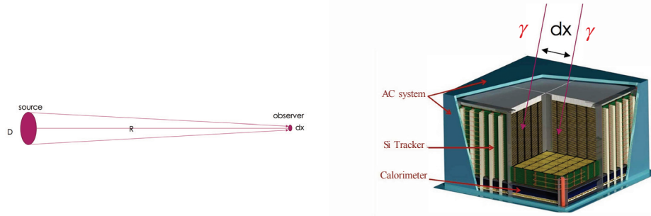
Figure 4.15.1: Left: Schematic relation between the source emitting region D and the observer, separated by a distance R ; dx is the photon separation in the observer frame. If dx < \lambda R/D , the pair of bosons are in the same state, and interference might occur. Right: A pair of coherent photon events impinging the detector, separated by a distance dx
