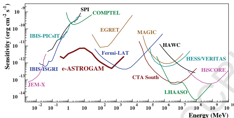
Figure 1.0.1: Point source continuum differential sensitivity of different X- and gamma-ray instruments. The curves for JEM-X, IBIS (ISGRI and PICsIT), and SPI are for an effective observation time T_{\text{obs}} = 1 yr, which is the approximate exposure of the Galactic center region accumulated by INTEGRAL since the beginning of the mission. The COMPTEL and EGRET sensitivities are given for the typical observation time accumulated during the \sim 9 years of the CGRO mission (see Fig. 1 in [5]). The Fermi -LAT sensitivity is for a high Galactic latitude source in 10 years of observation in survey mode. For MAGIC, VERITAS (sensitivity of H.E.S.S. is similar), and CTA, the sensitivities are given for T_{\text{obs}} = 50 hours. For HAWC T_{\text{obs}} = 5 yr, for LHAASO T_{\text{obs}} = 1 yr, and for HiSCORE T_{\text{obs}} = 100 h. The e-ASTROGAM sensitivity is calculated at 3\sigma for an effective exposure of 1 year and for a source at high Galactic latitude.
