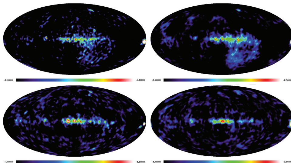
Figure 8.1.1: COMPTEL all-sky images using the current Maximum Entropy implementation. Galactic coordinates, centred on l = 0 , b = 0 . Left to right, top to bottom: 1-3 MeV, 3-10 MeV, 10-30 MeV, 1.8 MeV ^{26}\text{Al} line.
