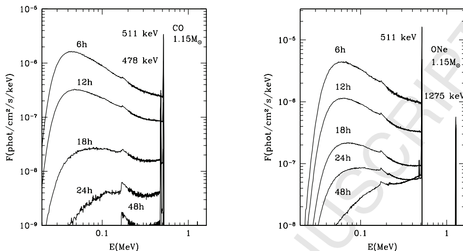
Figure 5.3.1: Gamma-ray spectra for (left) a CO nova and (right) a ONe nova of 1.15 M_{\odot} at different epochs after the outburst (defined as the peak temperature time) and at the distance of 1 kpc.
