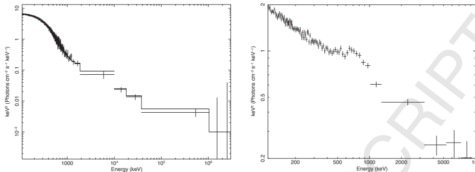
Figure 6.7.2: Left: Simulated 10^5 -s e-ASTROGAM average hard-state spectrum of Cyg X-1 assuming contributions from thermal Comptonization in the accretion flow at low energies and from synchrotron emission in a jet at high energies, as in Fig. 6.7.1. Right: Simulated 10^5 -s spectrum of an X-ray binary with a power law of \Gamma = 2.5 and a broad line from annihilation of e^\pm [716] at the temperature of kT \simeq 100 keV.
