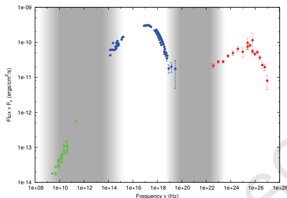
Figure 2.13.2: SED of Mrk 421 measured in multi-wavelength campaigns including Fermi and MAGIC telescopes [243]. The green circles corresponds to the radio emission from an extended region of the jet. The blue and red circles denote synchrotron and SSC emission respectively. The shaded area corresponds to the most appropriate frequency band, in order to constrain \gamma_{\min} .
