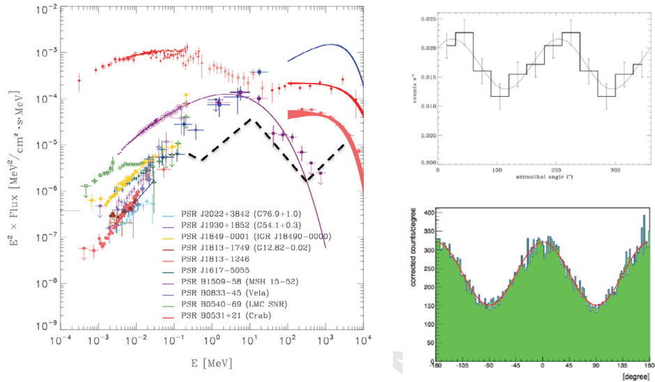
Figure 6.1.1: Left: SED for a number of soft gamma-ray pulsars taken from Kuiper & Hermsen [615] with the expected sensitivity for 1 Ms e-ASTROGAM exposure shown (black dashed line). Right: Comparison of the polarization sensitivity of INTEGRAL -IBIS (top) - observed Crab polarisation from 1 Ms observation (unpublished) vs e-ASTROGAM (bottom) for 1 Ms observation of a 100% polarised 10mCrab source in the 0.2 – 2 MeV range, see chapter 1. The spectral fit to the archetypal pulsar PSR B1509-58 is depicted by the purple curve.
