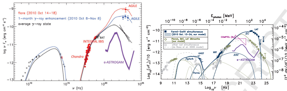
Figure 2.9.1: Left: Observed SED of the gravitationally lensed flat spectrum radio quasar PKS 1830–211 ( z = 2.507 ), built with archival data and Oct.-Nov. 2010 simultaneous data from the multi-wavelength campaign led by AGILE (models magnified by a factor of 10\times for the lensing). Adapted from [180]. Right: observed SED of PKS 1830–211 built with simultaneous LAT and Swift XRT and UVOT data, averaged over the Oct. 13–24, 2010 period of the multi-frequency campaign led by Fermi . Past 26-month LAT, 58-month BAT, Planck ERCSC, Gemini-N, Hubble -ST, Chandra and INTEGRAL IBIS [185], COMPTEL and EGRET data are also reported (corrected for lensing by a factor of 10\times ). Adapted from [181]. This study is an example of a possible future confluence in e-ASTROGAM of synergetic legacy science from teams of Fermi , AGILE and INTEGRAL missions.
