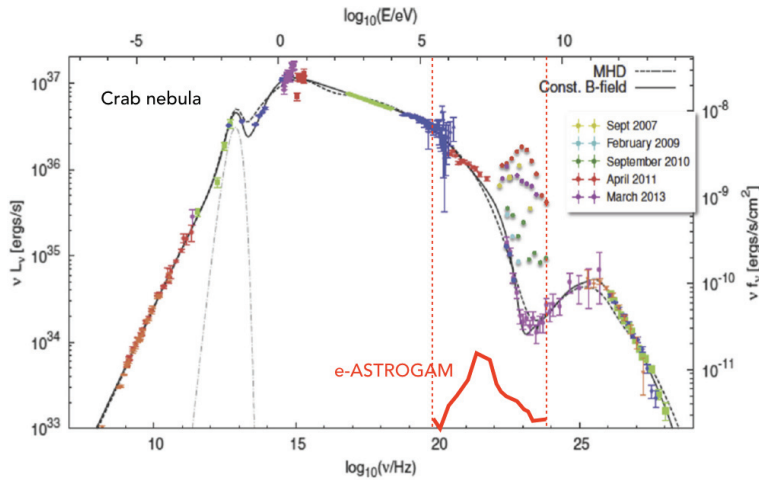
Figure 6.5.1: SED of the Crab nebula from the radio to VHE gamma-rays, also showing the flares. The sensitivity of e-ASTROGAM (red curve) is given for one year of effective exposure in the Galactic disk. Adapted from [672, 675].
