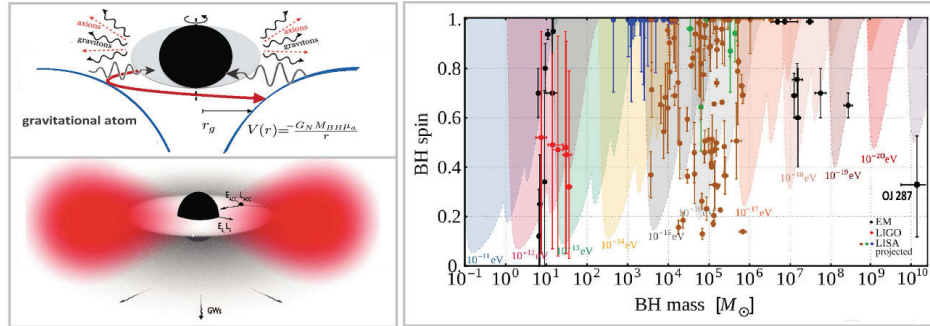
Figure 4.13.1: Left: cartoon of the bosonic gravitational atom (axion, red, cloud bound to a Kerr BH). E, L is the energy/angular momentum lost through superradiant scalar waves and GWs (S) or transported in the accretion disc (ACC). The material is in free fall after the innermost stable circular orbit (ISCO). Adapted from [508]. Right: Exclusion regions in the Regge plane for a massive boson field. Black points: BH spin from e.m. estimates (X-ray K_\alpha or ISCO-based fits). The OJ 287 value is obtained trough optical variability clocking [512]. Red data: LIGO detections GW150914, GW151226, GW170104. Blue/green/brown data: projected LISA. Adapted from [509].
