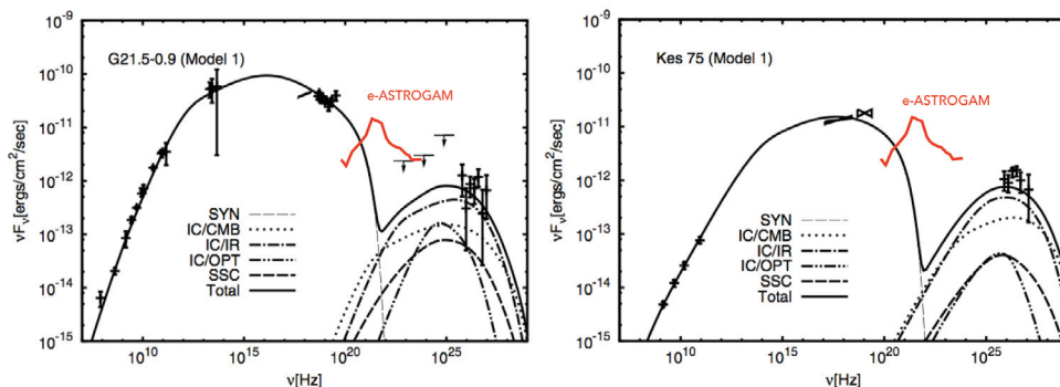
Figure 6.5.2: Spectra and models for PWN G21.5-0.9 and Kes75 from [679]. The sensitivity of e-ASTROGAM (red curve) is given for one year of effective exposure in the Galactic disk.
