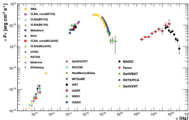
Figure 2.8.1: Overall SED of the TeV blazar Mkn 421. Multi-wavelength observations of the source emission, from radio to TeV energies, allowed for an accurate measurement of the acceleration mechanisms of the electrons in the jet [167]. In this HBL object the synchrotron emission lies in the optical/soft X-ray energy range. Therefore, the synchrotron peak of the source could be precisely determined and modeled.
