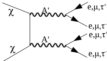
Figure 4.9.2: Feynman diagram for DM annihilation into lepton final states.
