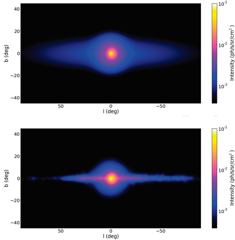
Figure 5.5.1: Simulated e-ASTROGAM observations of the 511 keV emission, obtained for an exposure of 1 year of the inner Galactic region, assuming (top) the model proposed by [600] with a thick disk and (bottom) a model with the disk of [613] and the point source and bulge components of [614].
