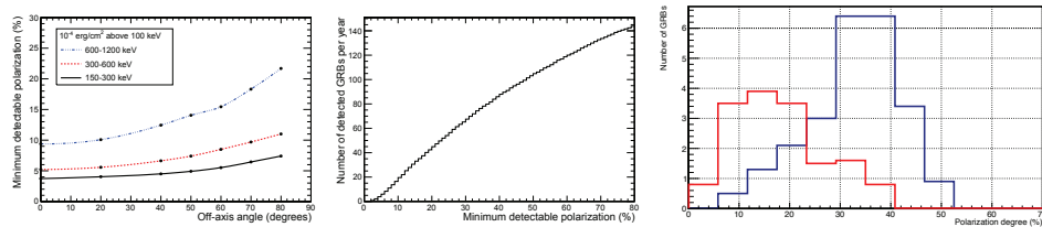
Figure 2.3.2: Left: Minimum polarization fraction detectable by e-ASTROGAM in three energy bands as a function of the off-axis angle. Centre: Cumulative number of GRBs to be detected by e-ASTROGAM as a function of the MDP. Right: Expected measured distribution of polarization degrees achieved using 1 year of data for the photospheric emission model (red) and the synchrotron with highly ordered magnetic field model (blue).
