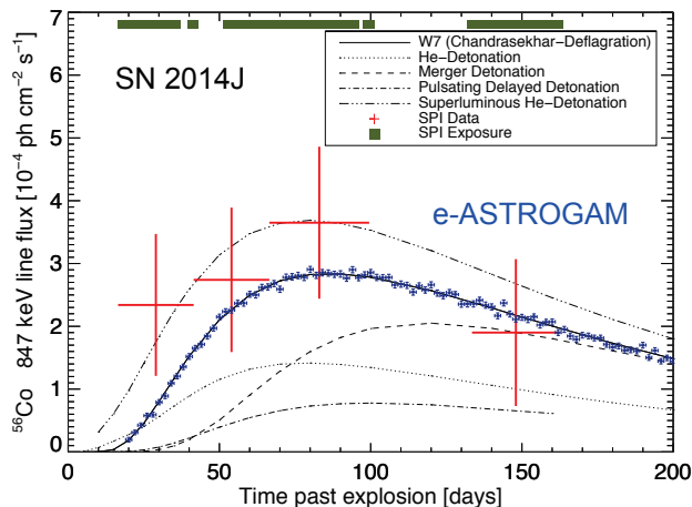
Figure 5.1.2: Light curve of the 847 keV line from ^{56}\text{Co} decay in SN 2014J. INTEGRAL data (adapted from Fig. 4 in Ref. [548], red data points) are compared to various models of Type Ia SN [555]. A simulation of the e-ASTROGAM response to a time evolution of the 847 keV line such as in the W7 model [553] shows that the sensitivity improvement by e-ASTROGAM (blue points) will lead to a much better understanding of the SN progenitor system and explosion mechanism.
