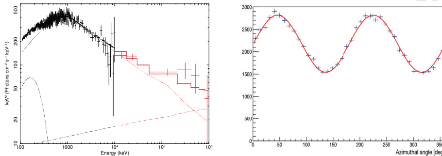
Figure 2.3.1: e-ASTROGAM spectra (left) and 0.1-1 MeV photon modulation with polarization angle in degrees (right) expected for a 100% polarized GRB 080916C.
