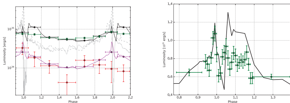
Figure 3.2.1: Left: Simulated and observed X-ray and gamma-ray light curves of \eta Carinae through two periastron passages. The green and red points show the observed Fermi -LAT light curves at low (0.3-10 GeV) and high (10-300 GeV) energies. The dim grey light curves show the observed (continuous) and predicted (dash, without obscuration) thermal X-ray light curves. The black and purple lines and bins show the predicted IC and neutral pion decay light curves. Right: A merged Fermi -LAT analysis (0.3-10 GeV) of the two periastrons for narrower time bins.
