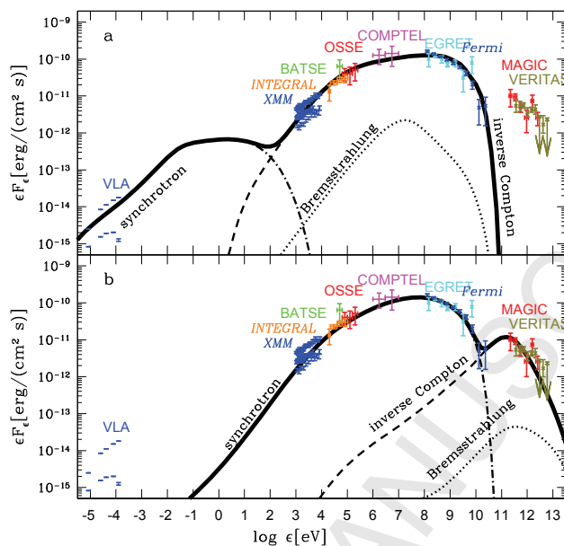
Figure 6.6.1: The broad-band spectrum of the gamma-ray binary LS I +61 303 modelled by two variants of the model of the pulsar-wind/stellar-wind interaction [688]. (a) The model in which the soft and HE gamma-rays are dominated by Compton scattering. (b) The model in which the soft and HE gamma-rays are dominated by the synchrotron process.
