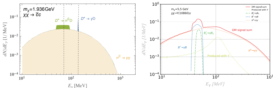
Figure 4.4.1: Left: Example of the expected gamma-ray spectrum for DM annihilation into charm quarks, with a DM mass m_\chi just above the kinematic threshold to produce D -mesons. The sharp spectral features result from the indicated meson transitions, while the background is mostly due to \pi^0 \rightarrow \gamma\gamma . For more details, see Ref. [416]. Right: Gamma-ray spectrum from DM annihilation through the quarkonium channel \chi\chi \rightarrow \Upsilon(10860)\gamma . The three visible spectral features are due to two different meson transitions and the photon produced in conjunction with the quarkonium. For more details, see Ref. [425].
