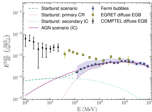
Figure 3.4.1: Fermi Bubbles spectrum compared to the AGN (leptonic IC, solid purple line) and starburst (hadronic, dashed green line) models of the gamma-ray emission [324]. The shaded band shows the systematic uncertainty on the FB spectrum [324]. The hadronic model includes the primary emission (dotted red line) of gamma-rays and the gamma-rays produced in IC interactions of secondary electrons and positrons (dash-dotted cyan line). The secondary component of gamma-ray emission in the hadronic model is significantly softer than the primary component which results in a break around 30 MeV and a significant difference between the hadronic and leptonic models of gamma-ray emission around a few MeV. For comparison, we also plot the diffuse extragalactic gamma-ray background (EGB) fluxes measured by the EGRET [329] and COMPTEL [330] experiments.
