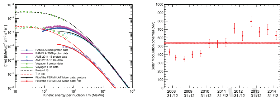
Figure 7.3.2: Left: CR proton and helium spectra obtained from the best fit of the Fermi -LAT Moon gamma-ray data [764]. The results of the fit (continuous black and red lines) are compared with the proton measurements taken by PAMELA [776] in 2008 (blue points) and 2009 (purple points) and with the AMS-02 [765, 766] proton (cyan points) and helium data (violet points). The plot shows also the proton and helium LIS (dashed black and red lines) and the Voyager 1 proton (light green points) and helium (dark green) data [777]. Right: Time evolution of the solar modulation potential, evaluated from a fit of the lunar gamma-ray emission. The central band corresponds to the average value of the solar modulation potential during the whole data-taking period.
