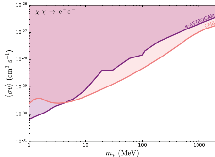
Figure 4.2.1: Model independent limits on the DM annihilation cross section as a function of the DM mass, m_\chi , based on the existing CMB data (red curve) [408] and the e-ASTROGAM mission (purple curve) [393]. It is visible that e-ASTROGAM will furnish limits competitive to those from the CMB and have the potential to discover DM below \sim 10 MeV. See [409] for details.
