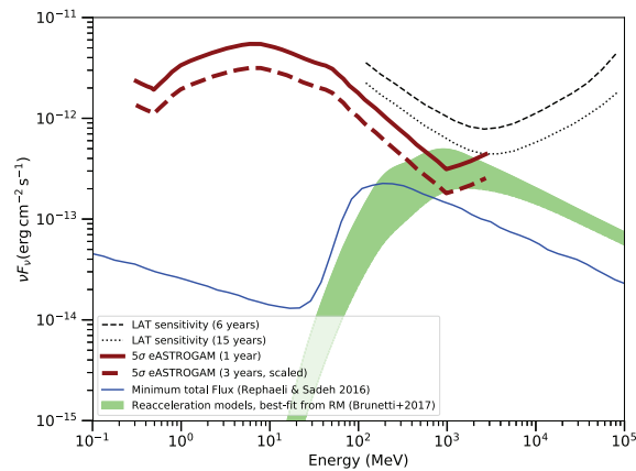
Figure 2.15.1: Predicted gamma-ray spectra for viable models of energetic electrons and protons in clusters, based on various cluster dynamical, intracluster gas, and magnetic field properties. The blue curve shows the minimal level of the total emission predicted in the model based on the assumption that particles originate in star-forming galaxies and the two dominant radio galaxies in the cluster core (without re-acceleration) [267]. Predicted emission in turbulent re-acceleration models assuming various values of the acceleration time and duration of the acceleration period [269] are shown by the green-colored region. Black lines correspond to the sensitivity of Fermi -LAT (solid for 6 years, dashed for 15 years, respectively). The bold red curves are the same as in Chapter 1, for 1 year (solid) and 3 years (dashed). The figure is based in part on a similar figure in [269].
