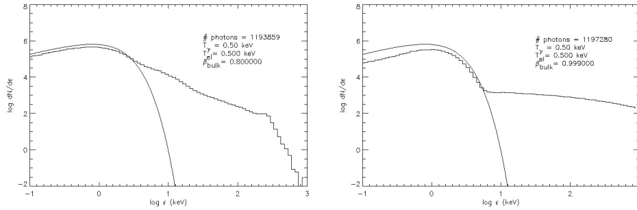
Figure 6.3.2: Monte Carlo simulations of RCS spectra emerging from a globally twisted magnetosphere for different values of the bulk electron velocity, \beta = 0.8 , left, and \beta = 0.999 , right [654].
