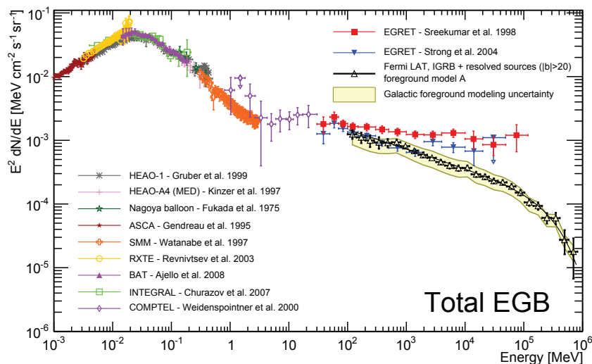
Figure 2.14.1: Spectrum of the high-energy background from X-ray to TeV gamma-rays. Adapted from [259].
