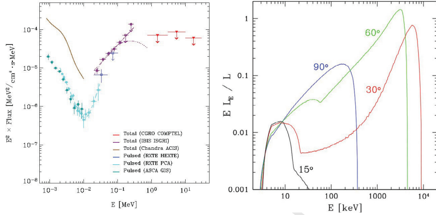
Figure 6.3.1: Left: The observed SED of the AXP 4U 0142+614 [653]. Right: RCS model spectra from a localized j-bundle at different viewing angles with respect to the magnetic axis [652].
