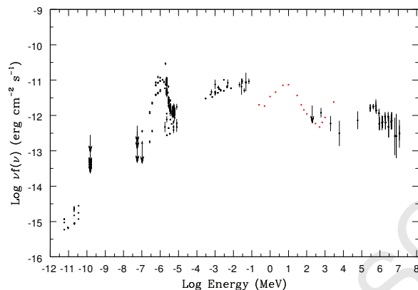
Figure 2.8.2: SED of the extreme blazar 1ES 0229+200 (black markers). In this case, the peak of the synchrotron emission is not well determined due to the lack of measurements at frequencies above 100 keV. The 1-year sensitivity of e-ASTROGAM is plotted with red markers. Adapted from SSCC website.
