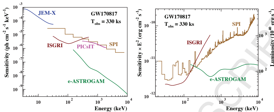
Figure 2.1.1: Left: Continuum and (b) narrow-line sensitivities reached in the INTEGRAL targeted follow-up observation of GW170817, compared to the corresponding sensitivities of e-ASTROGAM. All sensitivities are shown for a total exposure of 330 ks. The luminosity units of the panel on the right assume a distance to the source of 40 Mpc. Adapted from Figs. 5 and 6 of Ref. [49].
