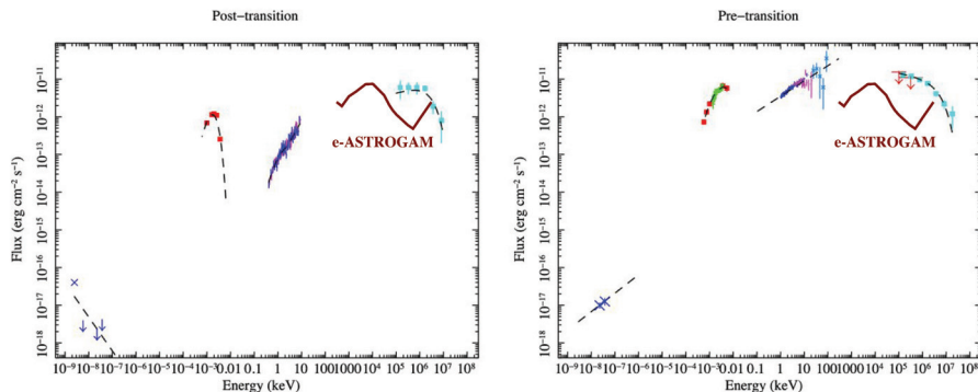
Figure 6.2.1: Broadband SED of XSS J12270–4859/PSR J1227–4853 during RPP state (left) and LMXB state (right), taken from [644]. The one-year sensitivity of e-ASTROGAM is added to each panel. This tMSP would be detected with high significance by e-ASTROGAM in either state, and in particular the spectrum from a long-lasting LMXB phase might be detectable across the full science range.
