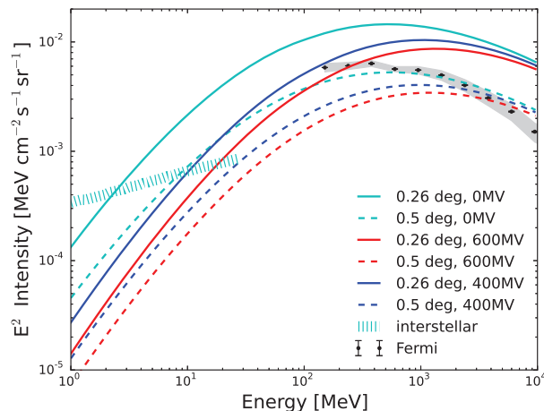
Figure 7.4.1: Predictions of the intensity of the solar IC emission for the energy range of e-ASTROGAM for various models and various angular distances from the Sun [795]. The figure shows also the Fermi -LAT data [788] and predictions of the interstellar emission at intermediate latitudes for comparison [356]. The figure is taken from [795].
