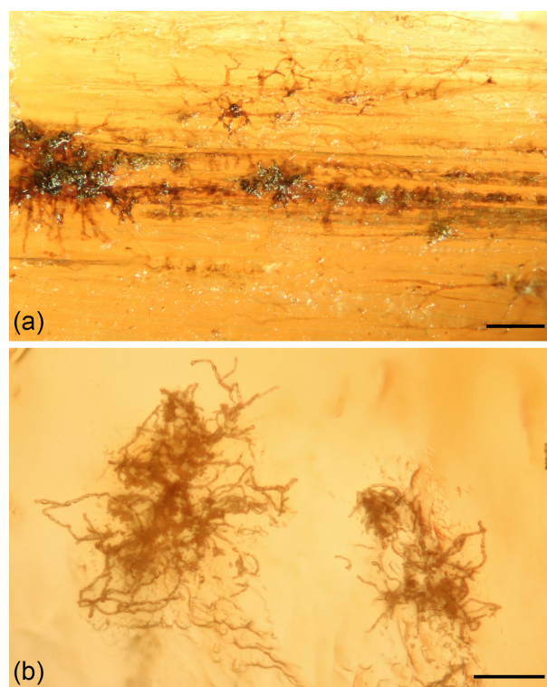
Figure 5. Dematiaceous hyphomycetes growing on naturally occurring resin pieces of Araucaria columnaris in New Caledonia. (a) Mycelium and (b) branched hyphae partly being submerged in resin. Scale bars: 50 µm.
