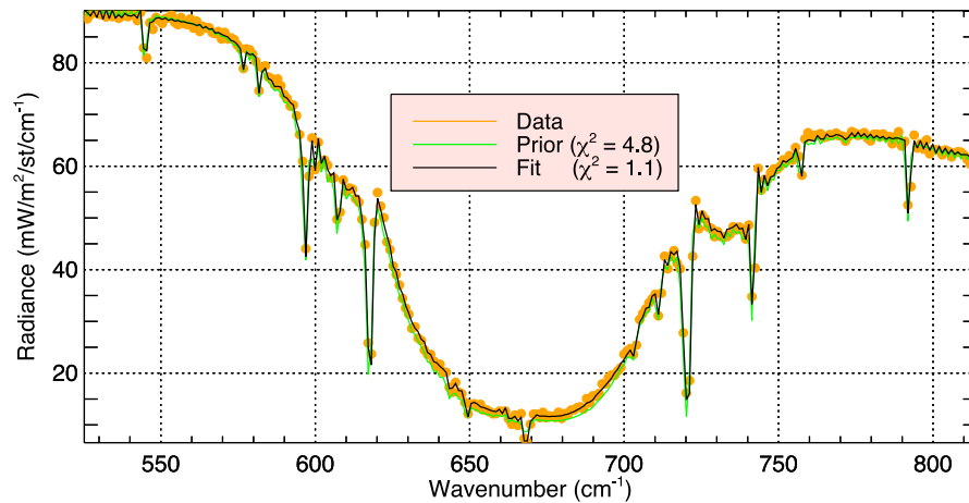
Fig. 10. Forward modeling of the TIR1 spectra for orbit 205, SYN spectrum #8.
