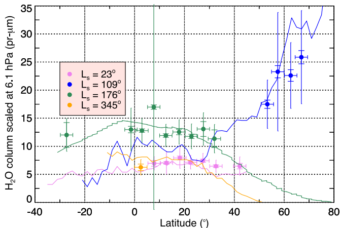
Fig. 21. (Left) zonal average of scaled H_2O column abundances obtained for parametric TIR estimation including or (Right) not including the simultaneous retrieval of the atmospheric temperature. As in Fig. 18, the inner error bars represent the statistical uncertainty, the outer error bar show the quadratic sum of statistical uncertainty and standard deviation in the latitudinal bin. The lines display the scaled column abundances extracted from Trokhimovskiy et al. (2015).
