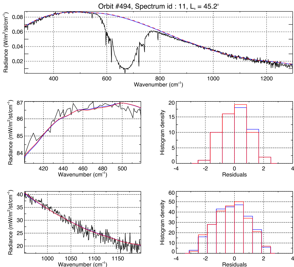
Fig. 5. A typical fit of PFS data in the TIR3 band where surface temperature and dust optical depth are retrieved, blue: without scattering, red: full transfer with scattering. The values of the parameters are a DOD of 0.18 at 9\text{ }\mu\text{m} , an effective dust radius of 1.5\text{ }\mu\text{m} and a surface temperature of 253.2\text{ K} . The bottom plots zoom over the two edges of the TIR3 domain and display the corresponding histogram of the residuals given in %.
