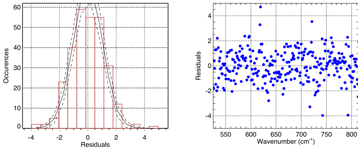
Fig. 11. Residual (differences between data and model divided by the radiometric noise at 1-σ) distribution corresponding to the fit displayed in Fig. 10.
