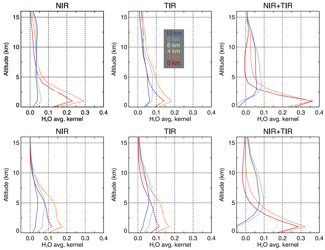
Fig. 23. Averaging kernels (see (8)) for NIR, TIR and NIR + TIR setups obtained in a dry (upper line of plots) and a wet (lower line of plots) configuration. Only the kernels computed for the altitude located at and below 10 km (see legend) are shown for the sake of clarity.
