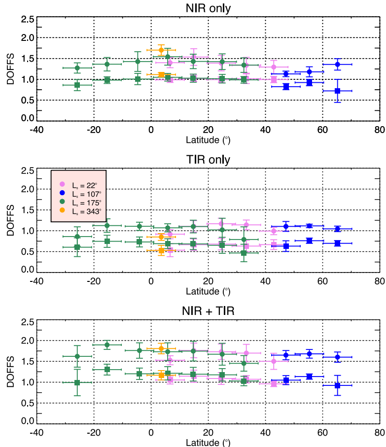
Fig. 26. (Upper) Zonal averages of H_2O DOFFS in the NIR. (Middle) TIR and (Lower) NIR + TIR cases for the total column (filled circle) and up to 5 km above the surface (filled square). The error bars give the standard deviation in the considered latitude/ L_s bin.
