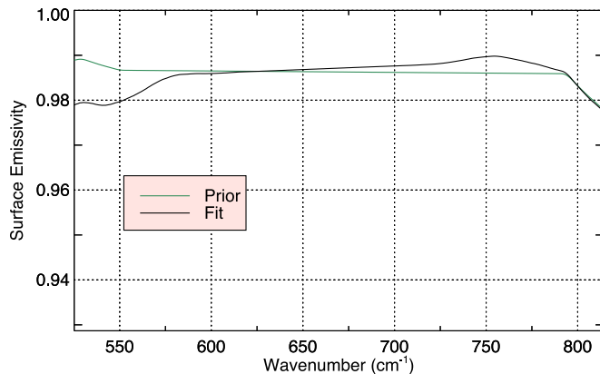
Fig. 12. Retrieval of the spectral emissivity in the TIR1 band corresponding to the fit displayed in Fig. 10.
