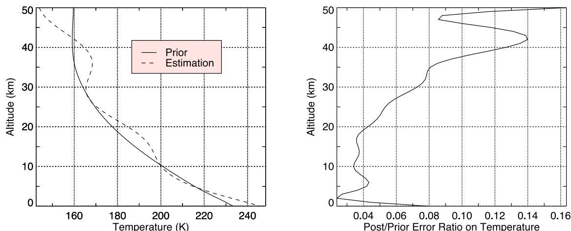
Fig. 13. (Left) Retrieval of the temperature profile. The prior corresponds to the MCD predictions for the spectra of Fig. 10. (Right): Error reduction factor on the atmospheric temperature parameters.
