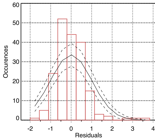
Fig. 20. Residual (expressed in %) distribution corresponding to the fit displayed in Fig. 19.
