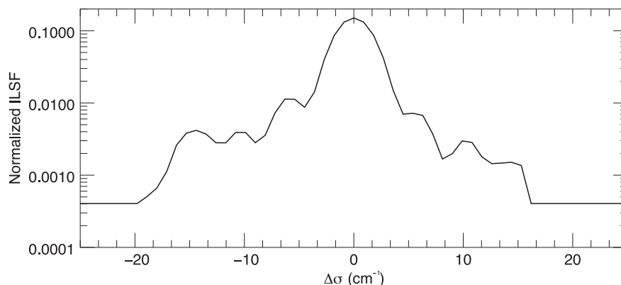
Fig. 1. The normalized instrument line shape function as it appears at the central wavenumber of the NIR band used throughout this study.
