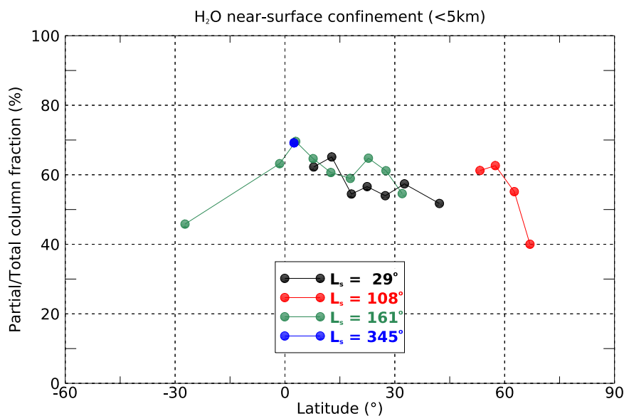
Fig. 28. Plot showing the relative vertical partitioning of water as deduced from the NIR + TIR synergetic method. The quantity displayed, expressed in %, is the 5-km partial column ratioed with the total column abundance of water. Higher ratio values indicate stronger confinement of water near the surface.
