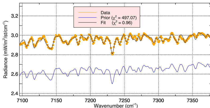
Fig. 14. Modeling of a NIR spectrum for orbit 1485, SYN spectrum #1. The estimated column abundance is 25 \pm 2 pr- \mu\text{m} .
