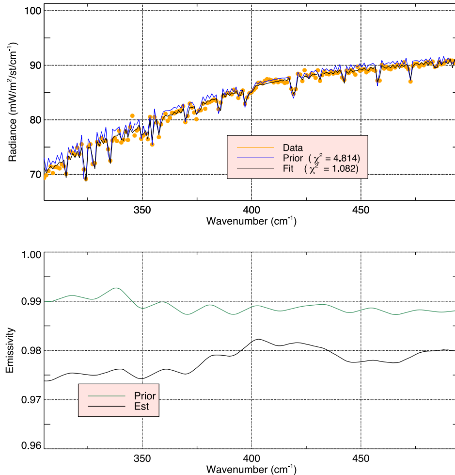
Fig. 19. (Top) simulated TIR2 spectra for orbit 1040 (SYN spectra #2). (Bottom): Result obtained after the inversion of the continuum.
