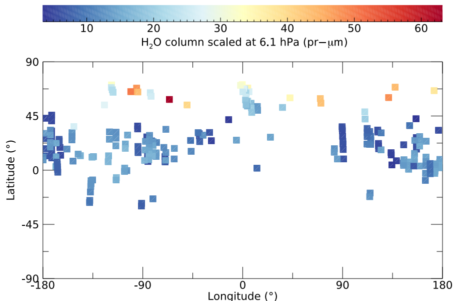
Fig. 17. Map of retrieved \text{H}_2\text{O} column abundances scaled at 6.1 hPa. TIR-only inversion.
