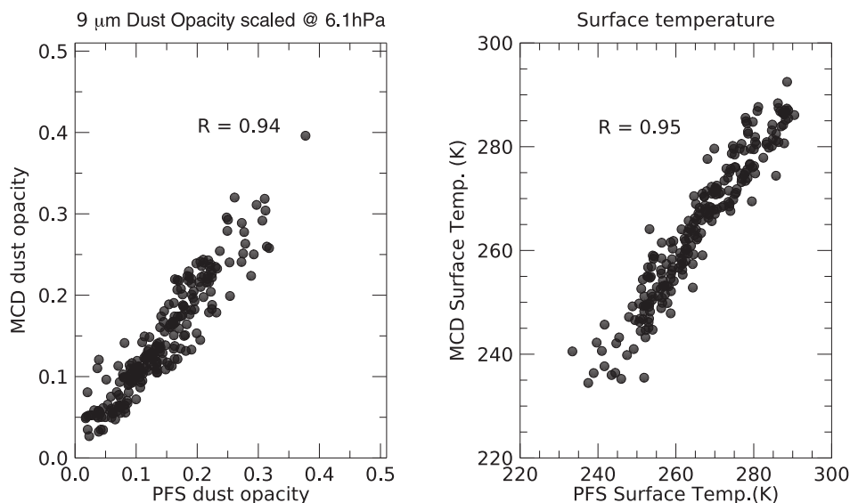
Fig. 9. Retrievals of DOD without scattering (left) and of the surface temperature (right) from PFS data and compared to the predictions of the MCD. Correlation coefficients (R) between PFS and MCD datasets are given in the plots.
