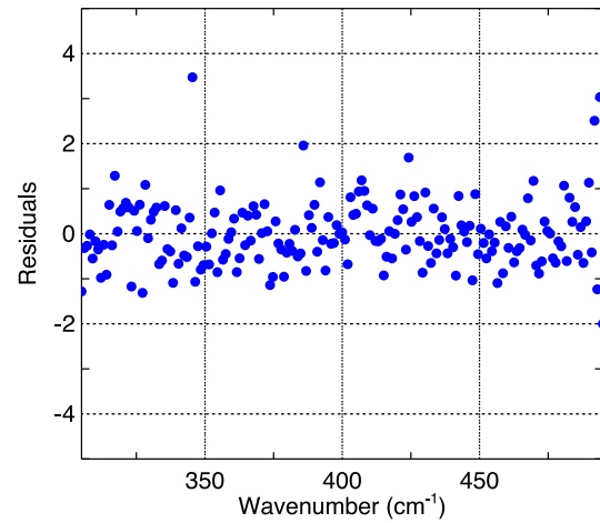
Fig. 20. Residual (expressed in %) distribution corresponding to the fit displayed in Fig. 19.
