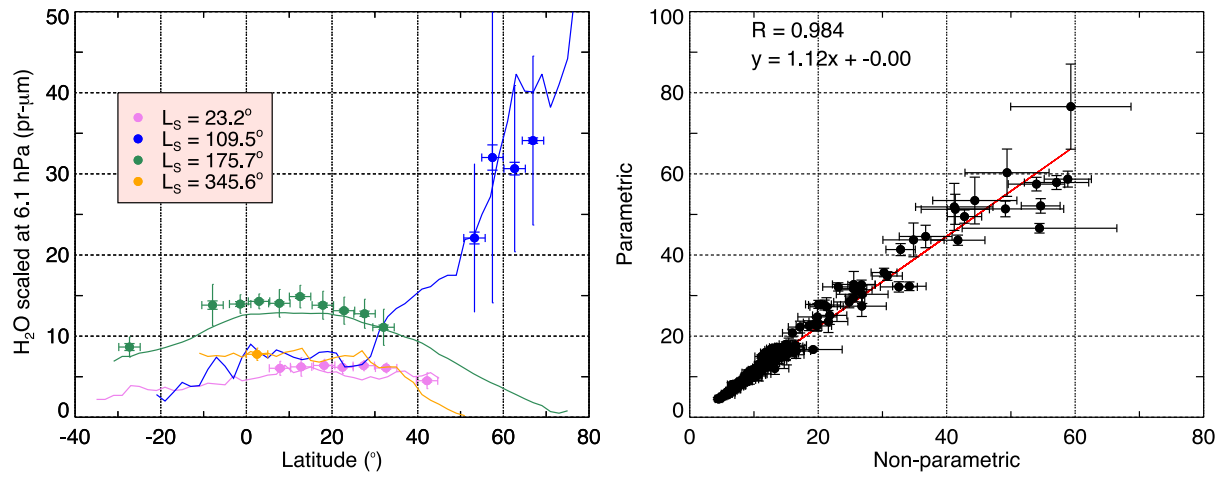
Fig. 18. (Left) zonal average of scaled H 2 O column abundances obtained for a parametric inversion. The inner error bars represent the statistical uncertainty, the outer error bar show the quadratic sum of statistical uncertainty and standard deviation in the latitudinal bin. The lines display the scaled column abundances extracted from Trokhimovskiy et al. (2015). (Right) scatter plot of the column abundances corresponding to parametric and non-parametric inversions. Statistic error bars on column abundances are ~6 and 10% on average in the parametric and non-parametric cases respectively.
