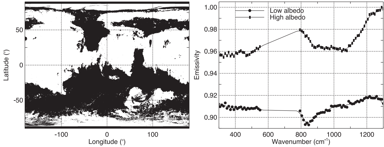
Fig. 3. Left: dark/bright region mask built from the TES albedo map. High albedo ( >0.18 ) regions appear in white, low albedo in black. Right: the symbols display the spectral emissivity for dark and bright regions obtained from TES data. The lines show the interpolations used in the forward model.
