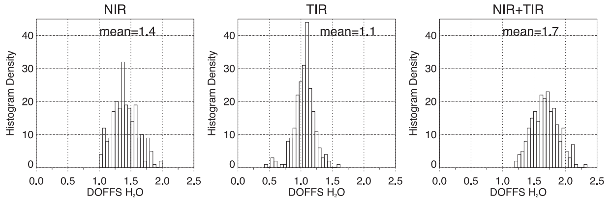
Fig. 25. DOFFS for water vapor profile obtained in the NIR, TIR and NIR + TIR cases.
