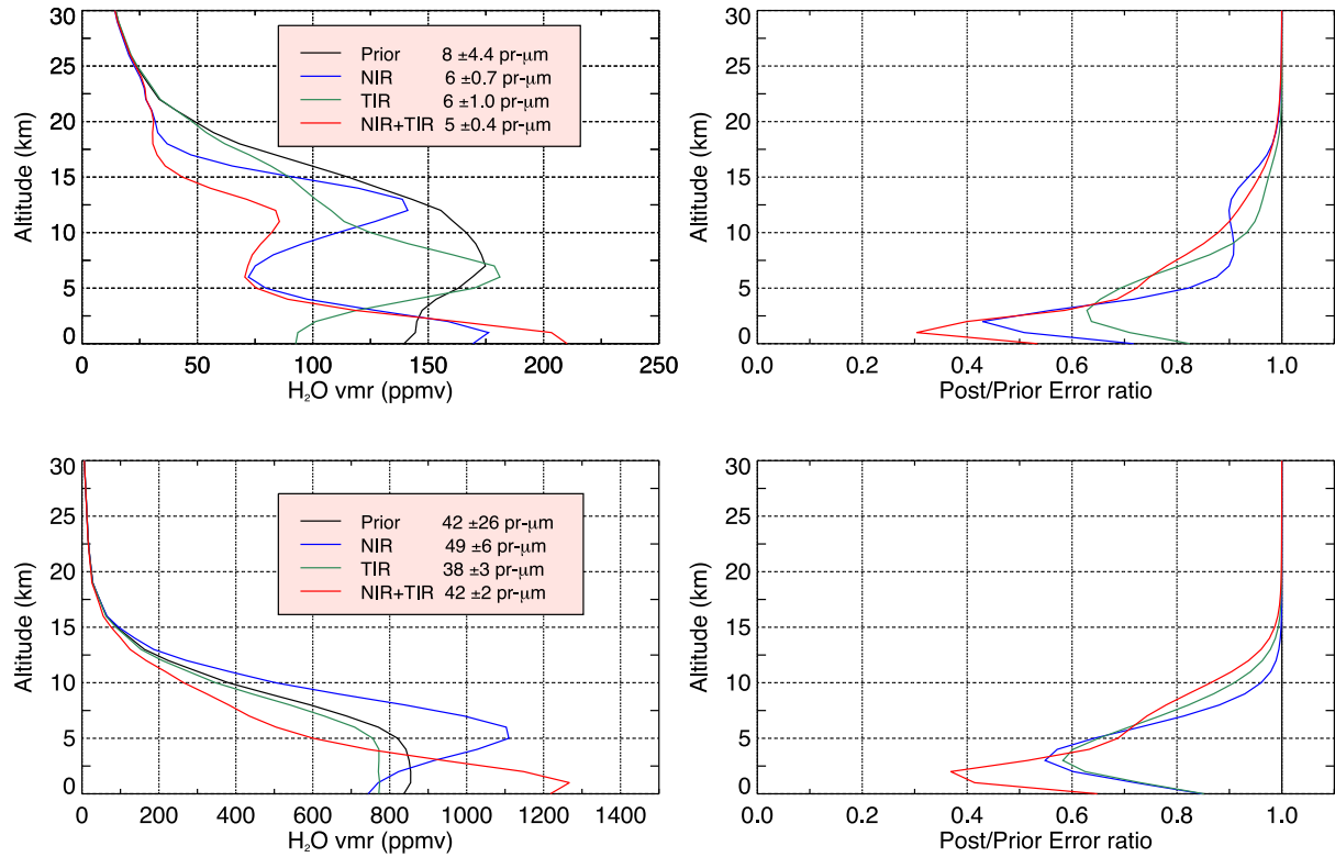
Fig. 24. (Left) H 2 O vmr estimations vs. altitude. The retrieved column abundances are given in the legend box for all the types of inversion, compared to the prior estimate. (Right) post. to prior uncertainty ratio vs. altitude. The upper figures are for the “dry” atmosphere case, while the lower figures concern the “wet” atmosphere case.
