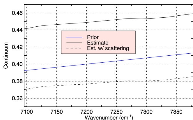
Fig. 16. Continuum retrieval corresponding to the fit displayed in Fig. 14. The solution found while accounting for scattering is shown as well (DOD = 0.08, mean radius = 1 \mu\text{m} ).
