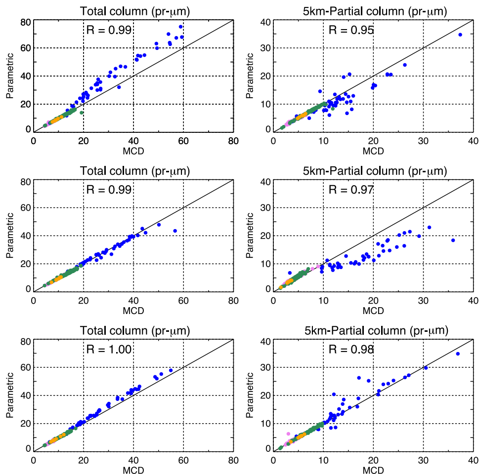
Fig. 27. Comparison between total (left) and partial (right) column abundances obtained using a parametric or a predicted (MCD) 1st guess of the water vapor profiles. From top to bottom: NIR, TIR, NIR + TIR cases. On each plot the value of the linear correlation factors, R , are indicated. The color code is the same as in Fig. 26.
