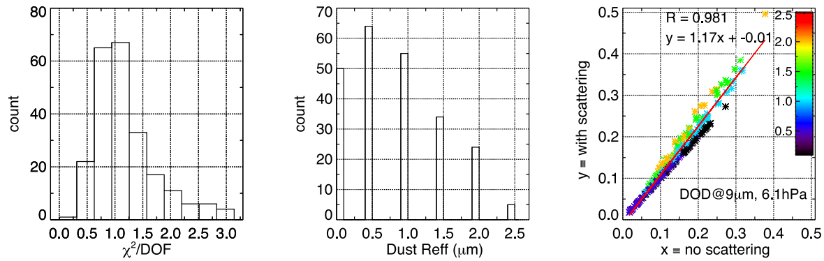
Fig. 6. (From left to right) reduced \chi^2 , number of occurrences of the dust effective radius, correlation between the DOD obtained with scattering (y-axis) and the DOD obtained without scattering (x-axis). Color is coded according to the effective radius value. DOD values are normalized to a reference pressure of 610 Pa.
