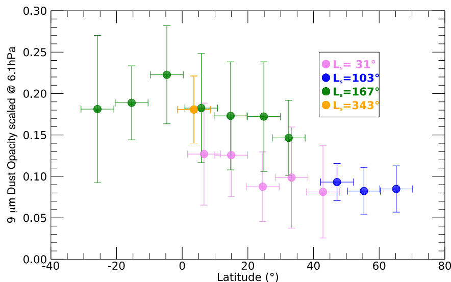
Fig. 8. Zonal averages of normalized DOD. The error bars correspond to the standard deviation within the latitude/solar longitude bin.
