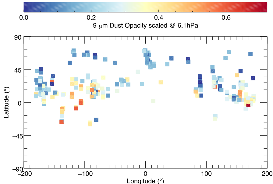
Fig. 7. Map of DOD scaled at 610 Pa and derived without accounting for scattering from the PFS data.
