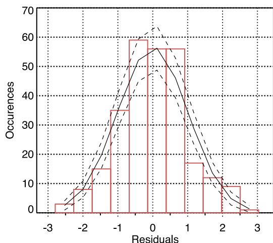
Fig. 15. Residual distribution corresponding to the fit displayed in Fig. 14.
