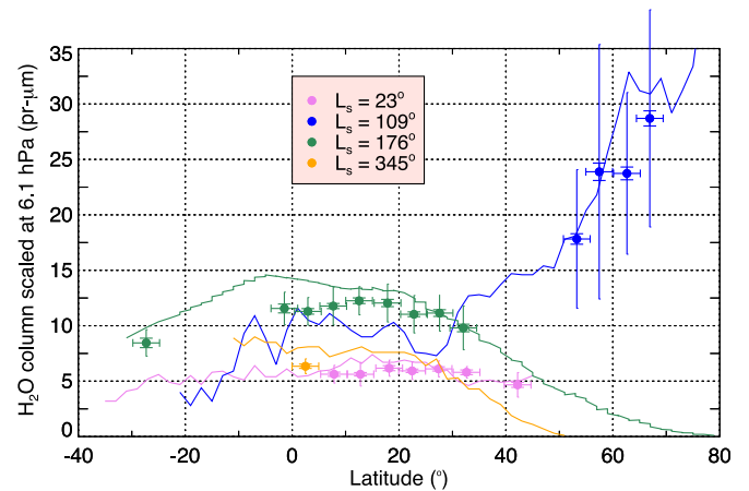
Fig. 22. Zonal averages of scaled H_2O column abundances obtained from a non-parametric NIR + TIR retrieval (see Fig. 18).
