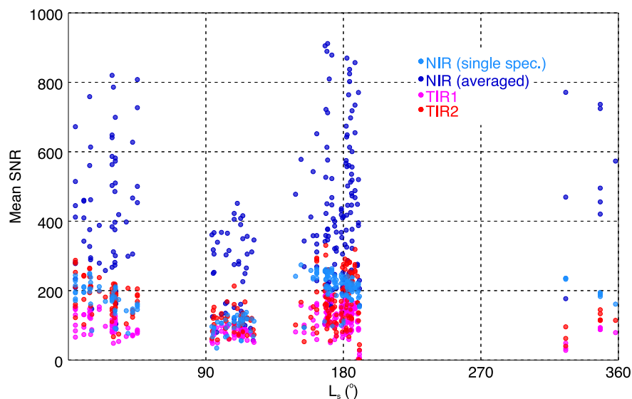
Fig. 2. SNR values for each spectral channel. NIR values obtained from individual spectrum are also shown.
