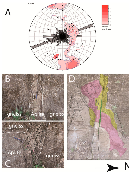
Figure 7. (A) Stereonets and rose diagrams of the REE bearing veins from the Gashirwe prospect (Low. Hem., Equal Area); (B) Aplite intruding gneiss, note the clustering of the post-aplite vertical dry jointing around the intrusive aplite dykes. Those dry fractures are almost parallel to the REE veins at the outcrop scale; (C) Similar pattern of “dry” fracturing within aplite which can enlarge as sill (bottom left). The gneiss foliation is disturbed by drag folding along the aplite and fractures; (D) REE veins (green) crosscutting aplite (pink) and pegmatite (yellow). The REE vein is not continuous and has a variable thickness.
