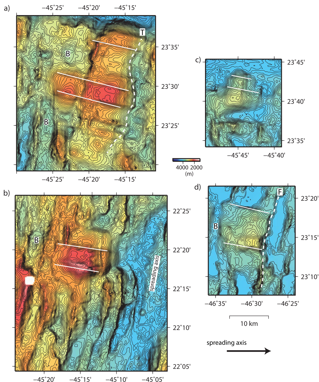
Figure 4. Examples of corrugated core complexes. Bathymetry data are contoured at 50 m intervals, and locations are shown in Figure 1. In each map the spreading axis lies to the east. Examples of corrugations are marked by continuous white lines. T and associated dashed white line: the termination of the detachment (where termination refers to the line of emergence of the fault from the ocean floor). F and associated dashed white line: a later fault that has cut across the detachment fault. B marks small basins (see text for details). (a) The Kane Megamullion area described by Dick et al. [2008]. (b) Area described by Dannowski et al. [2010]. South of the core complex is a group of small faults emerging from the median valley floor. (c, d) Sites some way off-axis. (d) A good termination fault.
