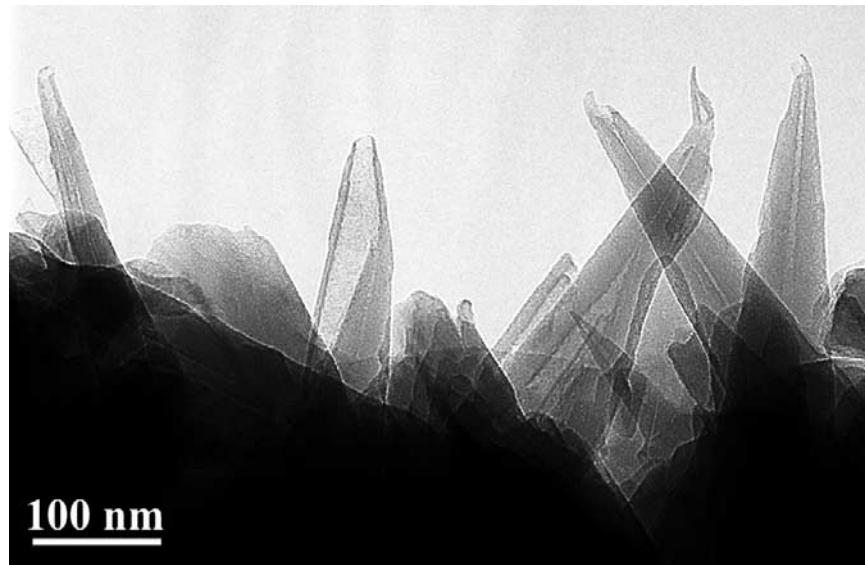
Figure 8. TEM image of conical serpentine tubes that dominantly fill a V1-type vein.
