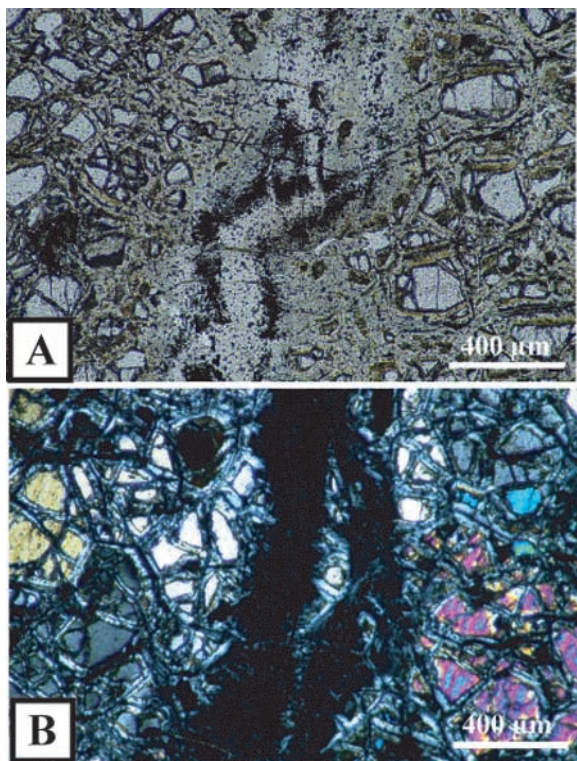
Figure 6. Serpentine vein of the V1 generation, marked by (a) oxide alignments on their walls when observed under polarized light and (b) a dark isotropic aspect under crossed-polarized light. They also present an alteration halo which is marked by the absence of relict olivine in close contact to the vein margins characterized by magnetite lineations.
