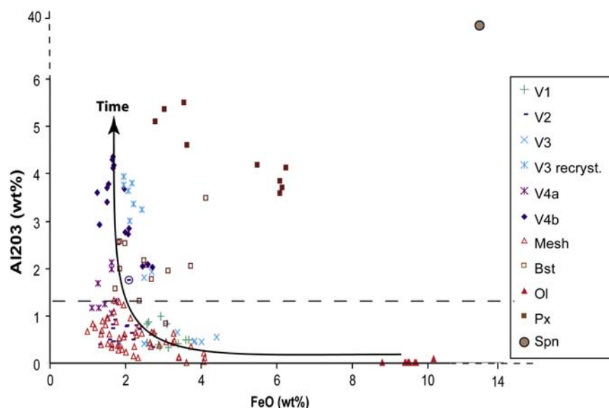
Figure 15. Comparison of the \text{Al}_2\text{O}_3 and \text{FeO} content of the different serpentine veins (V1 to V4) and some representatives compositions of relict minerals (Ol, olivine; Px, pyroxene; Spn, spinel) and pseudomorphic textures (Mesh; Bst, Bastite). The chemical evolution of the system with time (black arrow) is proposed on the basis of vein chronology.
