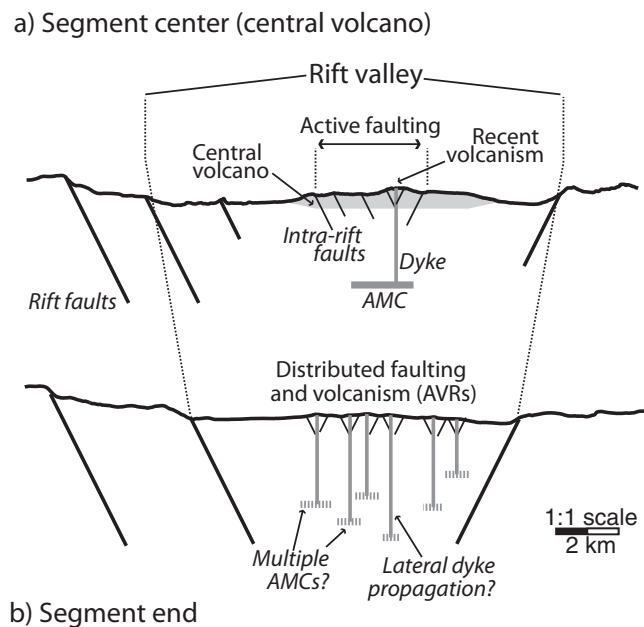
Figure 11. Cartoon showing differences in mode of volcanic emplacement and faulting between (a) the central volcano at the segment center and (b) the rift valley away from the central volcano. At the Lucky Strike volcano summit, recent volcanism and faulting are restricted to a well-defined axial graben (Figure 10). At the segment end, volcanism and deformation is distributed throughout the rift valley floor, and lacks a clear zone of preferential accretion. Volcanic ridges dominate volcanism, and can result from either lateral propagation of dikes from the central volcano and its underlying magma chamber, or from small, local magma chambers.
