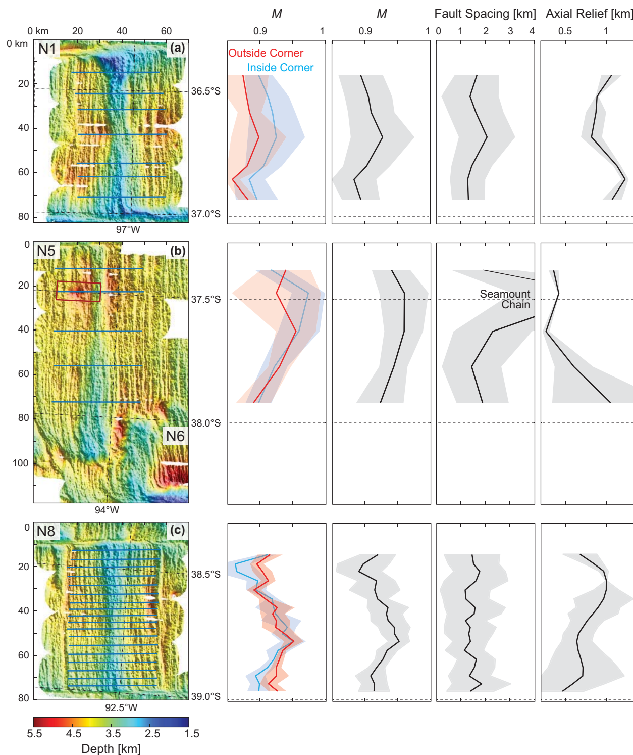
Figure 6. Chile Ridge bathymetry maps of studied segments (a) N1, (b) N5, (c) N8, (d) N9N, N9S, (e) N10, (f) V5, and (g) S5N, S5S, showing transects taken along spreading flow lines (blue lines) used to identify and measure faults, and to calculate axial relief. From left to right, the accompanying columns are: estimates of mean M (lines) and one standard deviation (colored backgrounds) for transect halves grouped by proximity to outside (red) and inside (blue) corners, estimates of total mean M , mean fault spacing, and axial relief (black lines) with one standard deviation (grey background) for whole transects.
