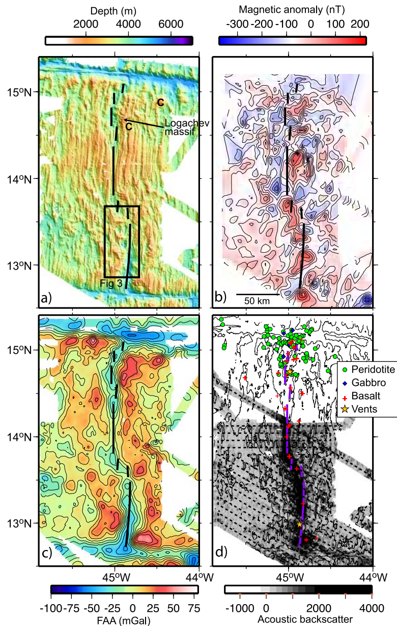
Figure 2. Data for the region between Fifteen Twenty and Marathon fracture zones from this study combined with those from Fujiwara et al. [2003] and Escartin and Cannat [1999]. Ridge axis is shown as a thick, segmented line. (a) Multibeam bathymetry data. The Logachev massif is marked. The area outlined is shown in greater detail in Figure 3. ‘C’: locations of core complexes identified by Fujiwara et al. [2003]. (b) Magnetic anomaly data. (c) Free air gravity data. (d) Acoustic backscatter plotted with dark indicating high amplitude returns and white low amplitude. Dashed lines: tracklines for the data collected by Smith et al. [2006]. Gold stars: hydrothermal vent fields hosted in ultramafic rocks. Green dots: locations where peridotites have been sampled. Blue diamonds: locations where gabbros have been sampled. Red plus: locations where basalts have been sampled.
