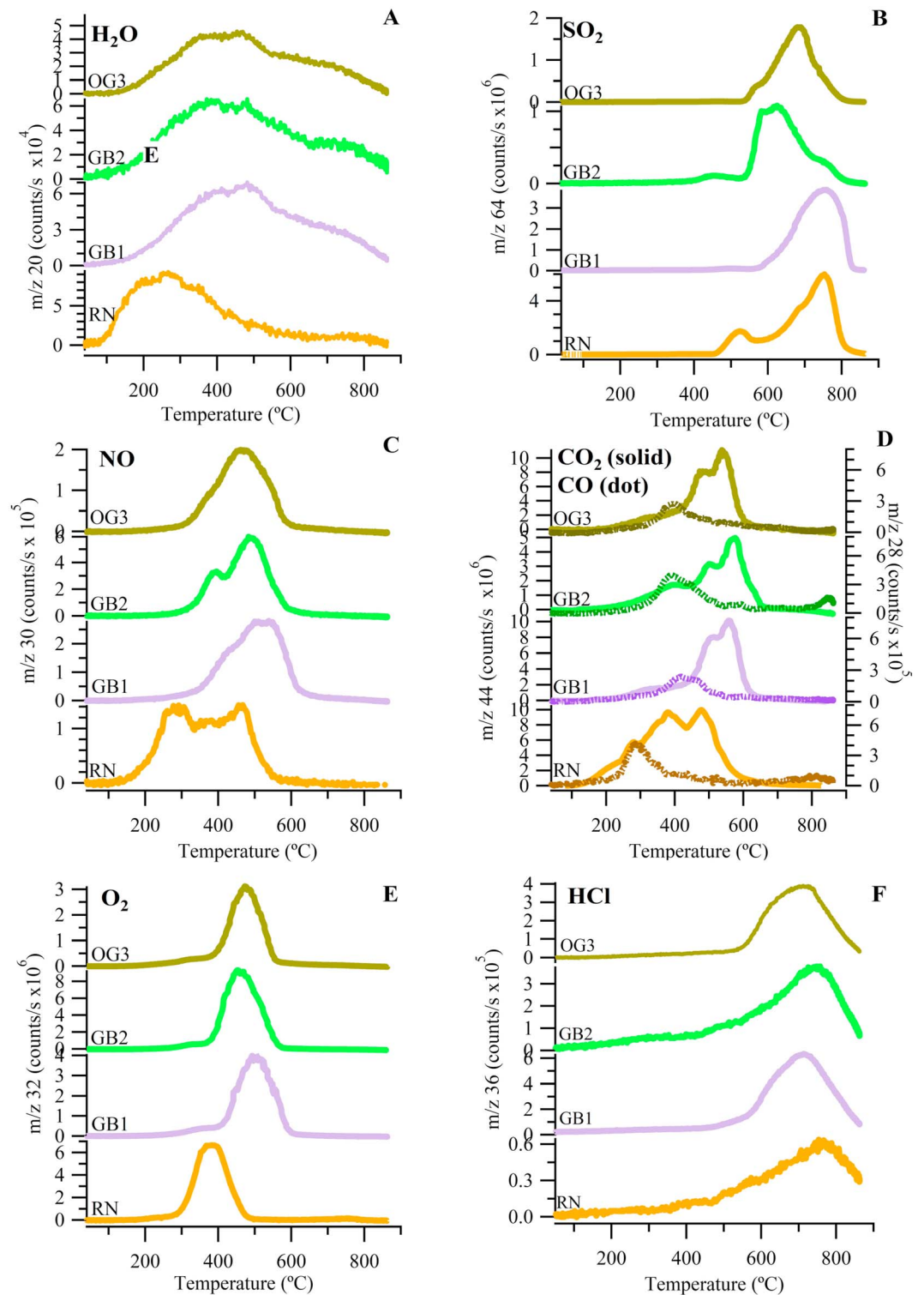
Figure 1. Evolved gas profiles for (a) H 2 O, (b) SO 2 , (c) NO, (d) CO and CO 2 , (e) O 2 , and (f) HCl. Y axes are scaled to optimize viewing for each species and vary accordingly. OG = Ogunquit Beach; GB = Gobabeb; RN = Rocknest.
