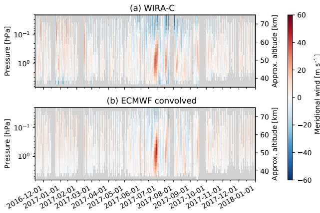
Figure 13. Same as Fig. 11 but for meridional wind. Time series of meridional wind speeds measured by WIRA-C (a) and ECMWF analysis data (b) between 14 November 2016 and 1 January 2018 for the altitude range of 35 to 75 km with a time resolution of 12 h (day and nighttime). The ECMWF data has been convolved with the averaging kernels of the retrieval in order to get the same spatial and temporal resolution for both datasets. Invalid data points are grayed out, resulting in different altitude ranges for different days. The few data gaps are due to a tropical cyclone and power outages.
