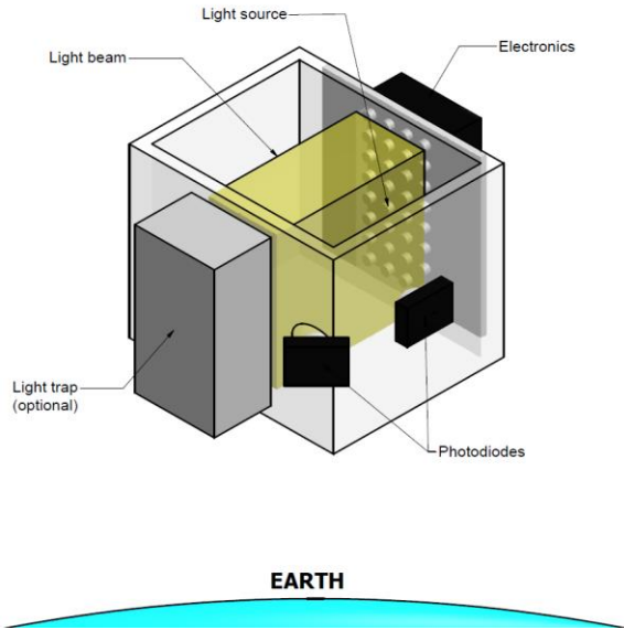
Figure 1: GRAAL concept.
