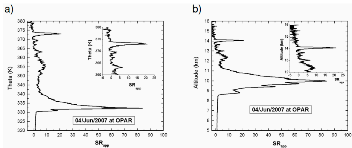
Figure 2. SR app profile observed by the lidar at Maïdo on 4 June 2007 at ~16h 50 UTC, according to the potential temperature (from ECWMF-ERA-Interim (Dataset of global atmospheric reanalysis stated as European Centre for Medium-Range Weather Forecasts Re—Analysis continued since 1979)) (a) and the corresponding altitudes (b).
