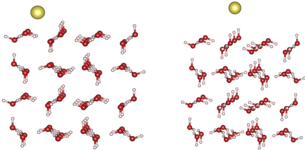
Figure 3. Apolar ice four bi-layers 1h unit cell used in calculations of adsorption energies on top of surface oxygens (left panel) and (right panel) hydrogen atoms ( 13.7 \times 13.7 \text{ \AA}^2 basal surface).
