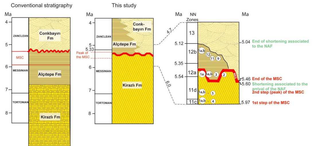
Figure 8. Controversial stratigraphy of the late Miocene-early Pliocene in the Canakkale region. Conventional stratigraphy (e.g., Görür et al., 1997; Sakiç et al., 1999; Yaltrık et al., 2000; Türkecan & Yurtsever, 2002; Çağatay et al., 2006) suggests gradual transition from the Kirazlı to the Alçıtepe Formations (Messinian age in this case) capped by the Zanclean Conkbayırı Formation. In this study (middle) angular and erosional (MES) unconformities between the Alçıtepe and Kirazlı Formations supported by calcareous nannoplankton biostratigraphy (Figure 7) explain well the stratigraphic setting. To the right: Detail corresponding to the top of the Kirazlı Formation and base of the Alçıtepe Formation at sites such as Sonok and Nuriyemut Beach (see Figure 5), with location of dated sections. MES = Messinian erosional surface; NAF = North Anatolian Fault; MSC = Messinian Salinity Crisis.
