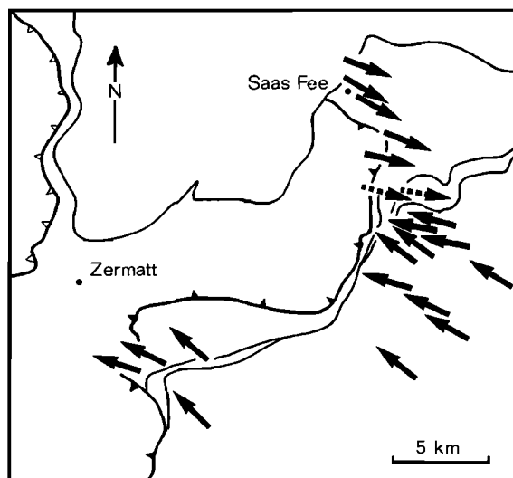
Fig. 16. Shear senses determined from sample and outcrop study at regional scale: arrows represent hangingwall movements; less well constrained shear senses are dashed.
