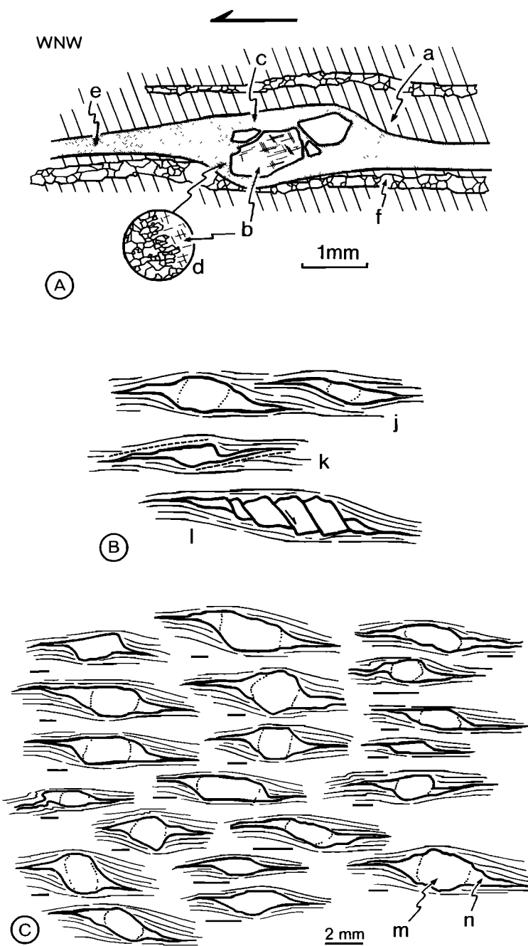
Fig. 11. Characters of feldspar deformation in gneisses (west vergent shear sense). (A) Microstructures: (a) matrix, (b) porphyroblast core, (c) mantle of small recrystallized grains, (d) detail of core mantle boundary, feldspar recrystallized at the core rim, (e) tail resulting from mantle deformation, (f) quartz ribbon. (B) Typical shear criteria: (j) sigmoidal porphyroblast, (k) "tilted" porphyroblast with edges and tails parallel to incipient shear planes (dashed), (l) antithetic slip on fractures within Feldspar. (C) Example of feldspar deformation in shear zone (shear sense determined independently by sigmoidal deflection of macroscopic foliation); (m) porphyroblast core, (n) tail.
