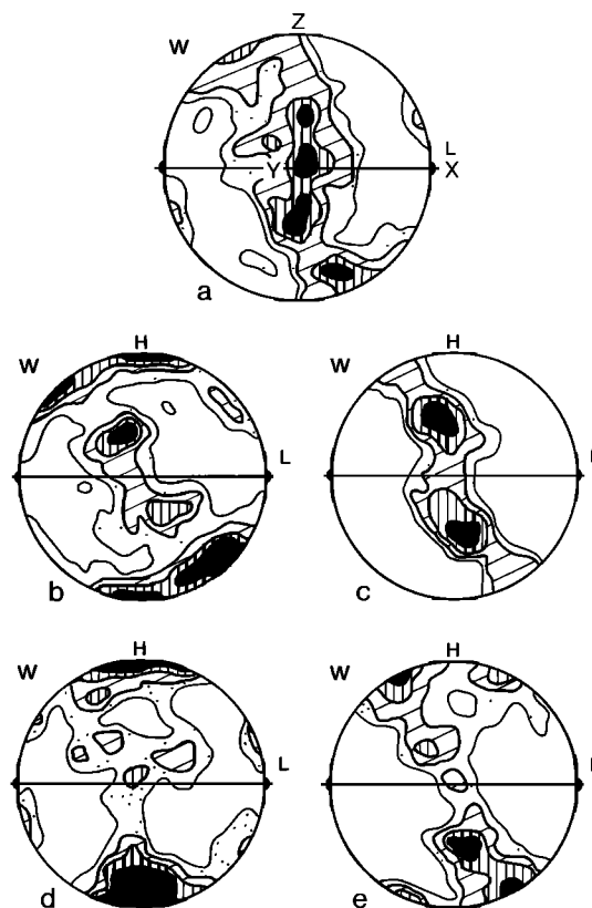
Fig. 10. Quartz c axis fabrics in gneisses and mylonites. (a) central part of shear zone, sample ZA2, W Mattmark shore lake, 340 c axes, contours 1; 1,5; 2,5; 3,5%, maxi 5,5%. (b) orthogneisses, sample SF55, E Mattmark shore lake, 180 c axes, 1; 2; 3; 4%, maxi 5%. (c) mylonite, sample SF62, W Mattmark shore lake, 180 c axes, 1; 2; 4; 8%, maxi 18%. (d) thin ultramylonite crosscutting outer shear zone foliation, sample SF42, MR Hütte, 200 c axes, 1; 2; 3; 4%, maxi 6%. Lower hemisphere Schmidt diagrams (as in Figure 12). Measurements made on Universal stage are presented in XZ plane; L is lineation and X axis.
