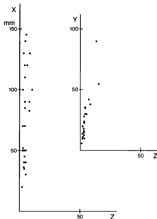
Fig. 13. Pebble shape fabric in conglomerates from Gornergrat. X \geq Y \geq Z are principal axes of elongated pebbles ( 10 \leq X/Z \leq 80 ; 0.5 \leq K \leq 1 ).
