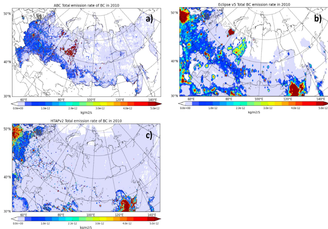
Figure 2. Comparison of different Eurasian black carbon (BC) emission inventories from (a) the Arctic BC (ABC) data set (Huang et al., 2015), (b) Evaluating the Climate and Air Quality Impacts of Short-Lived Pollutants version 5 (ECLIPSEv5; Stohl et al., 2015), and (c) Hemispheric Transport of Air Pollution version 2 (HTAPv2; Janssens-Maenhout et al., 2015) for the year 2010, from Sergent (2017). Note not all inventories cover the entire Arctic, hence the focus on Eurasia.
