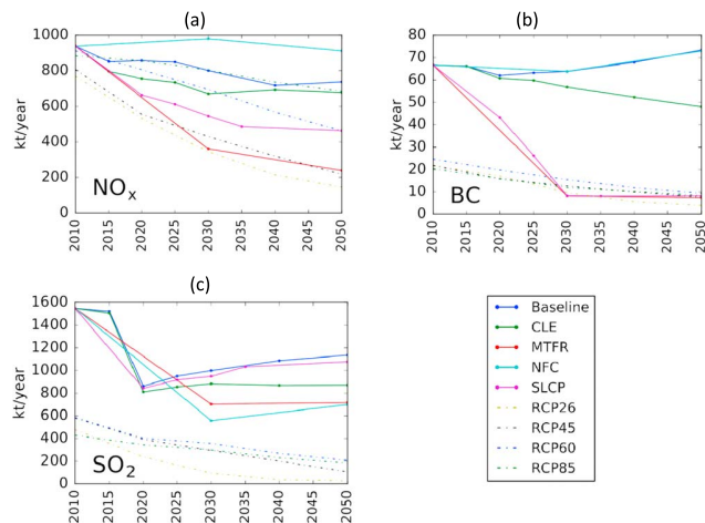
Figure 3. Future emission scenarios. Scenarios are for (a) NO x , (b) BC, and (c) SO 2 , based on the Evaluating the Climate and Air Quality Impacts of Short-Lived Pollutants (ECLIPSE) v5a and Representative Concentration Pathway (RCP) emissions data sets for regions north of 60°N (Stohl et al., 2015; van Vuuren et al., 2011). The colored lines show different future scenarios. Solid: ECLIPSE scenarios with baseline, current legislation (CLE), maximum technologically feasible reduction (MTRF), no further control (NFC), and short-lived climate-forcing pollutants (SLCP) mitigation. Dotted: RCP scenarios. Note that the ECLIPSE NFC scenario is from the v5 data set (not v5a). See main text for description of scenarios.
