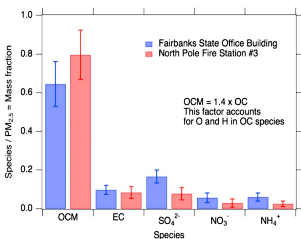
Figure 5. Fractional mass composition of PM 2.5 in Fairbanks and North Pole, Alaska. The species shown are: Organic carbonaceous materials (OCM), which is calculated by multiplying organic carbon (OC) by 1.4 to account for the mass of O and H in these species. Elemental carbon (EC) and inorganic ions (SO 4 2- , NO 3 - , and NH 4 + ) are also shown. Data represent the average from three winter seasons between November 2011 and February 2014.
