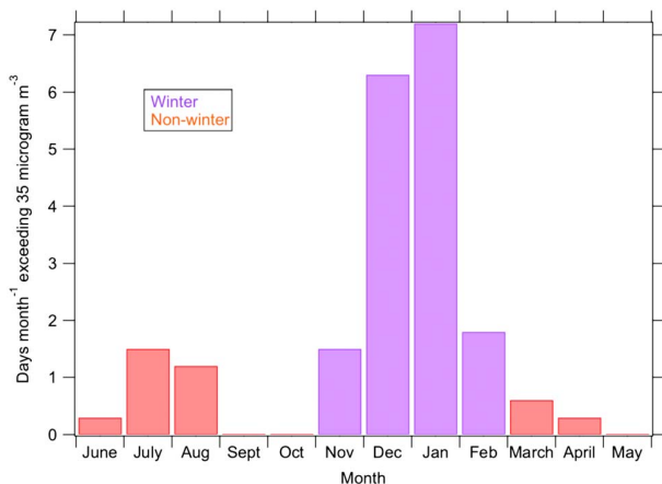
Figure 4. Air quality exceedances in Fairbanks, Alaska, United States. Mean number of measurement days in exceedance of the Environmental Protection Agency PM 2.5 standard (35 µg/m 3 ) per month 2006–2014 (from Environmental Protection Agency air quality database). Measurements are made only every third day, hence a factor of three has been applied to the data shown in this figure.
