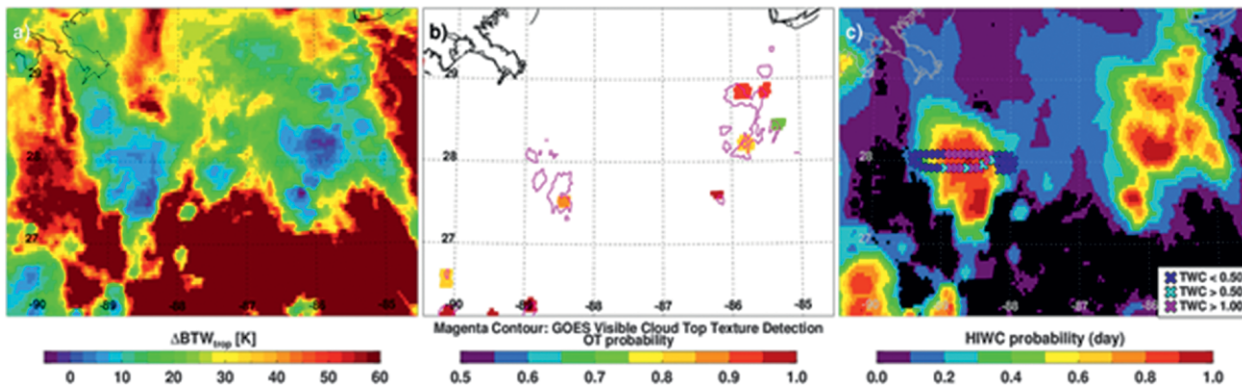
FIG. 2. (a) Tropopause-relative GOES-14 IR brightness temperature (GOES minus tropopause). Cool colors indicate cloud tops near to or above the tropopause. (b) GOES IR overshooting top detection probability (color shading; values >0.7 shown) and visible texture detection (magenta contours). (c) NASA LaRC PHIWC overlaid with a 10-min segment of TWC collected by the NASA DC-8 aircraft during the 2015 Fort Lauderdale flight campaign. Aircraft positions are colored by the observed TWC, showing a sharp transition when the aircraft entered a region of high PHIWC ( >0.6 ) driven by cloud tops near the tropopause and close proximity to overshooting cloud tops.
