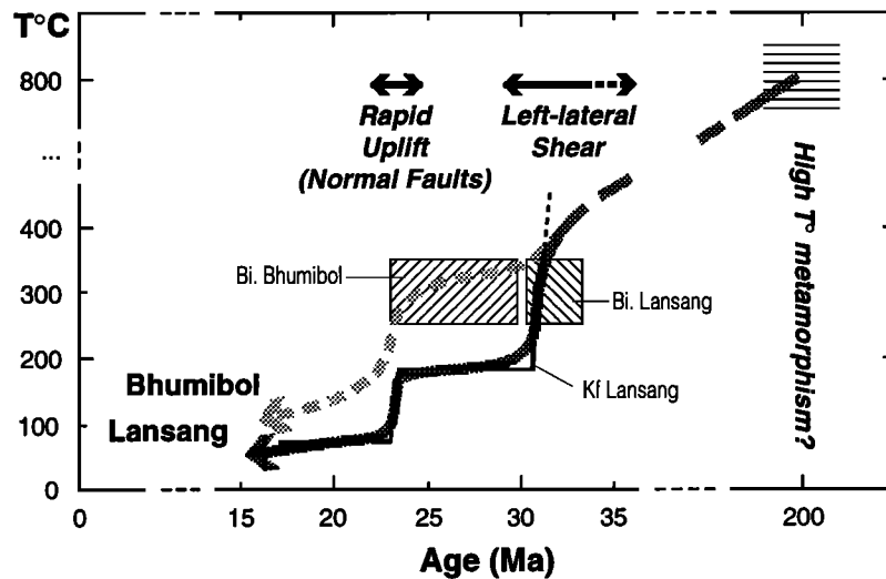
Figure 12. Time-temperature paths for Lansang mylonitic gneisses (dark gray) and for border of Lincang-Chiang Mai belt between Bhumibol dam and Lansang gneisses (light gray). Temperatures and ages deduced from biotite results (boxes with diagonal hatching) and K-feldspar modeling (solid line). Temperature conditions of high-temperature metamorphism from Martelet [1994]. Age of this metamorphism ( \approx 200 Ma according to Ahrendt et al. [1993]) is poorly constrained.
