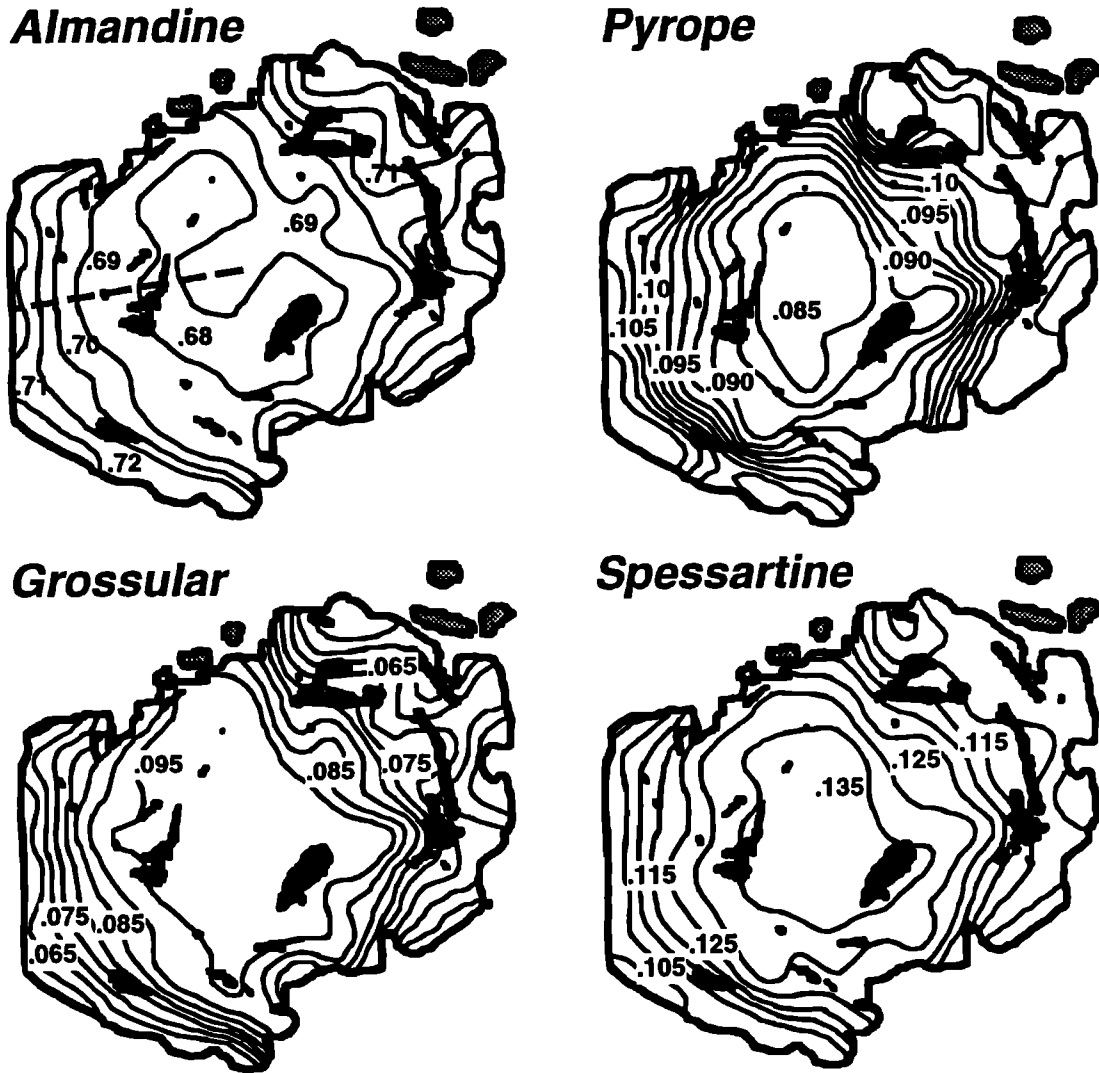
Fig. 11. Compositional zoning in garnet displaying concentric zonation truncated by areas of garnet resorption. The zoning profile in Figure 12 was collected along the trace shown by the dashed line.
