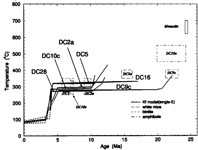
Fig. 23. Summary of all thermal history results from the Diancang Shan samples. Monazite U/Pb result from Liu et al. [1992]; all other results from this study. The Kf cooling histories are those assuming a single activation energy (single-E).
