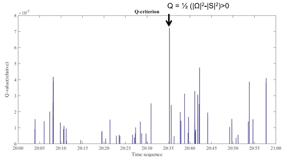
Figure 13. The Q -criterion values ( Q = \frac{1}{2} (\|\boldsymbol{\Omega}\|^2 - \|\mathbf{S}\|^2) ) versus time are measured for the identified 105 vortex core line cases. All Q -criterion values are positive, which also indicates the existence of vortices. The black arrow indicates one of the steepest waves around the time 20:35.
