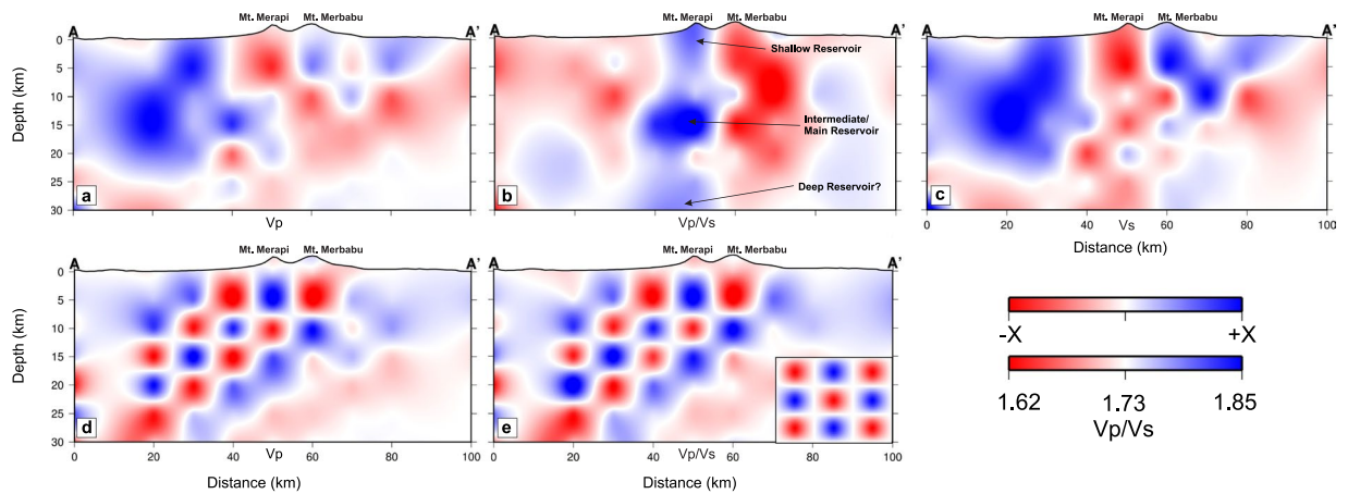
Figure 3. South-North vertical sections across Merapi and Merbabu. (a) V_p , (b) V_p/V_s , (c) V_s , (d) checkerboard recovery for V_p , and (e) same as (d) but for V_p/V_s . The input pattern of the checkerboard test is shown in the inset in (e) with input perturbations of X = 10\% for both V_p and V_p/V_s as in Fig. 2. V_p and V_s are plotted as perturbations with X = 12\% relative to the 1D model based on Koulakov et al. 18 and X = 5\% for the checkerboard recovery for V_p and V_p/V_s ; while V_p/V_s is plotted as absolute values.
