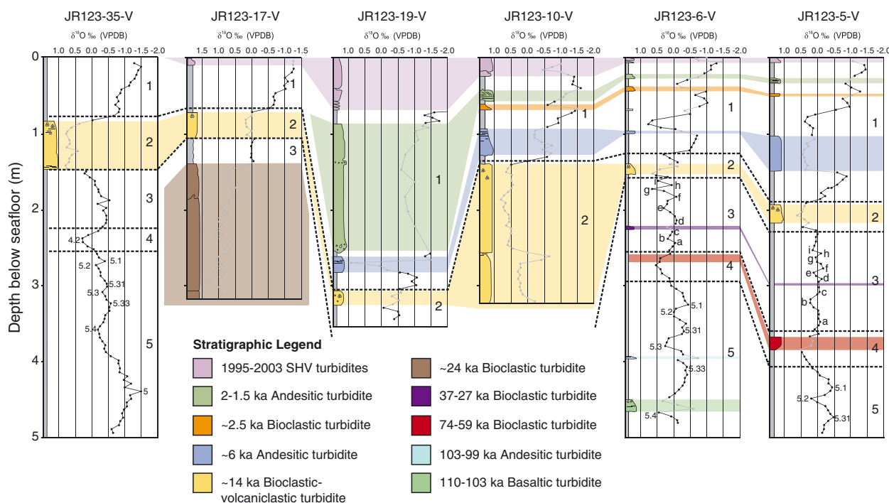
Figure 2. Oxygen isotope ( \delta^{18}\text{O} ) stratigraphy measured for cores 35-V, 17-V, 19-V, 10-V, 6-V, and 5-V (see Figure 1 for locations). Each core is presented with marine isotope stages (1 to 5) labeled on the right-hand side of each panel. Samples taken from within the flow or fallout units are shaded gray. Analysis of the stable isotope record in the text avoids this data.
