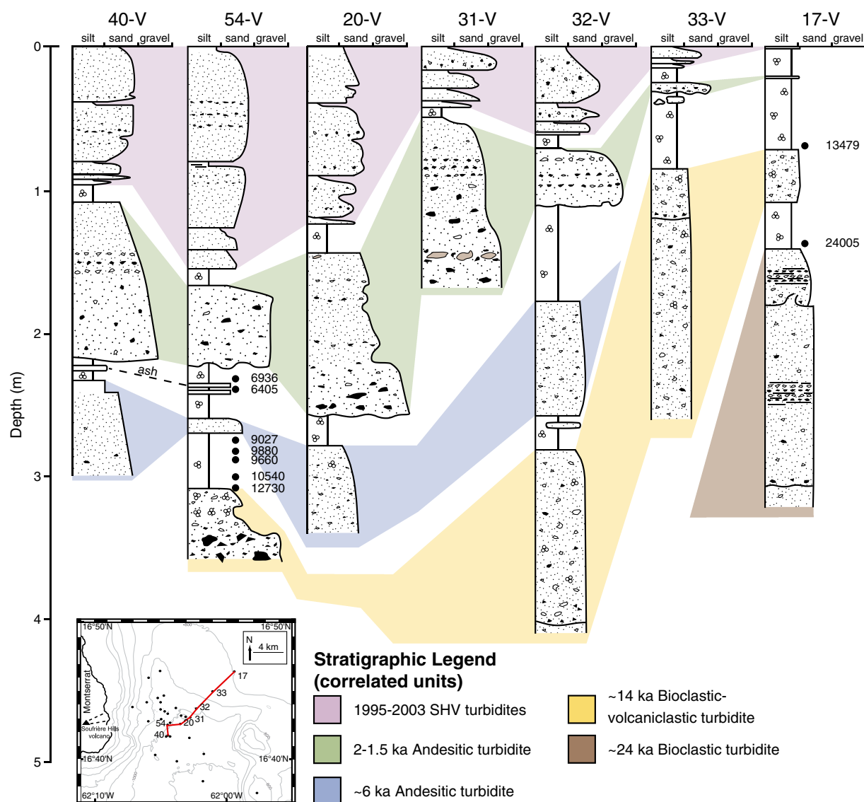
Figure 4. Correlated stratigraphic logs showing a transect through the northern Bouillante-Montserrat graben, perpendicular to the longitudinal graben axis. Radiocarbon dates are provided in “years before present” with 2\sigma standard deviation; full details are in Table 1. Inset map shows the core numbers and locations.
