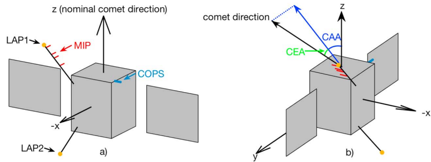
Figure 1. (a) Geometrical configuration of the LAP (yellow), MIP (red), and COPS (light blue) sensors. (b) Angles used to describe the spacecraft attitude.
