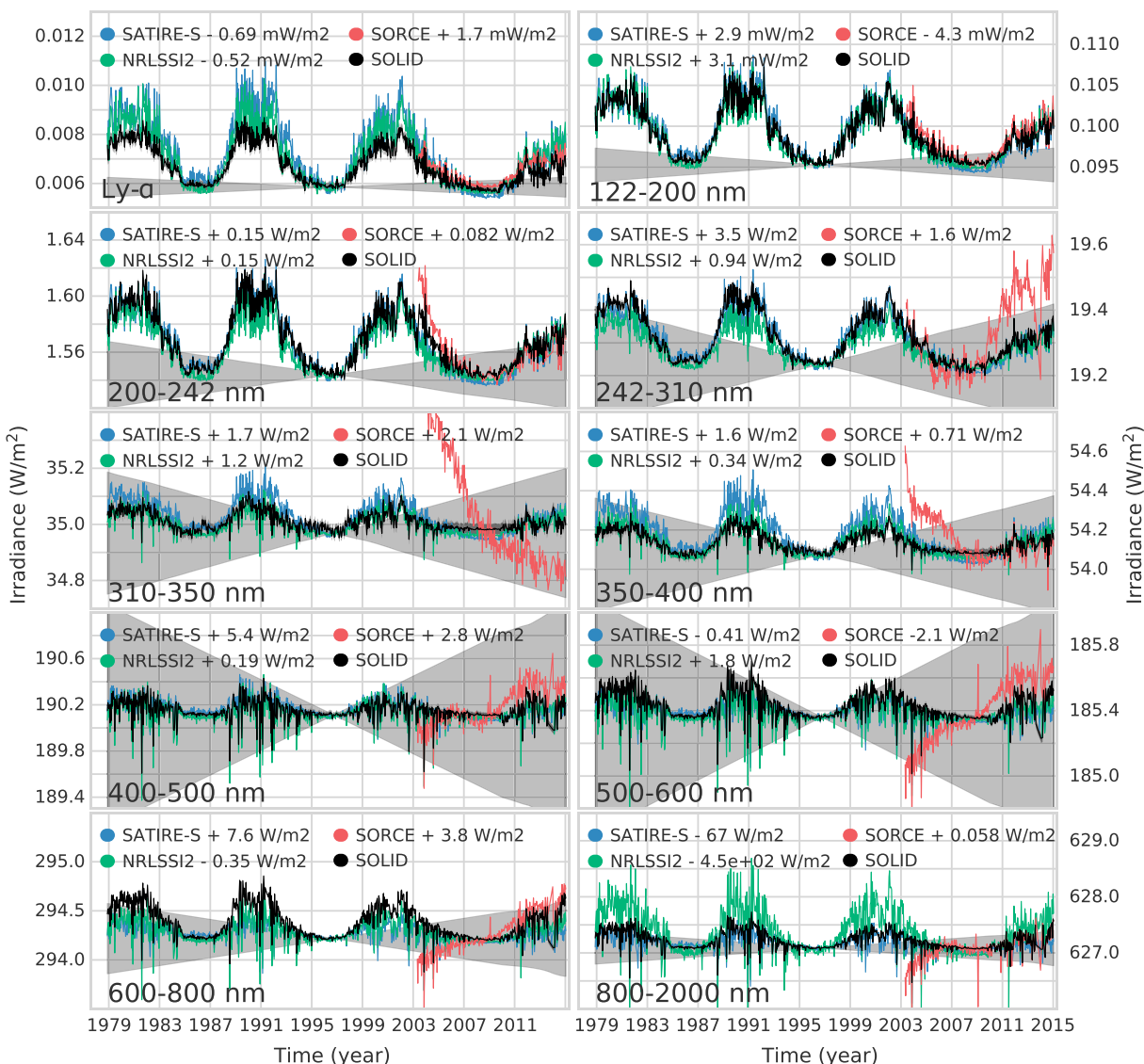
Figure 7. Same as Figure 3 but for the final SOLID composite.
