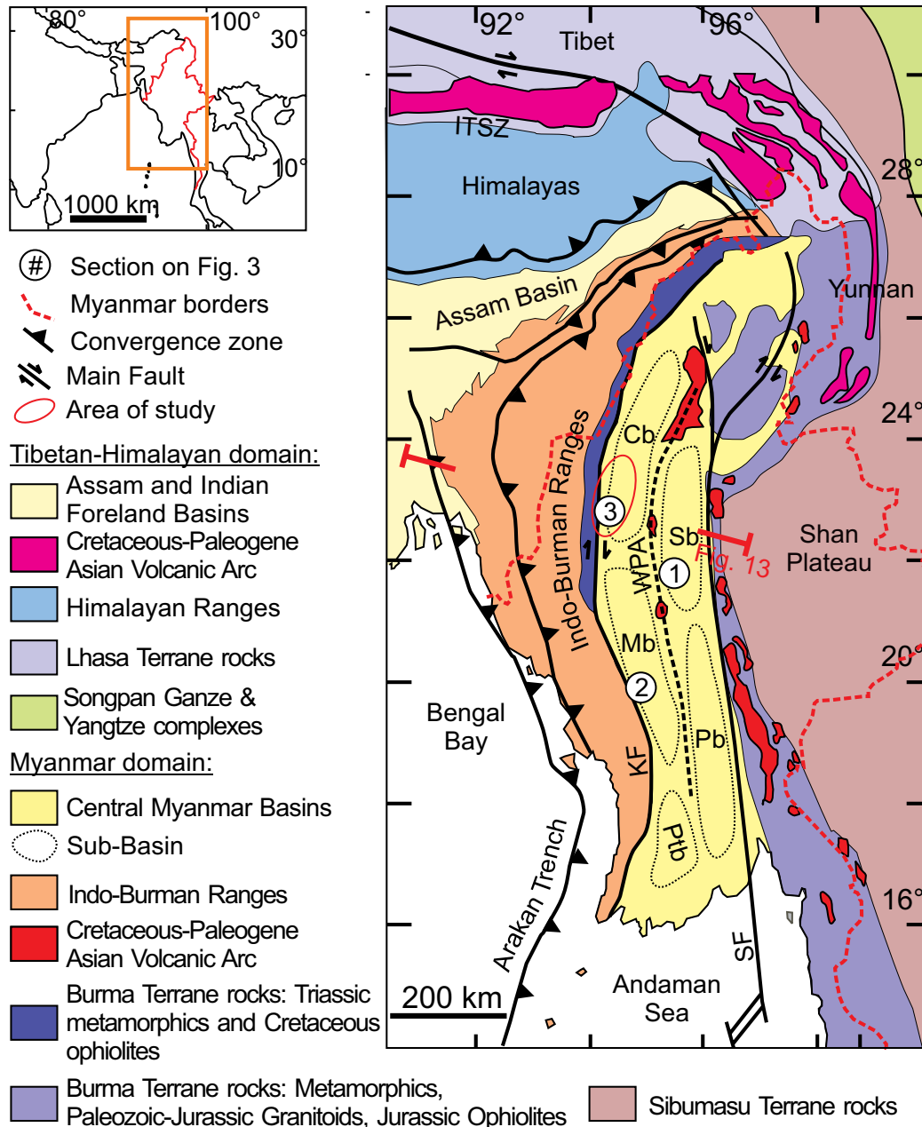
Figure 2. Schematic map of the eastern Himalayan syntaxis and central Myanmar, with the main geological units, after Licht et al. (2013) ; boundaries between Tibetan and SE Asian terranes are not precisely drawn because they are poorly known. The approximate axis of the Wuntho-Popa Andean arc (WPA) is shown by a thick, dashed black line. The sub-basins of central Myanmar are indicated with thin, dashed black lines: the Chindwin, Minbu, and Patheingyi basins (Cb, Mb, and Pb) in the forearc, the Shwethary and Pegu basins (Sb and Pb) in the backarc. ITSZ—Indus-Tsangpo Suture Zone; SF—Sagaing Fault; KF—Kabaw Fault. Numbers in circles indicate the location of the synthetic logs in Figure 3 , and the red line indicates the location of the cross section in Figure 13 . Area of study is shown by a red circle. Symbol (3) sits at the location of our composite section.
