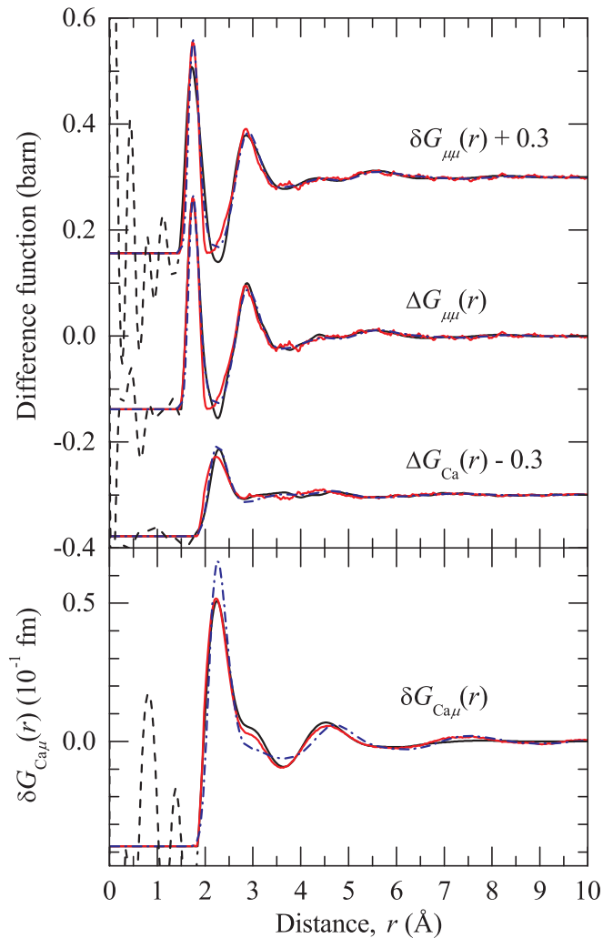
FIG. 5. The real-space difference functions \delta G_{\mu\mu}(r) , \Delta G_{\mu\mu}(r) , \Delta G_{Ca}(r) , and \delta G_{Ca\mu}(r) for liquid Ca_3Al_2O_6 (solid dark-black curves), as obtained by Fourier transforming the corresponding reciprocal-space functions given in Fig. 4. The broken black curves show the extent of the unphysical low- r features, the chained blue curves show the functions calculated from the partial pair distribution functions generated directly from the MD simulations, and the solid light-red curves are the results of the RMC structural refinement. For clarity, the results are displaced vertically.
