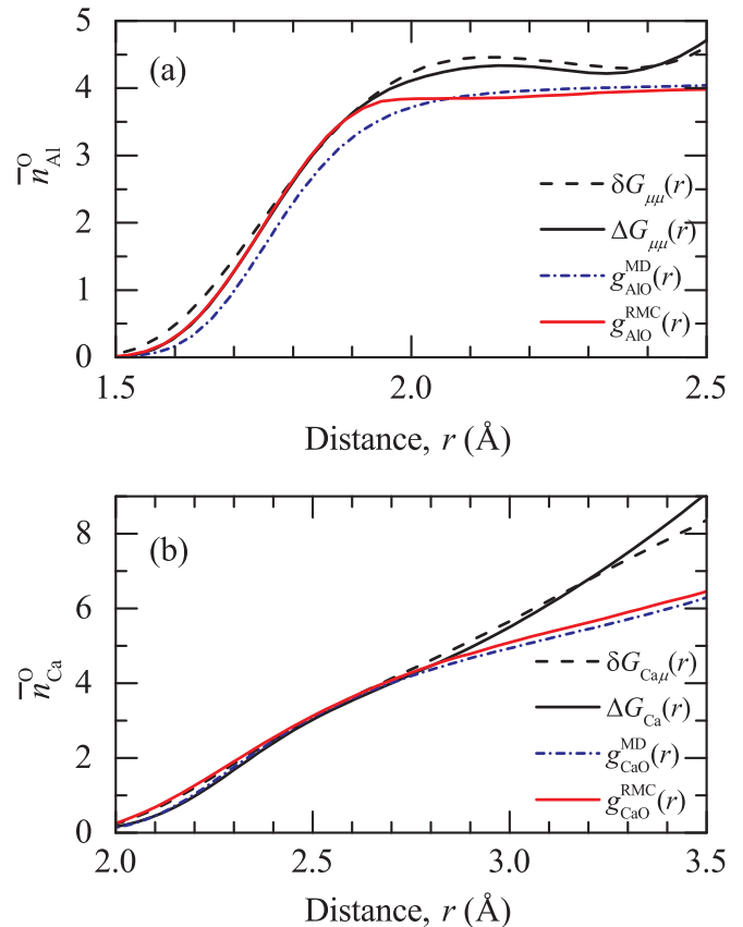
FIG. 6. Running coordination numbers (a) \bar{n}_{Al}^O and (b) \bar{n}_{Ca}^O determined from the measured difference functions and MD and RMC partial pair distribution functions indicated in the legend. The deviation at higher- r values is due to the contributions from correlations of other atomic pairs in the measured difference functions.
