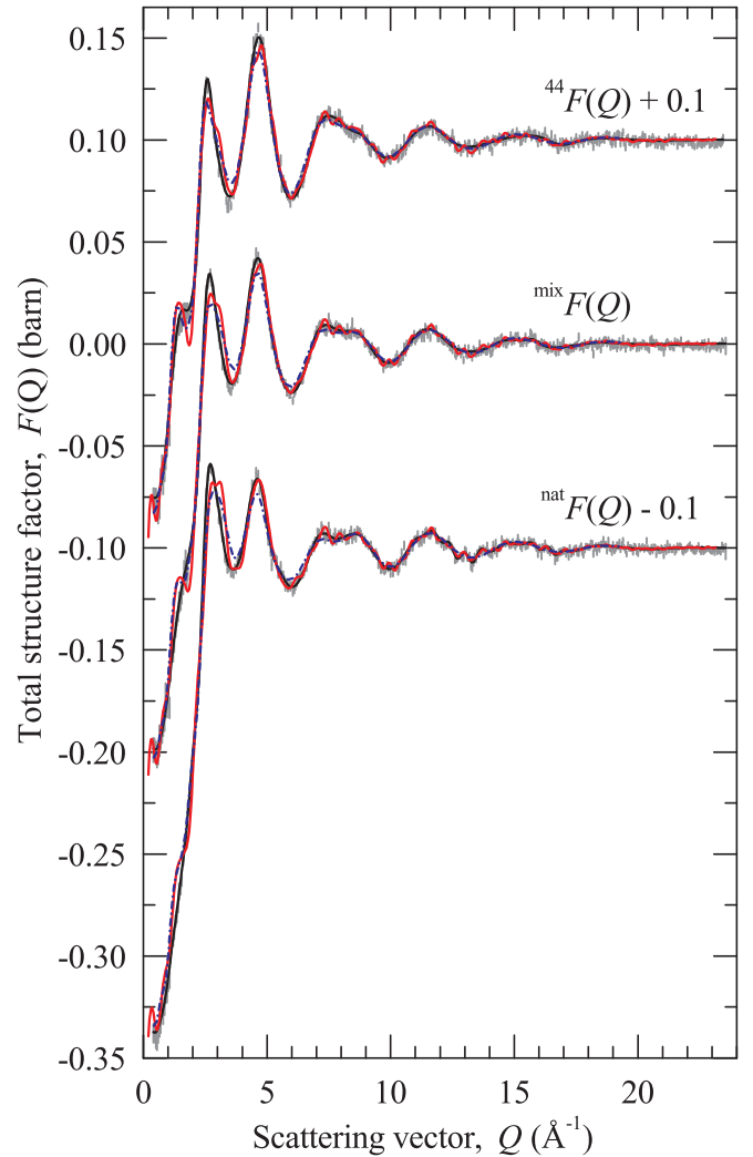
FIG. 1. Total structure factors ^{44}F(Q) , ^{\text{mix}}F(Q) , and ^{\text{nat}}F(Q) measured by neutron diffraction for the aerodynamically levitated \text{Ca}_3\text{Al}_2\text{O}_6 liquids at 2073(30) K. The vertical bars show the statistical errors and the solid dark-black curves are the Fourier back-transforms of the corresponding total pair distribution G(r) functions shown in Fig. 3 after the region below the first interatomic distance was set to the theoretical r = 0 limit. The chained blue curves show the functions generated from the MD simulations and the solid light-red curves show the results of the RMC structural refinement. For clarity, the results are displaced vertically.
