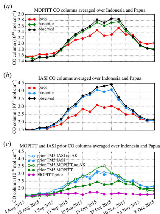
Figure 2. Measured weekly averaged (a) MOPITT and (b) IASI CO columns over Indonesia and Papua, and modelled by the prior GFAS and posterior IASI and MOPITT inversions. (c) Prior TM5 columns for IASI and MOPITT before and after applying the averaging kernel. The MOPITT retrieval prior, originating from a CAM-chem simulation with climatological biomass burning emissions, is also shown.
