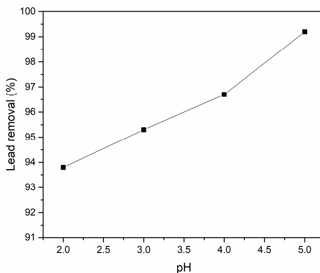
Figure 4. Effect of the solution pH on the removal of \text{Pb}^{2+} ions by N-HAp powders.
