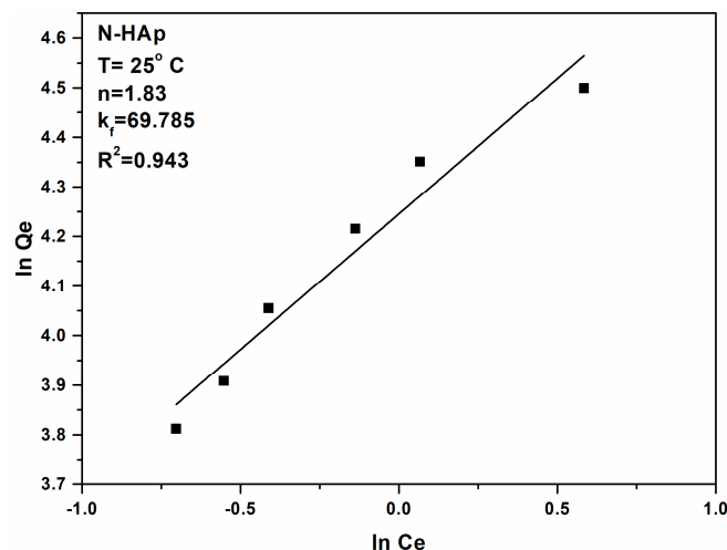
Figure 7. Freundlich linearized fits for the adsorption of lead ions on N-HAp.
